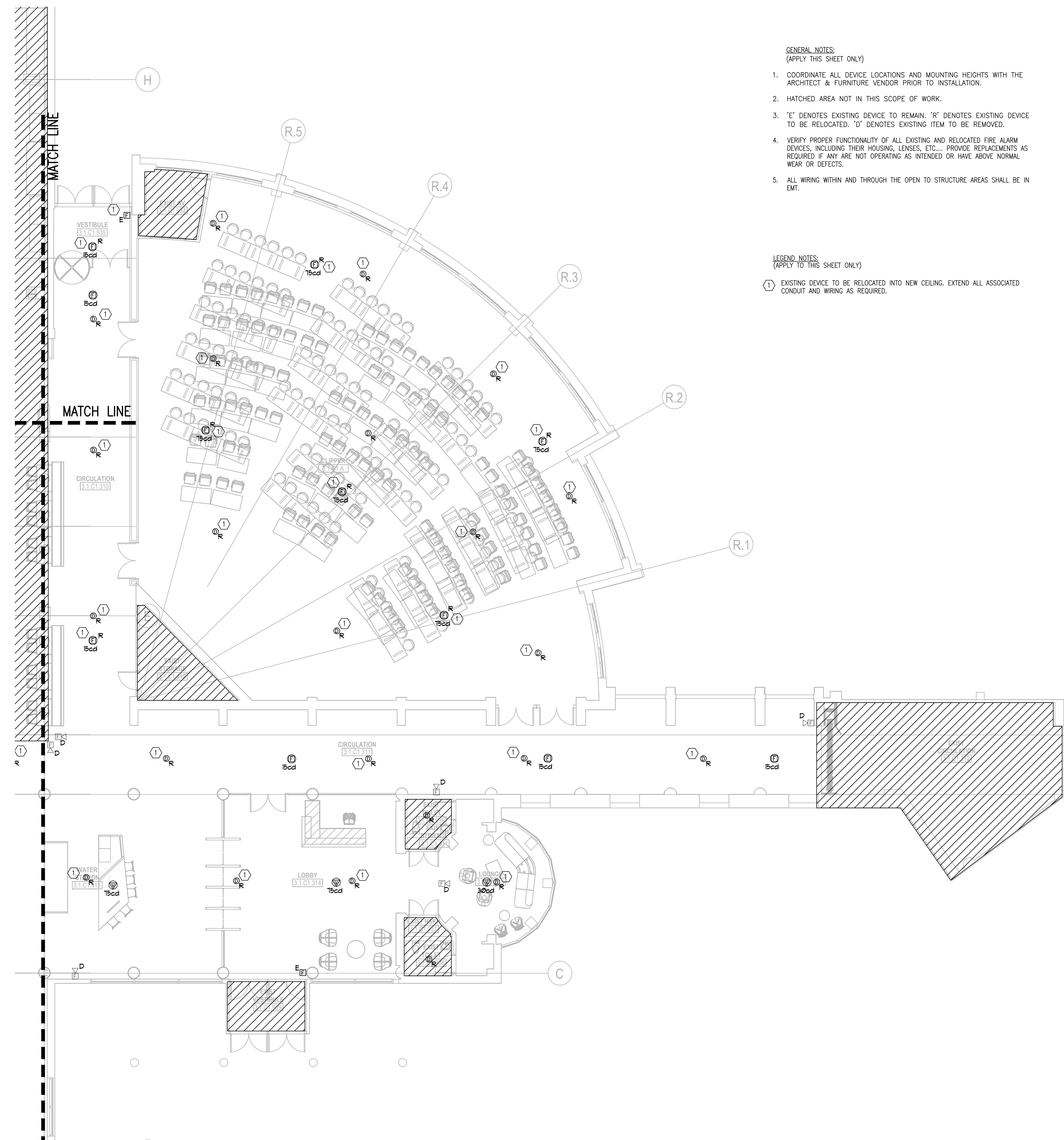
① 1ST FLOOR PLAN (AREA C1) - FIRE ALARM E2.301C.1 1/8"=1'-0"
