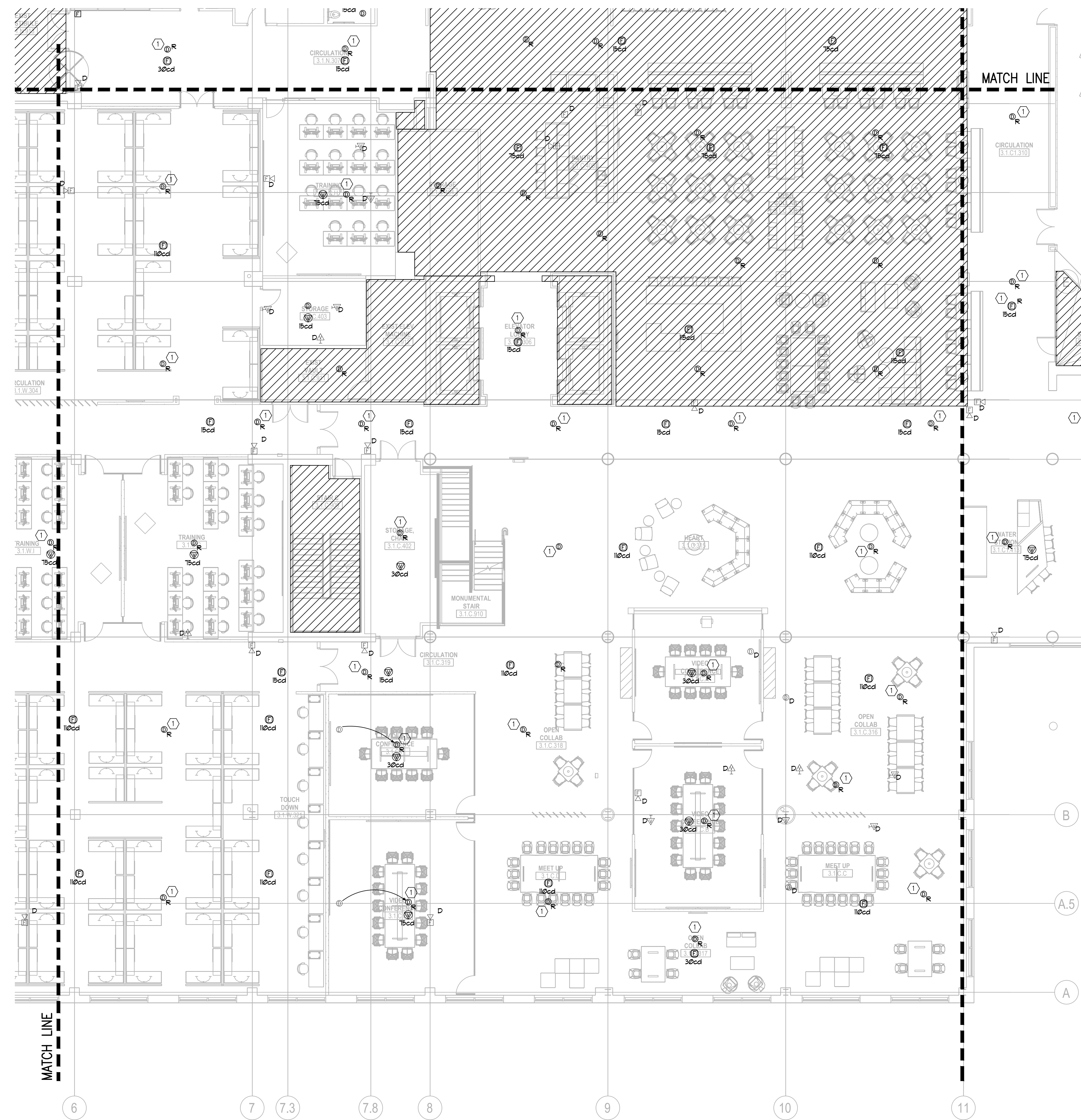
1 1ST FLOOR PLAN (AREA C) – FIRE ALARM E2.301C 1/8"=1'-0"
