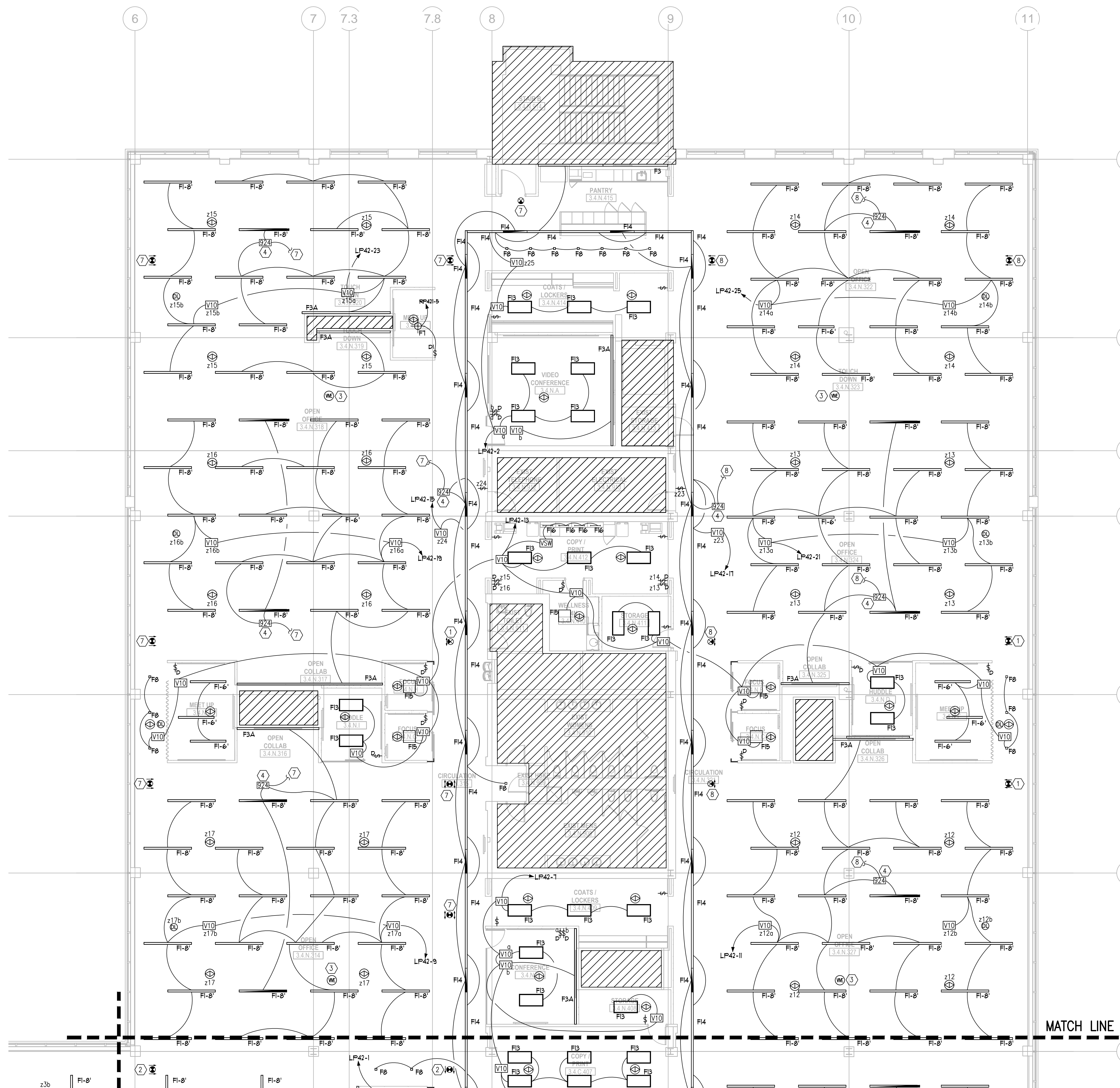
1 4TH FLOOR PLAN (AREA N) - LIGHTING E2.204N 1/8"=1'-0"
