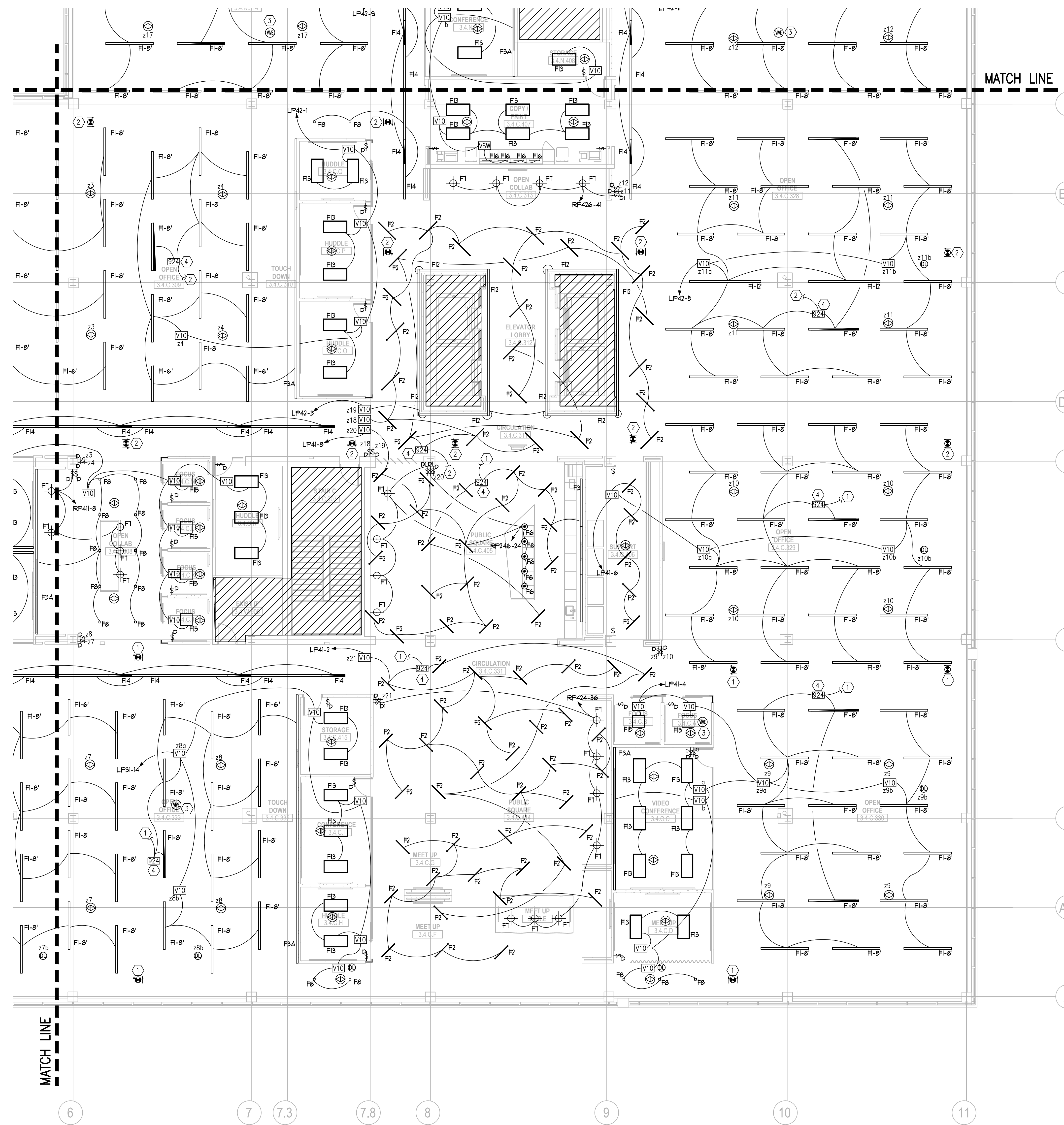
4TH FLOOR PLAN (AREA C) - LIGHTING 22.204C 1/8"=1'-0"
