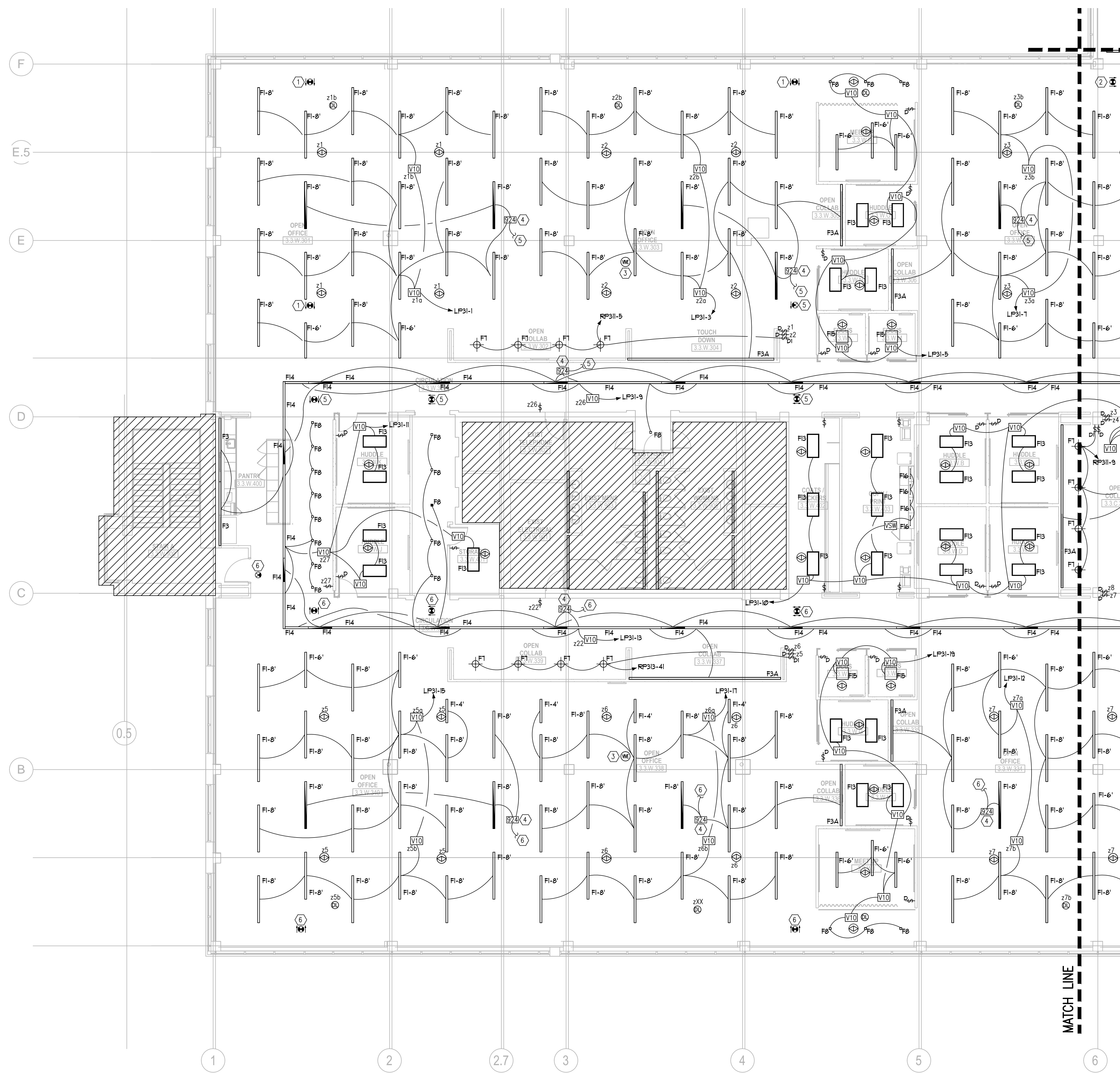
1 3RD FLOOR PLAN (AREA W) - LIGHTING E3.203W 1/8" = 1'-0"
