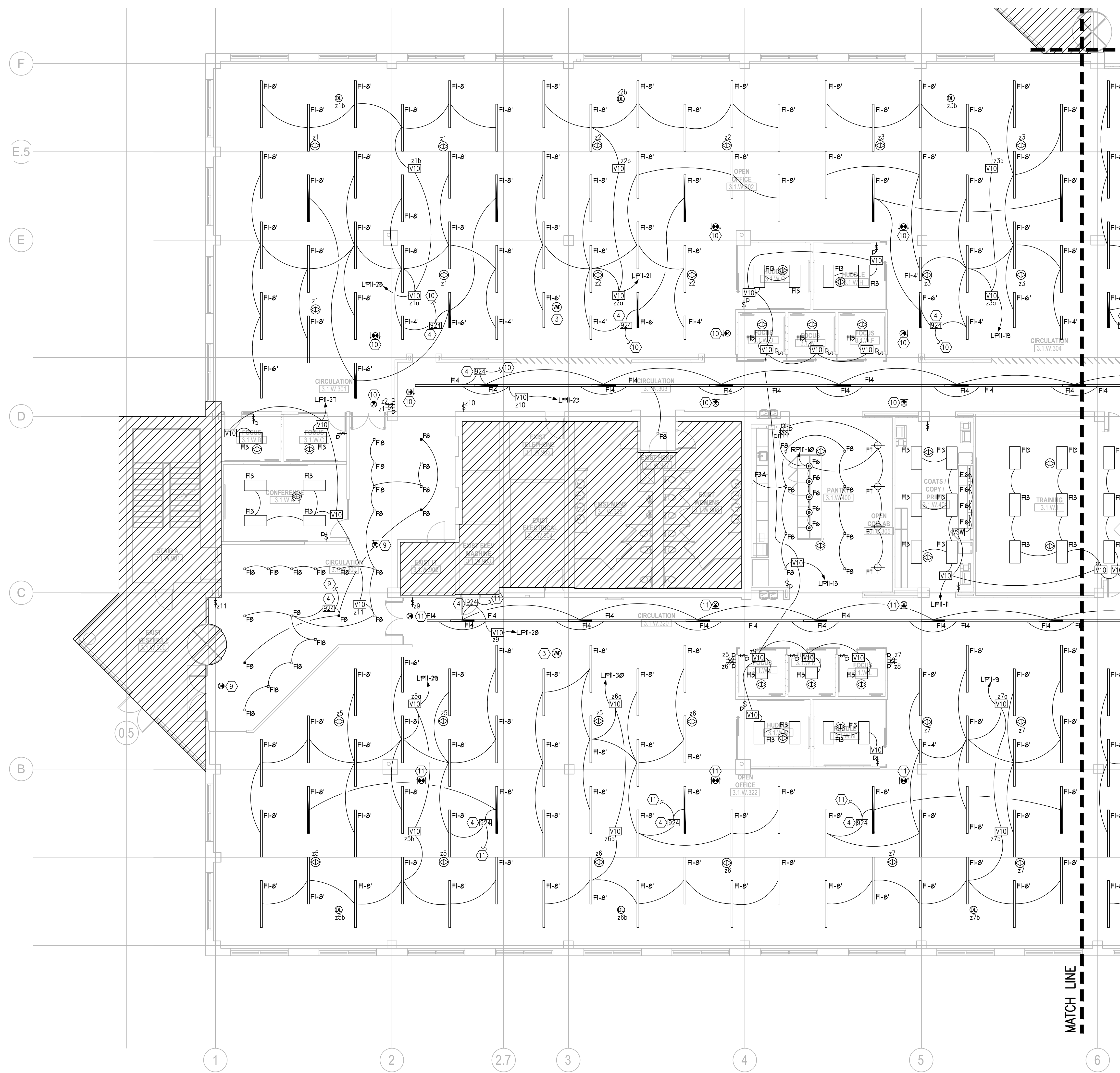
1 1ST FLOOR PLAN (AREA W) - LIGHTING 2.2.2016 1/8"=1'-0"
