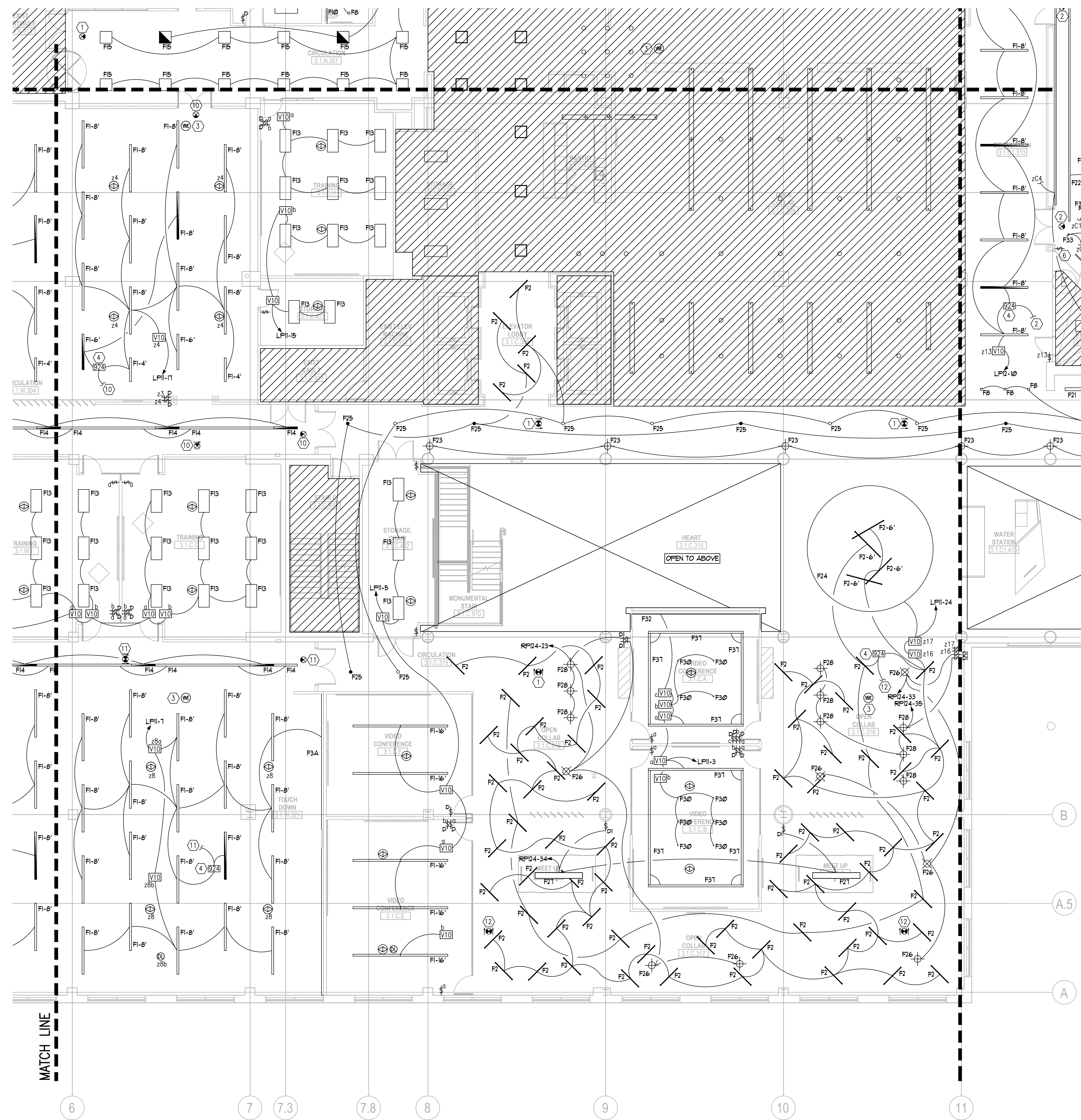
1 1ST FLOOR PLAN (AREA C) - LIGHTING 2.2010C 1/8" = 1'-0"
