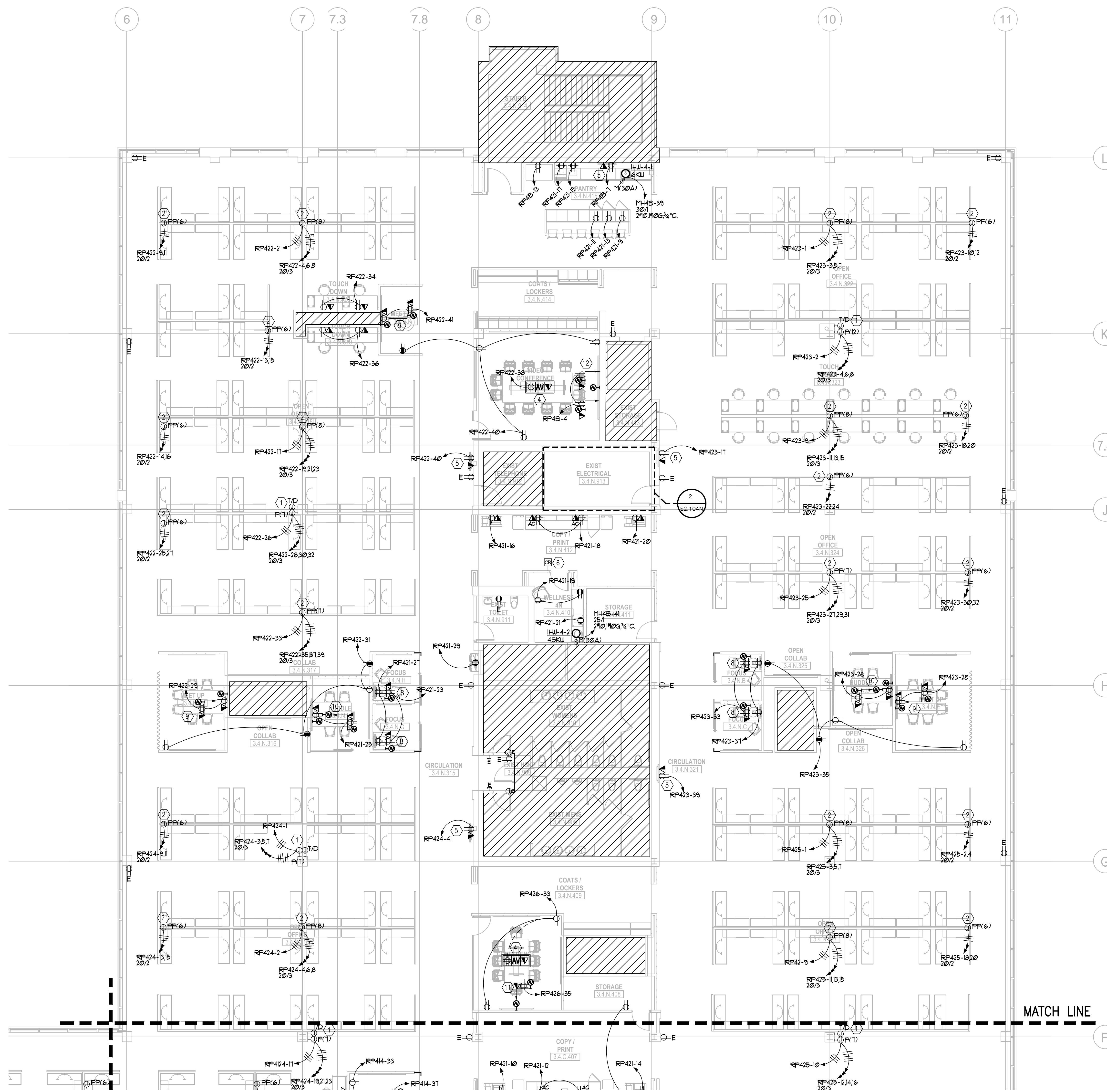
1 4TH FLOOR PLAN (AREA N) - ELECTRICAL 1/8" = 1'-0"
