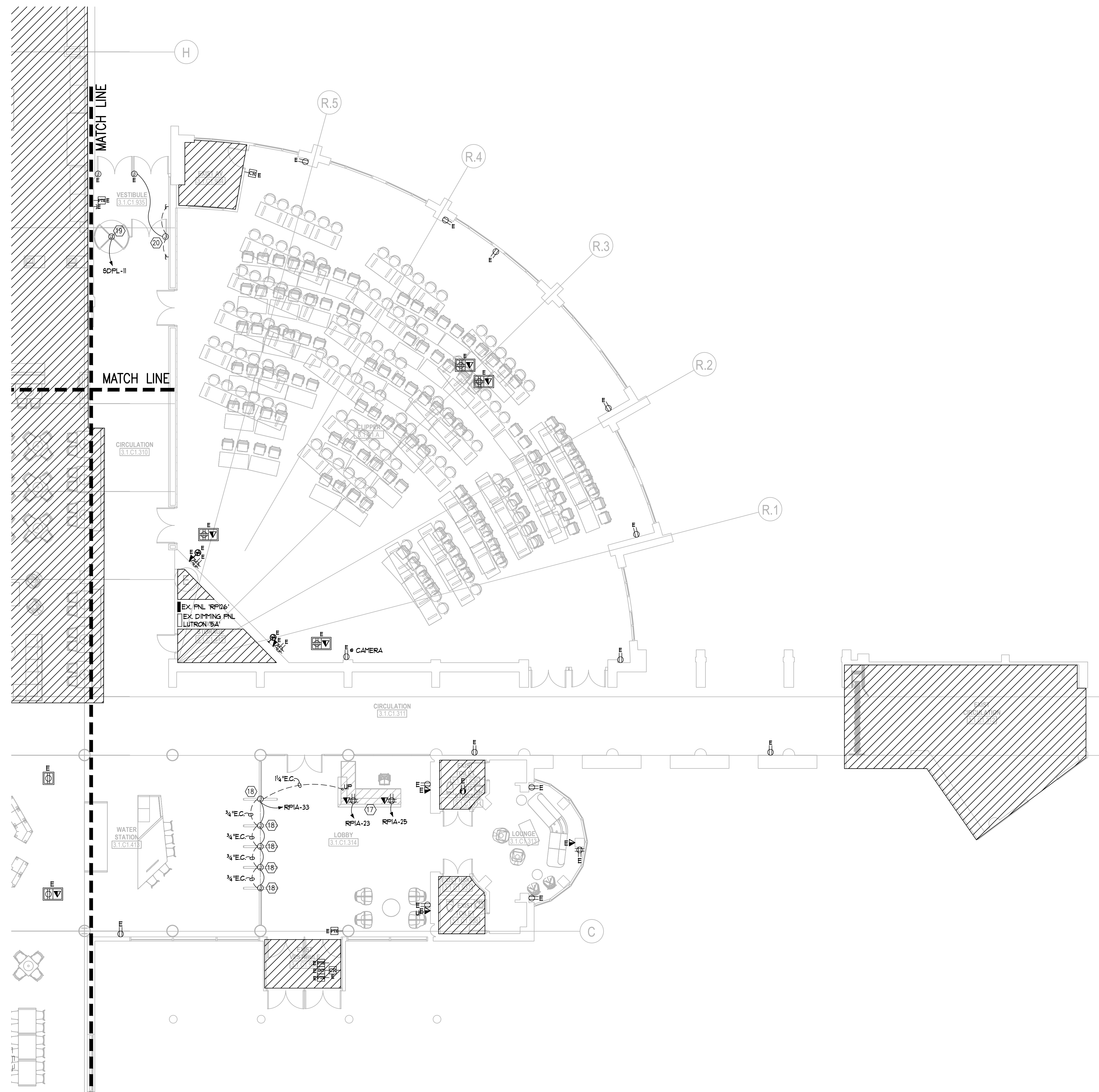
1 1ST FLOOR PLAN (AREA C1) - ELECTRICAL 1/8"=1'-0"
