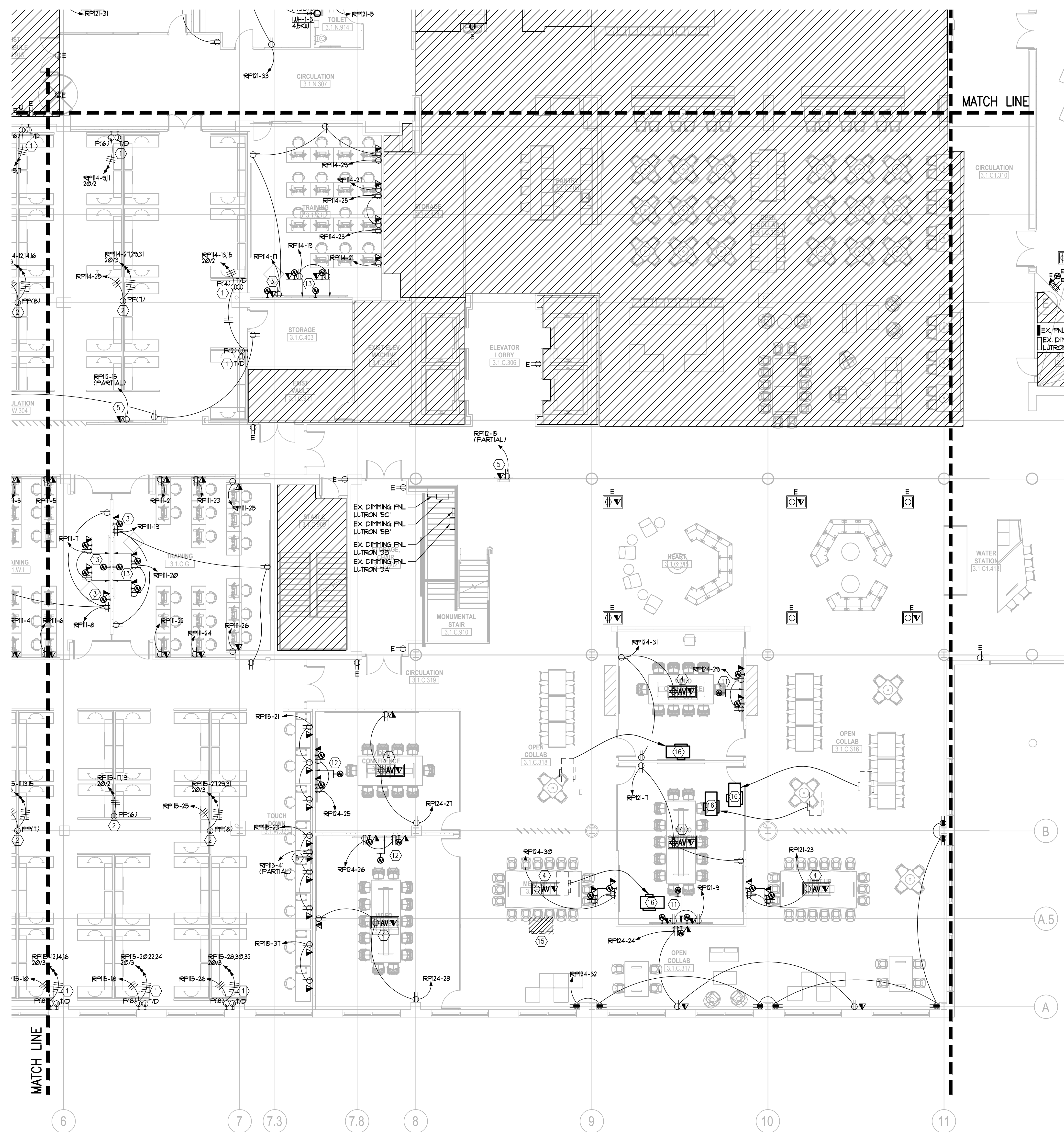
1 1ST FLOOR PLAN (AREA C) - ELECTRICAL E2.101C 3/8"=1'-0"
