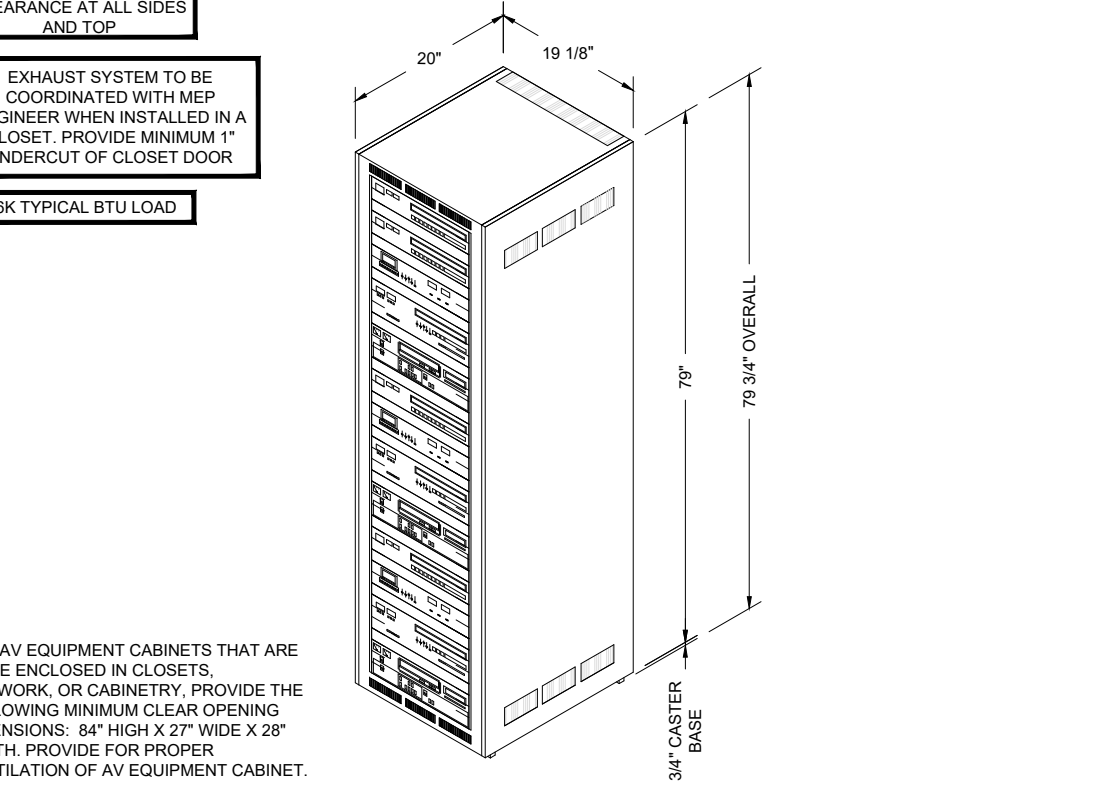
AV EQUIPMENT CABINET WITH CASTERS WEIGHT (LBS) 400 13
