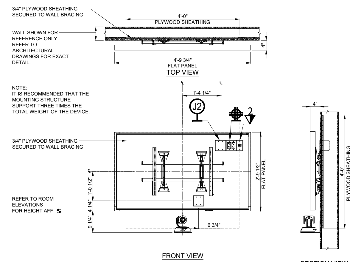
65" FLAT PANEL WITH CAMERA BELOW WEIGHT (LBS) 105 03
