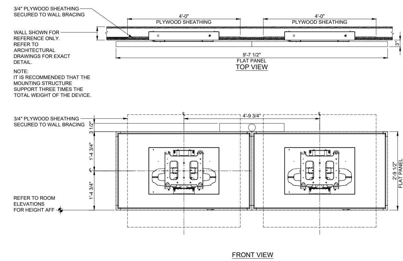
DUAL 65" FLAT PANEL WITH SPARK SYSTEM ABOVE WEIGHT (LBS) 245 01
