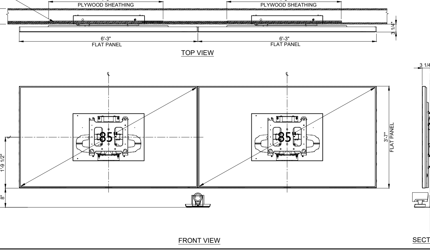
DUAL 85" DISPLAY W/ CAMERA BELOW WEIGHT (LBS) 300 17
