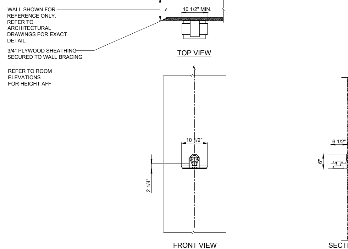
WALL MOUNTED CAMERA WEIGHT (LBS) 55 15
