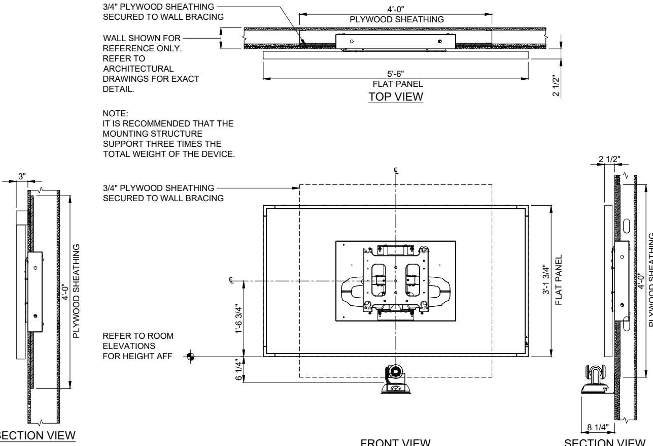
75" FLAT PANEL DISPLAYS WITH CAMERA BELOW WEIGHT (LBS) 85 02
