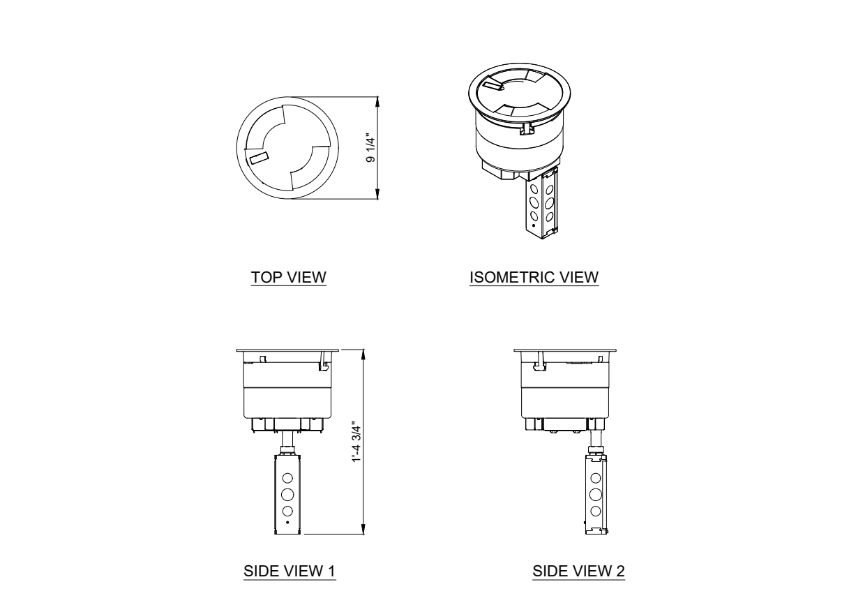
FLOOR POKE THRU WEIGHT (LBS) 20 05
