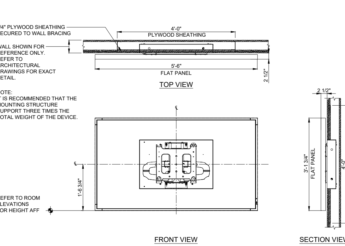
75" FLAT PANEL DISPLAY WEIGHT (LBS) 128 14
