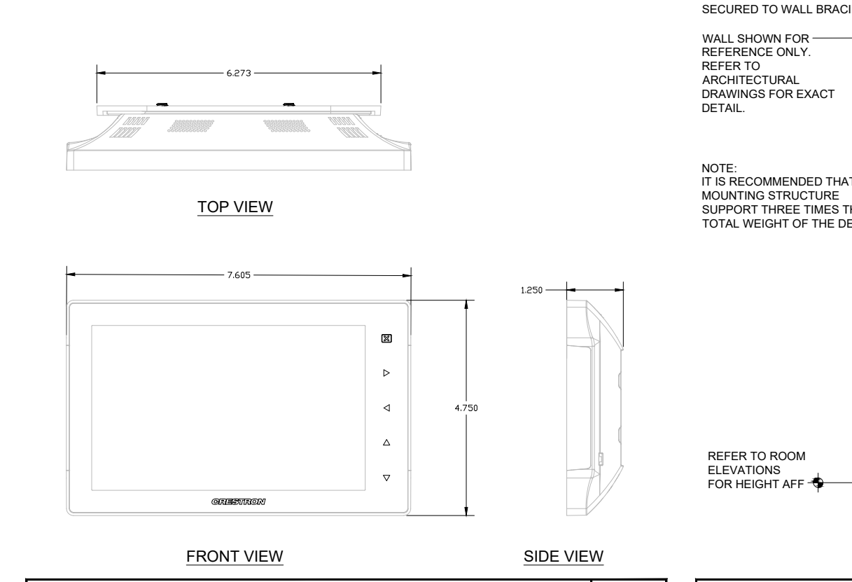
ROOM SCHEDULING TOUCH SCREEN- IN WALL WEIGHT (LBS) 1 16
