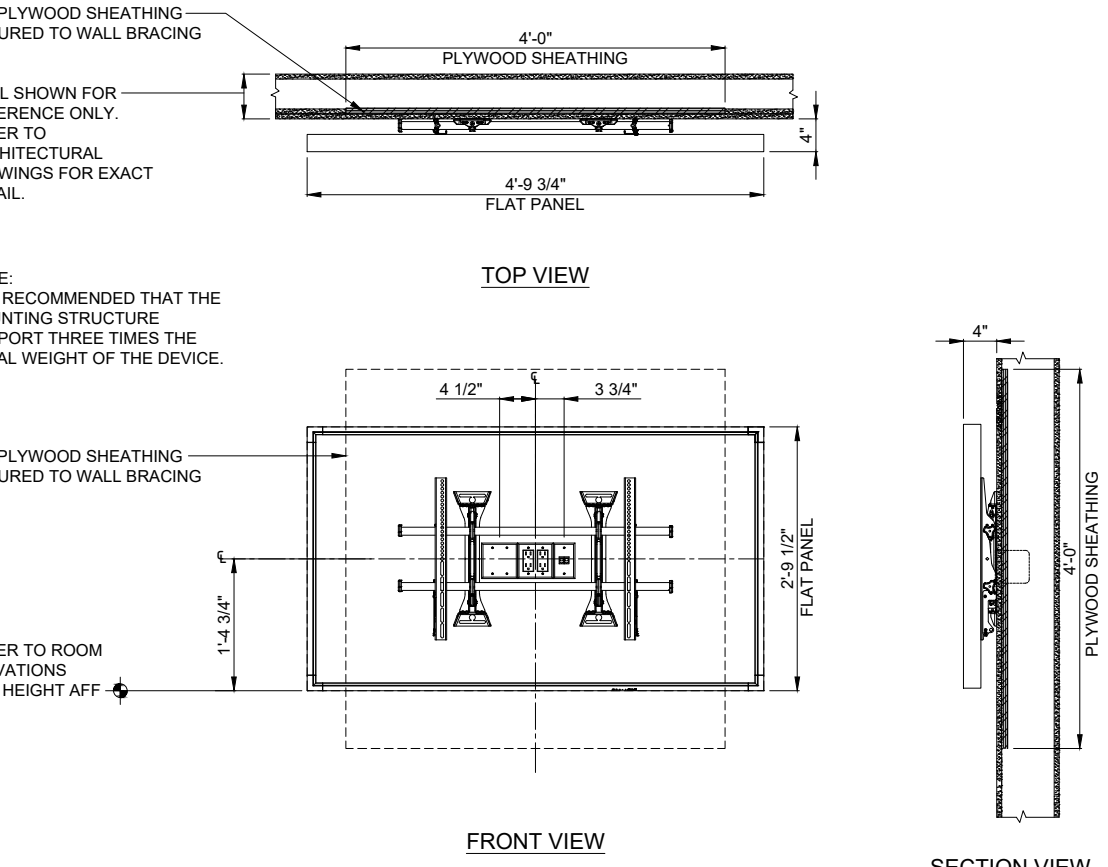
65" FLAT PANEL WEIGHT (LBS) 80 06
