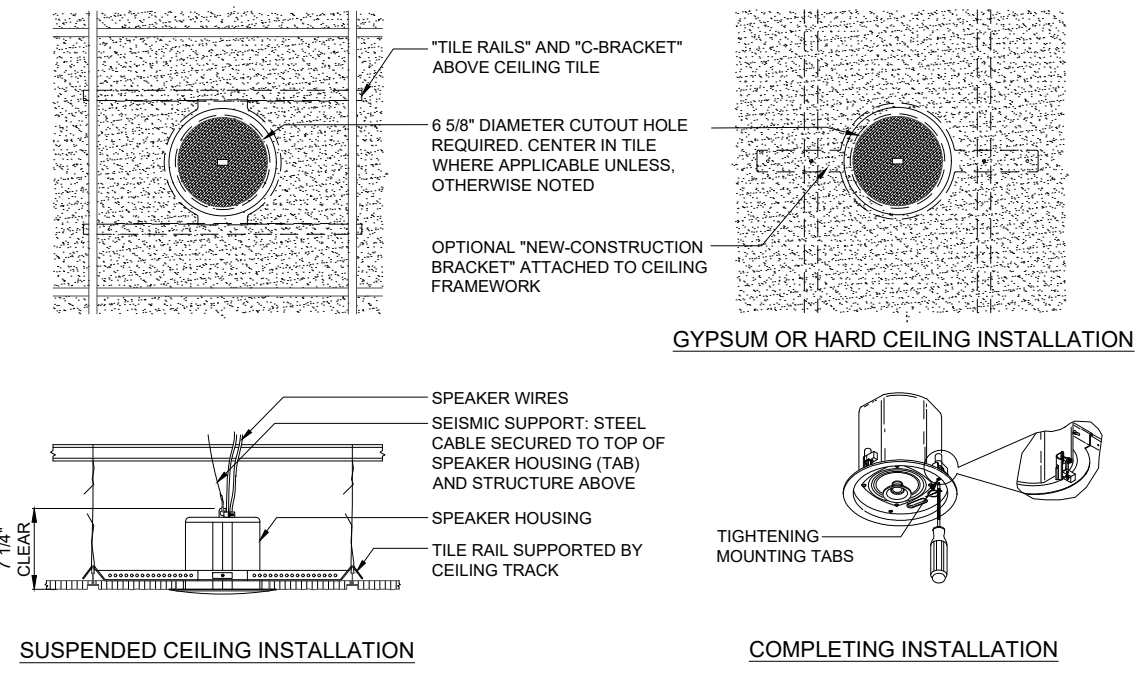
JBL CONTROL 24CT - CEILING SPEAKER WEIGHT (LBS) 5 04
