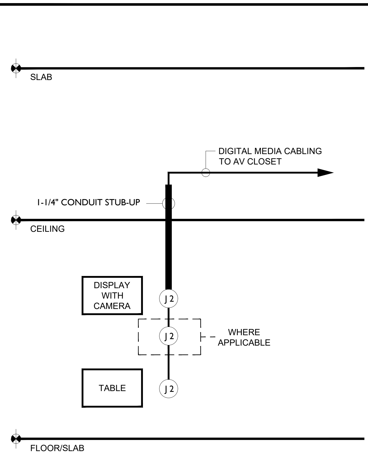
AUDIOVISUAL RISER DIAGRAM (FULL PRESENTATION)
