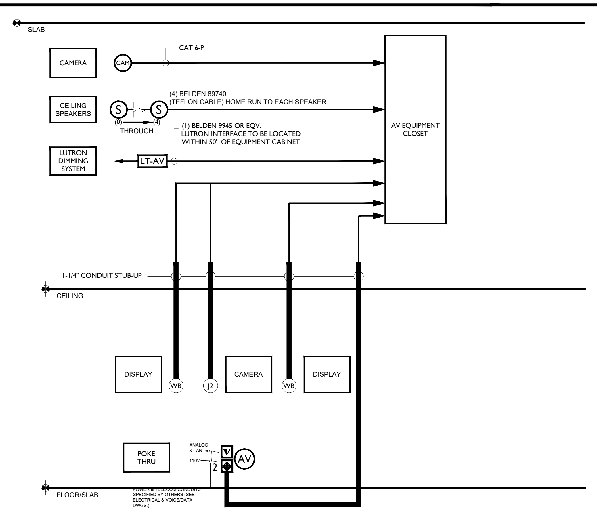
AUDIOVISUAL RISER DIAGRAM (VIDEO TELEPRESENCE CONFERENCE ROOM)
