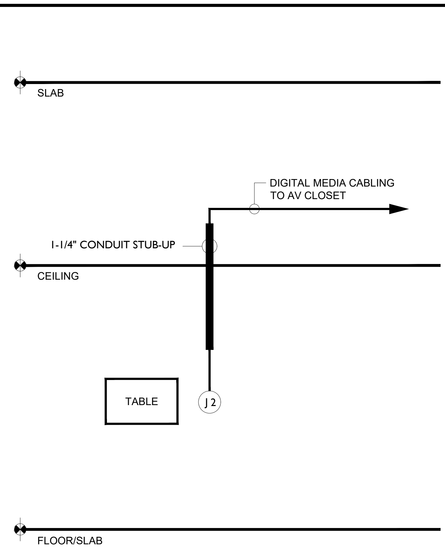
AUDIOVISUAL RISER DIAGRAM (PRESENTATION LITE)
