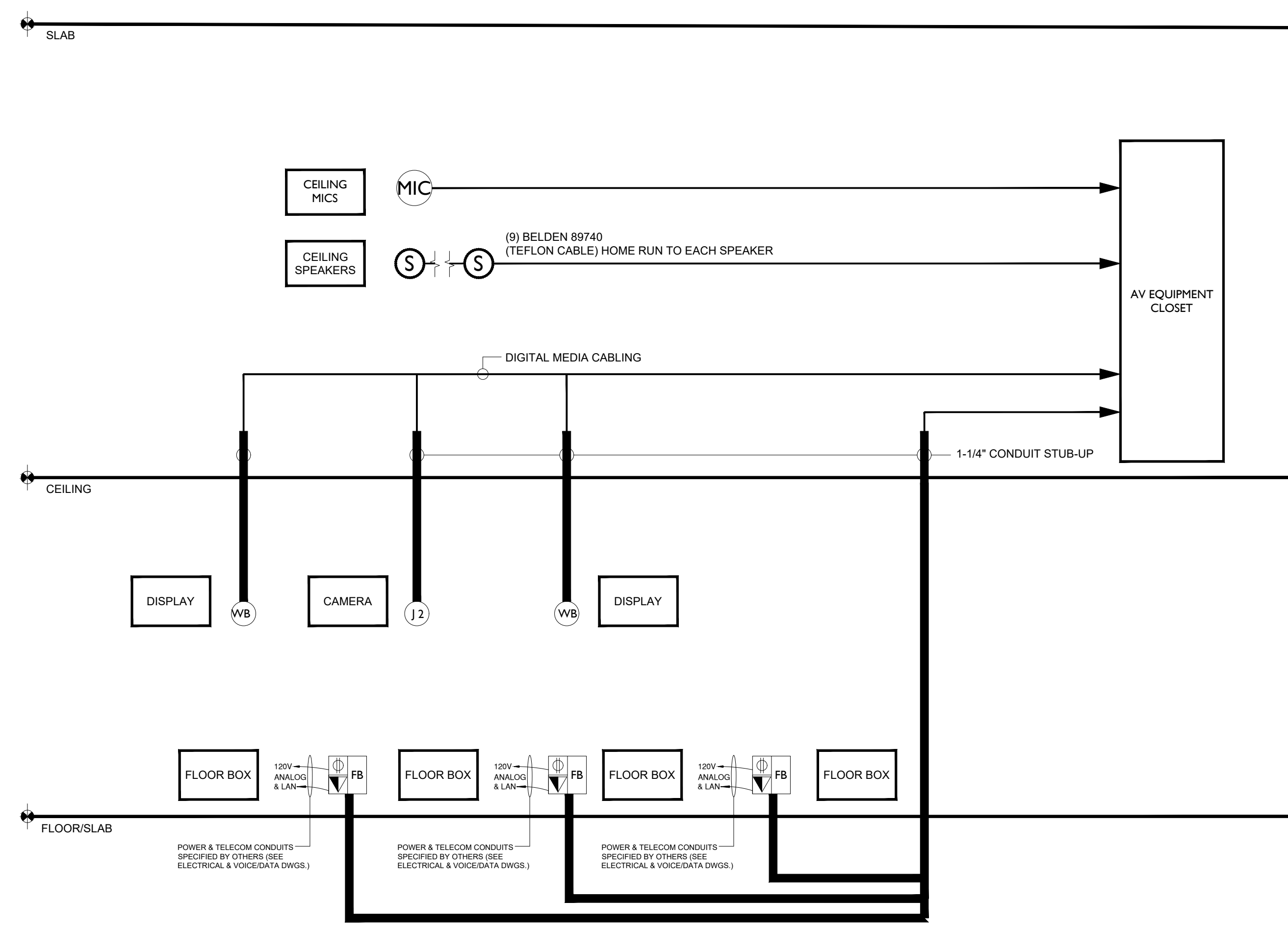
AUDIOVISUAL RISER DIAGRAM (TRAINING ROOM)
