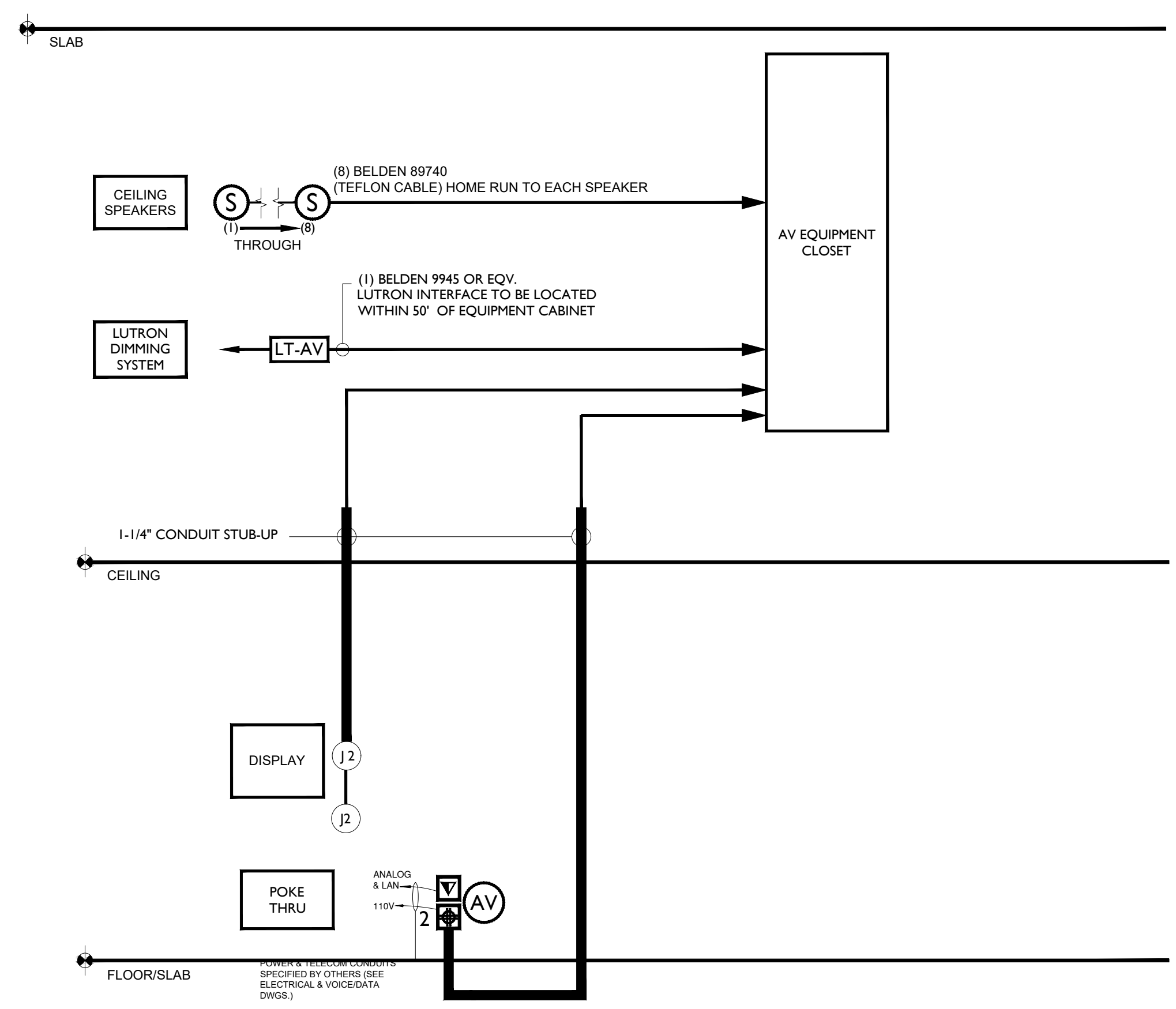
AUDIOVISUAL RISER DIAGRAM (FULL PRESENTATION)
