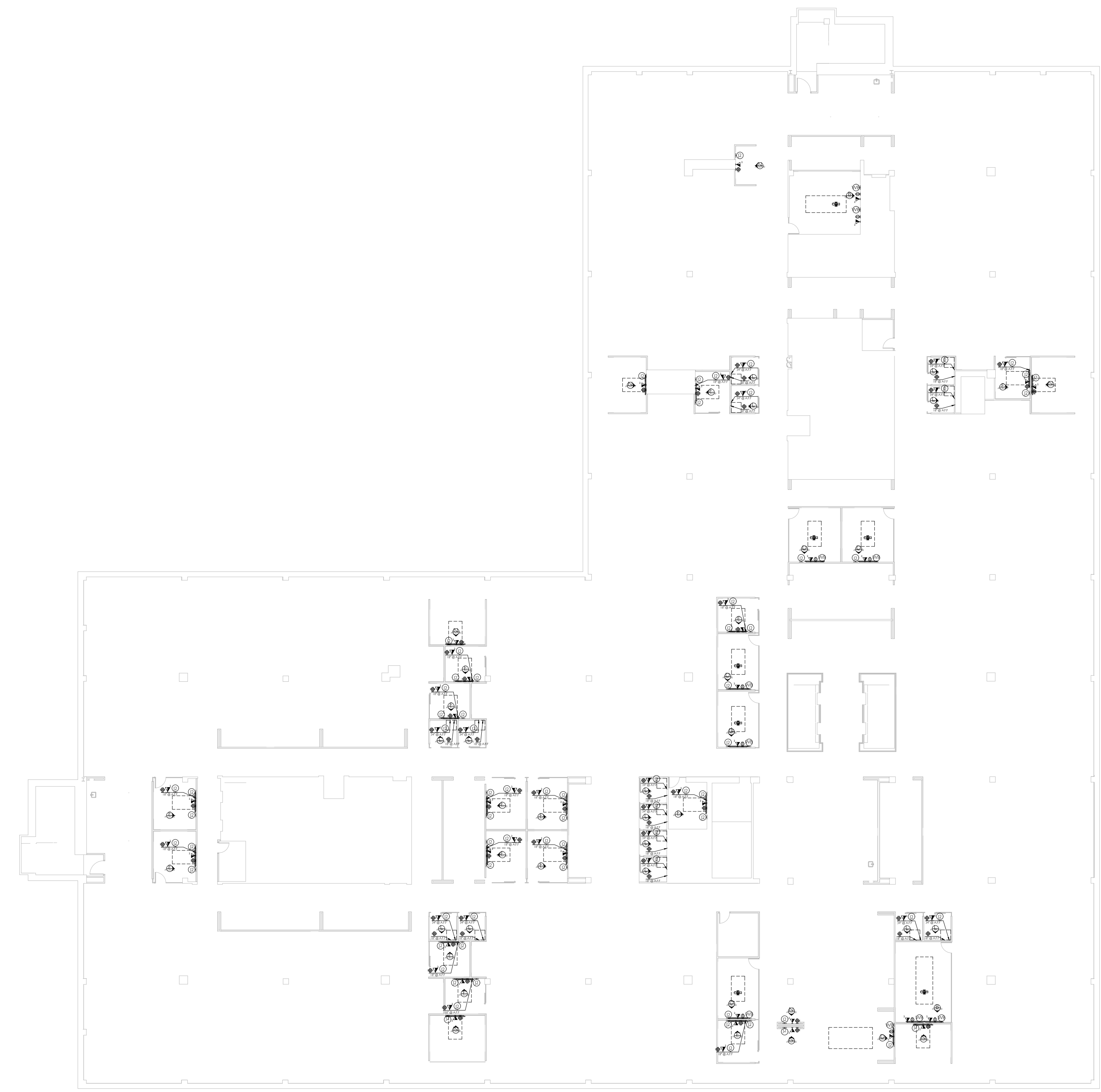
AUDIOVISUAL ELECTRICAL PLAN FLOOR #HO3-04 SCALE SIZE: 1/16" = 1'-0" B
