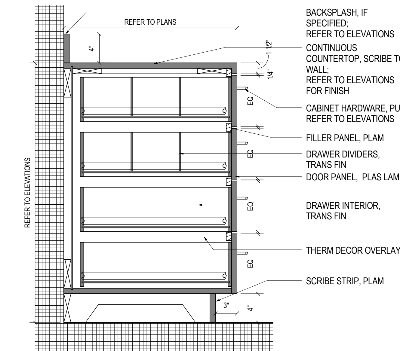
07 BASE CABINET - FOUR DRAWERS SCALE: 1 1/2" = 1'-0"
