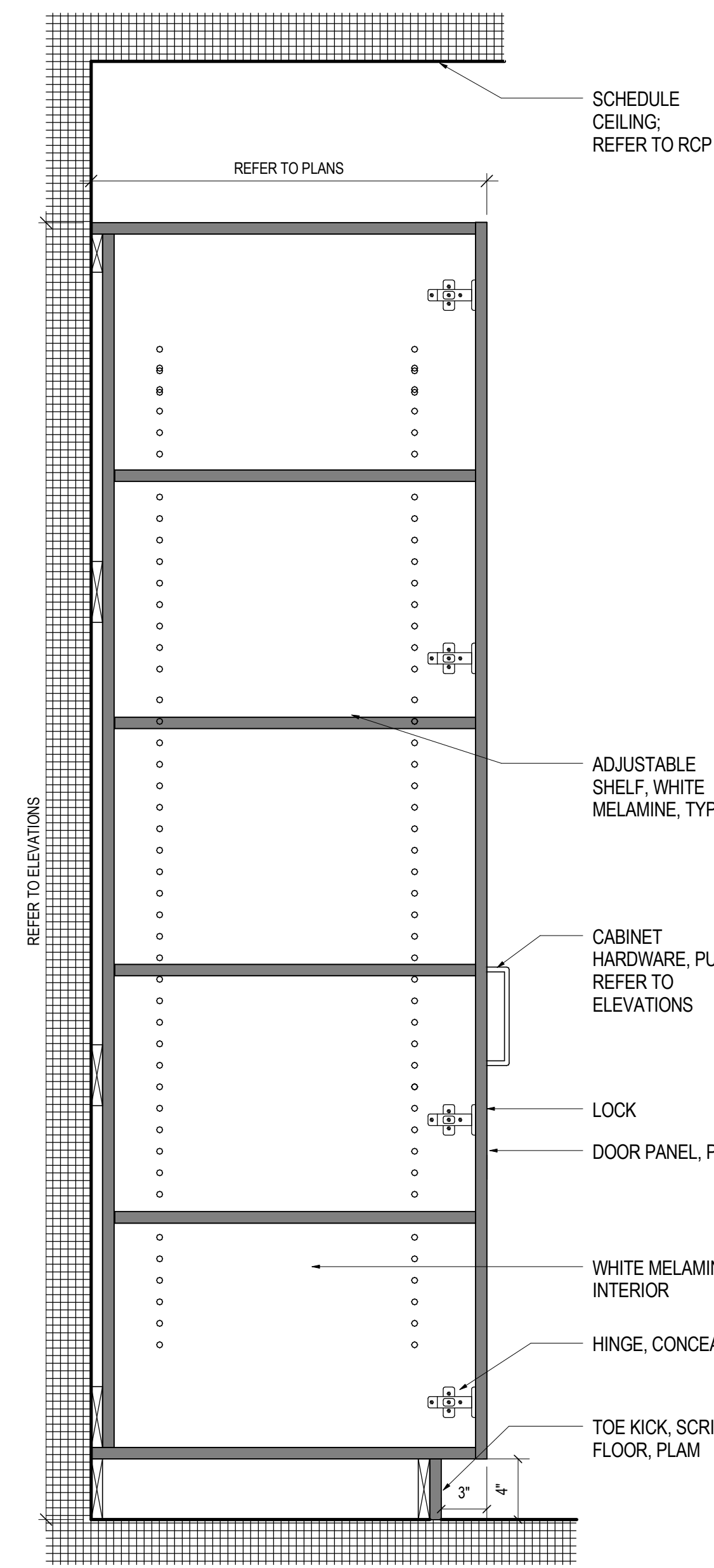
09 FULL HEIGHT CABINET SCALE: 1 1/2" = 1'-0"
