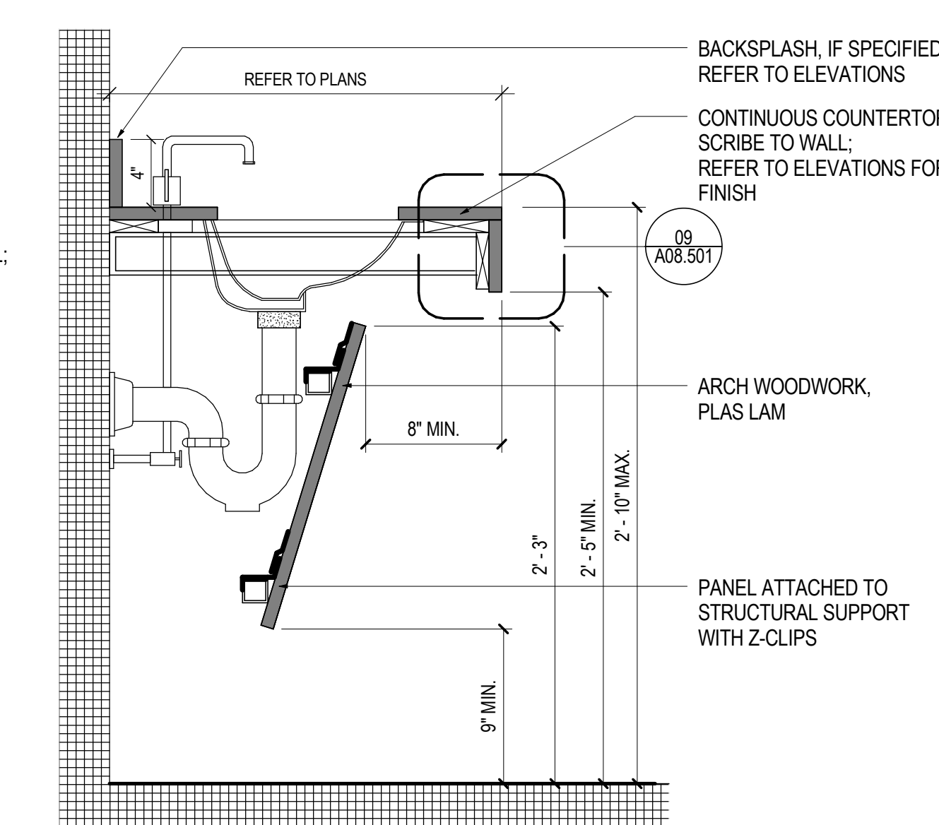
03 COUNTER - ADA LAVATORY SCALE: 1 1/2" = 1'-0"
