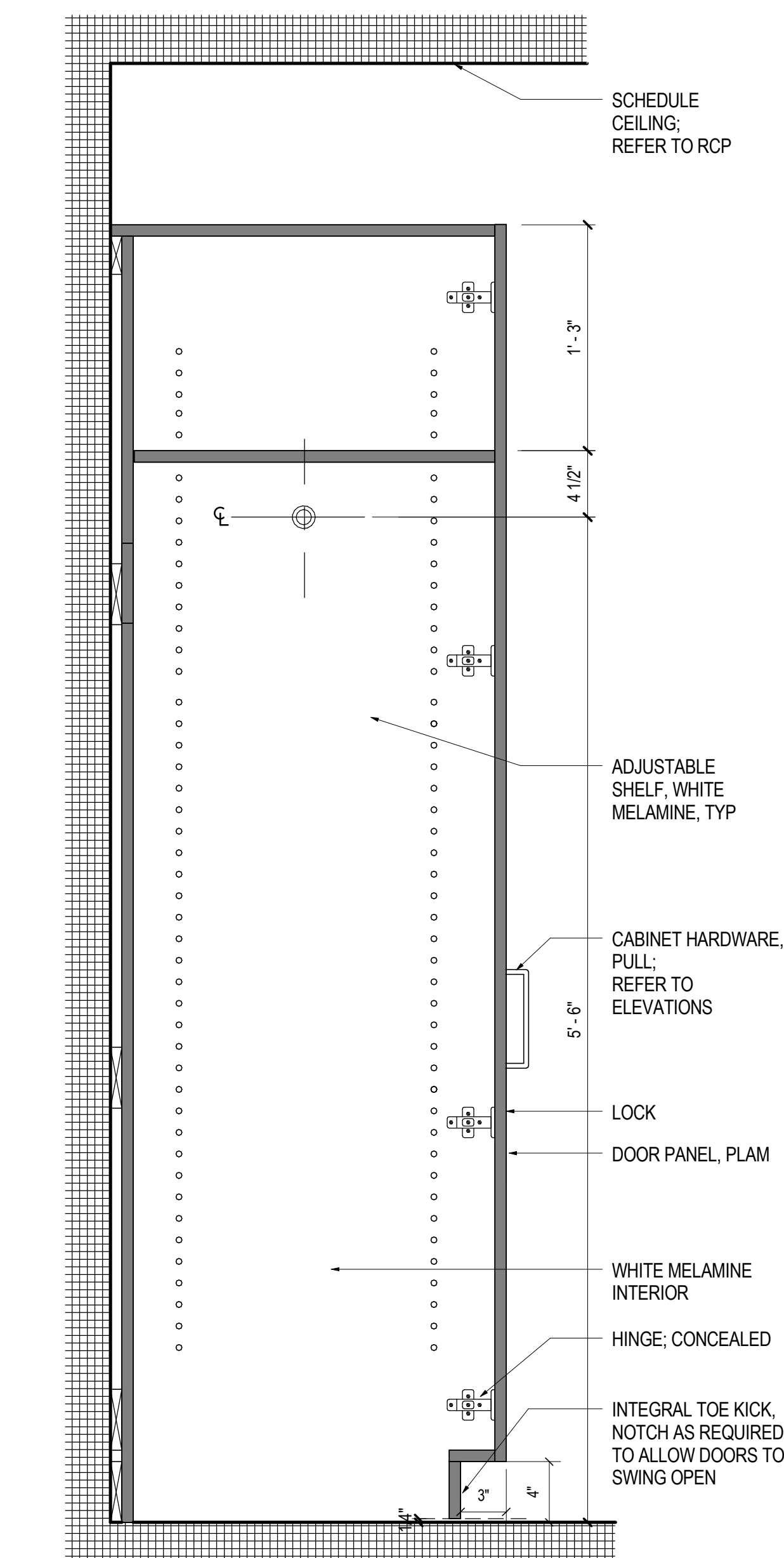
10 FULL HEIGHT LUGGAGE STORAGE SCALE: 1 1/2" = 1'-0"
