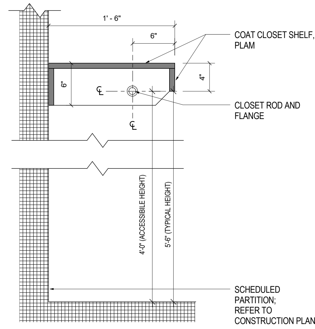
12 CLOSET SHELF AND ROD SCALE: 1 1/2" = 1'-0"
