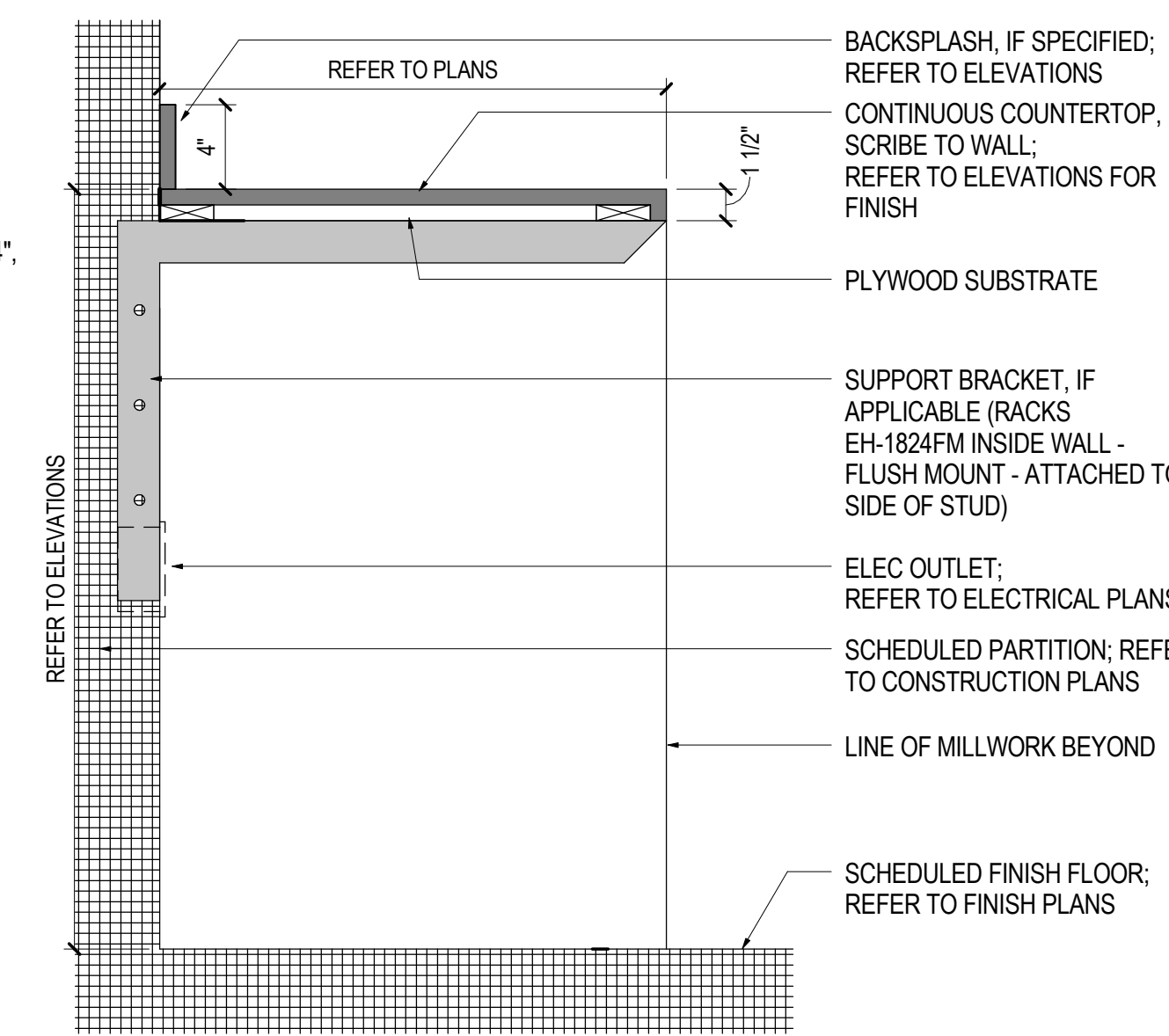
01 COUNTER - OPEN SCALE: 1 1/2" = 1'-0"
