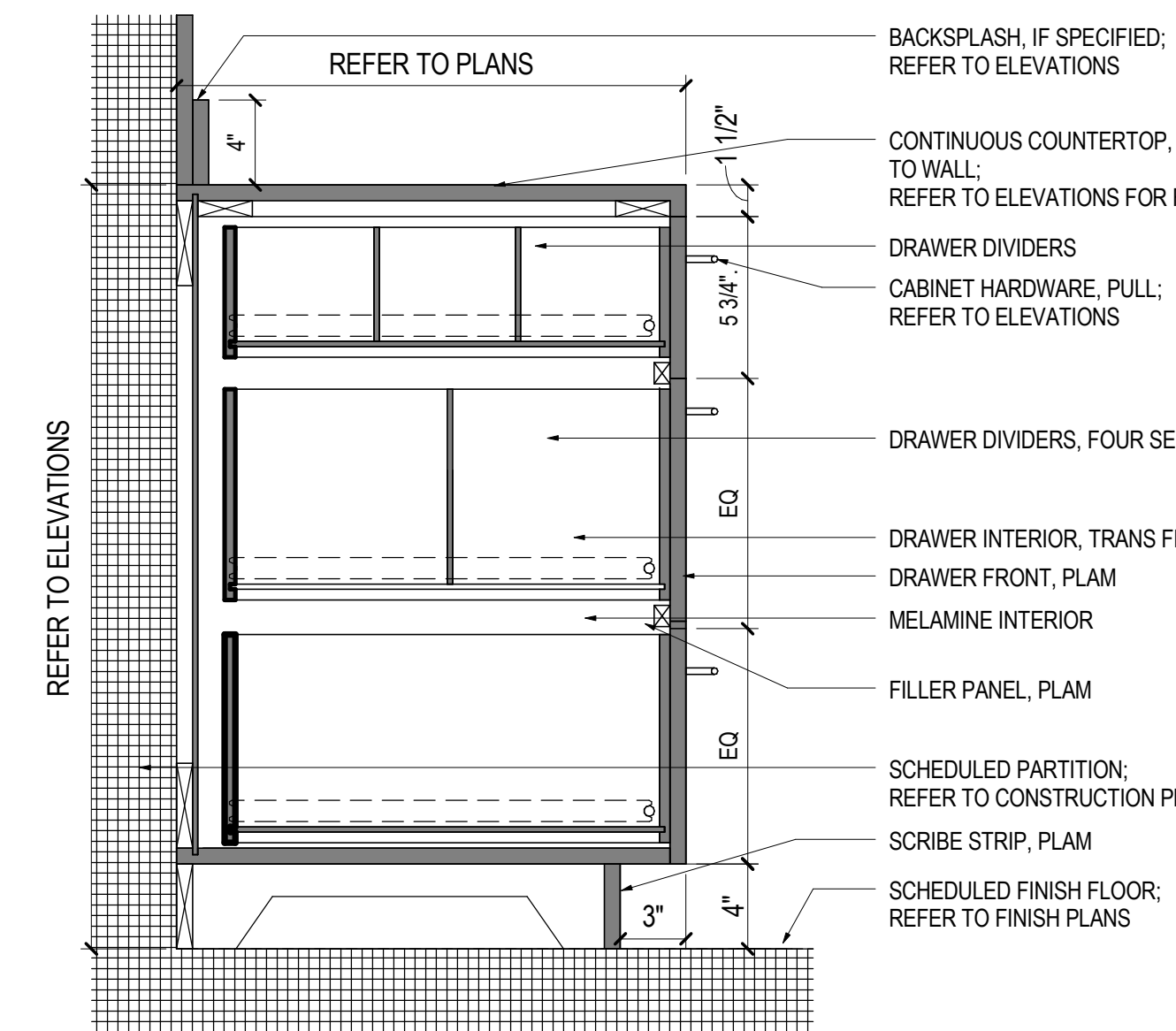
06 BASE CABINET - THREE DRAWERS SCALE: 1 1/2" = 1'-0"
