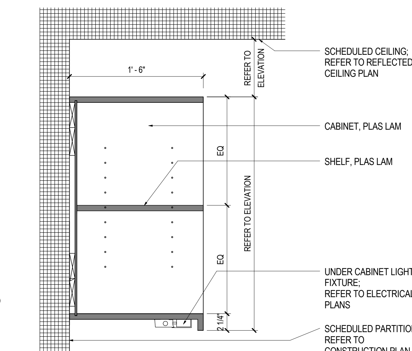
08 UPPER CABINET - OPEN SHELVES SCALE: 1 1/2" = 1'-0"
