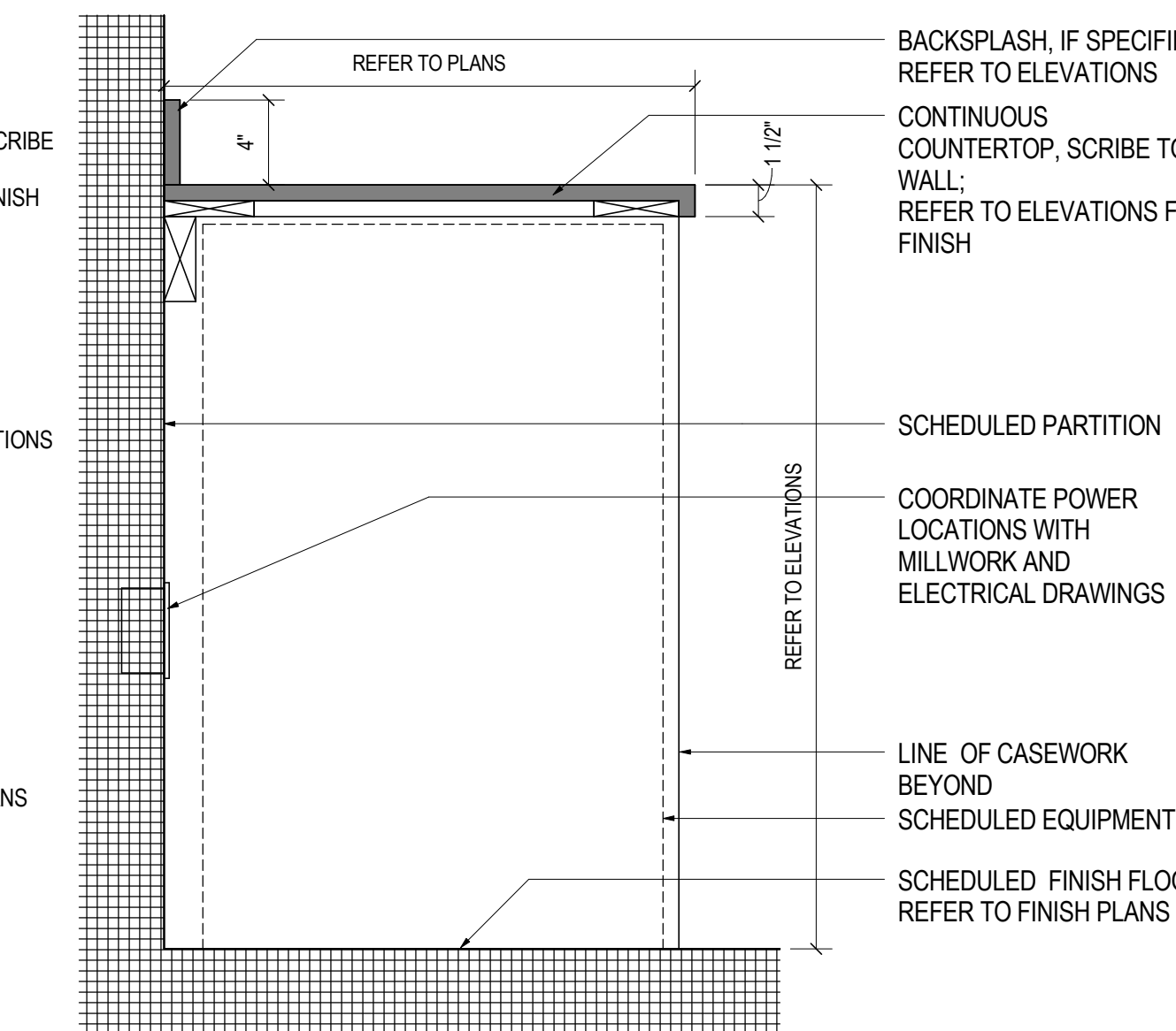
02 COUNTER - EQUIPMENT SCALE: 1 1/2" = 1'-0"
