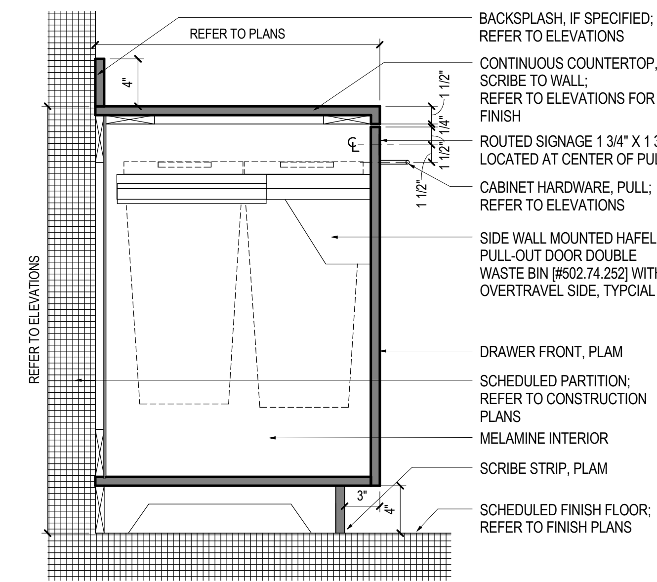
05 BASE CABINET - PULL-OUT TRASH SCALE: 1 1/2" = 1'-0"
