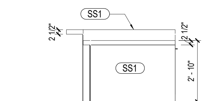
03 ANGLED DESK - SOUTH ELEVATION SCALE: 3/8" = 1'-0"
