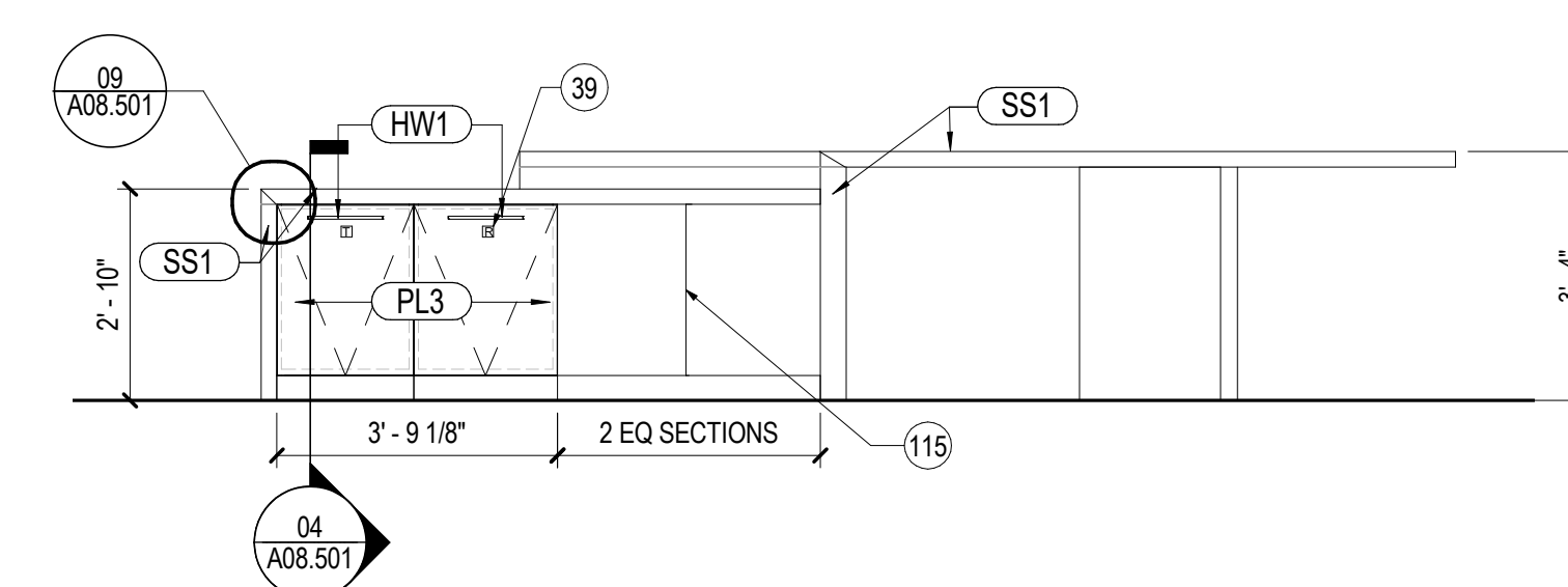
06 ANGLED DESK - EAST ELEVATION SCALE: 3/8" = 1'-0"
