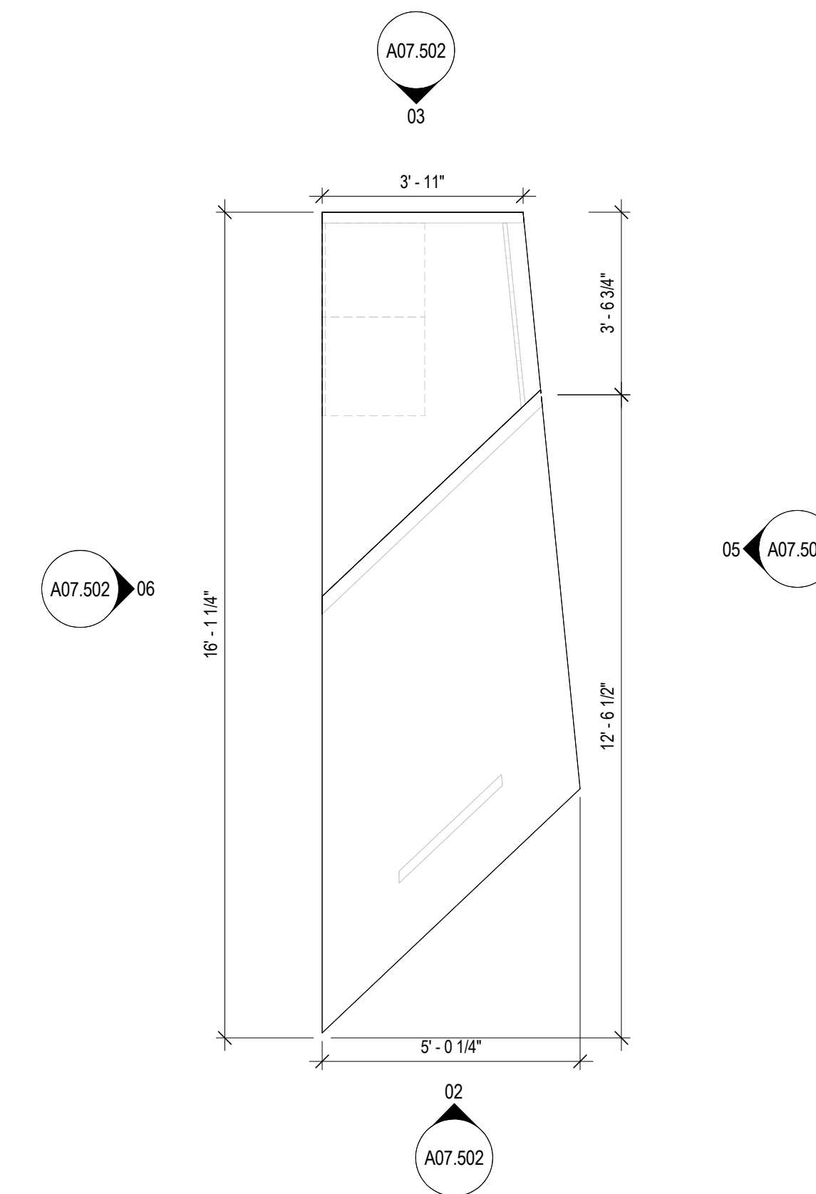
01 ENLARGED PLAN - LEVEL 01 - WATER STATION SCALE: 3/8" = 1'-0"
