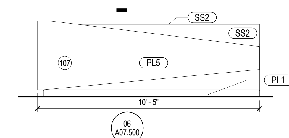
02 RECEPTION DESK - ELEVATION NORTH SCALE: 3/8" = 1'-0"
