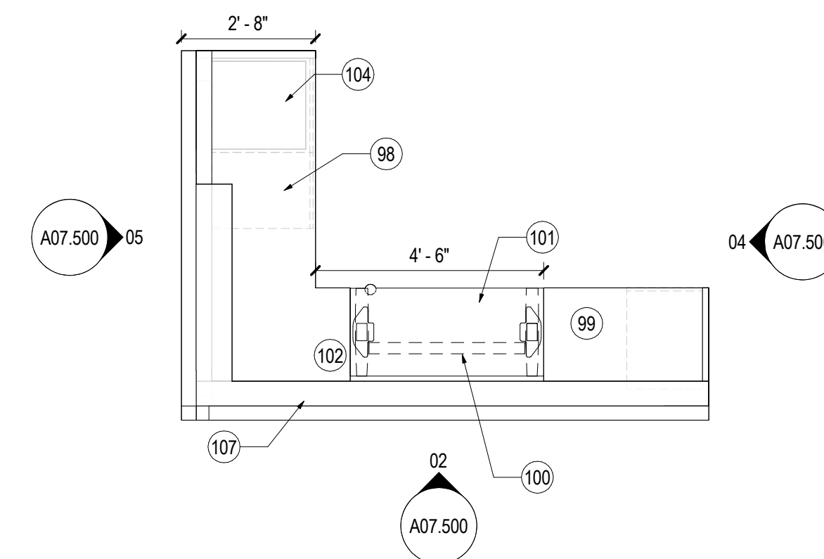
01 RECEPTION DESK - ENLARGED FLOOR PLAN SCALE: 3/8" = 1'-0"
