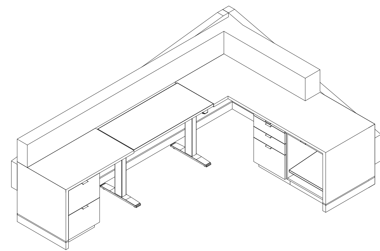
08 RECEPTION DESK AXON Copy 1 SCALE:
