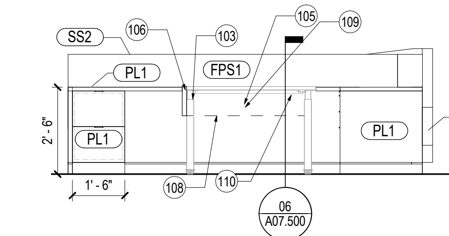
03 RECEPTION DESK - ELEVATION SOUTH SCALE: 3/8" = 1'-0"
