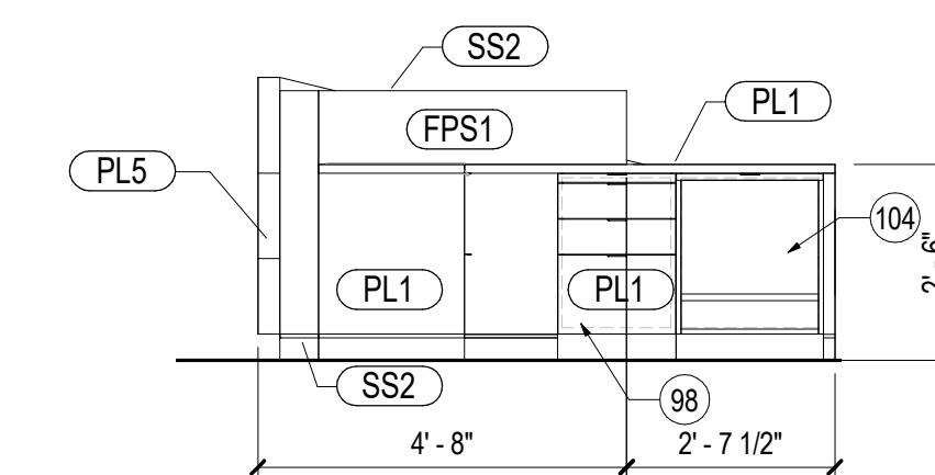
04 RECEPTION DESK - ELEVATION WEST SCALE: 3/8" = 1'-0"
