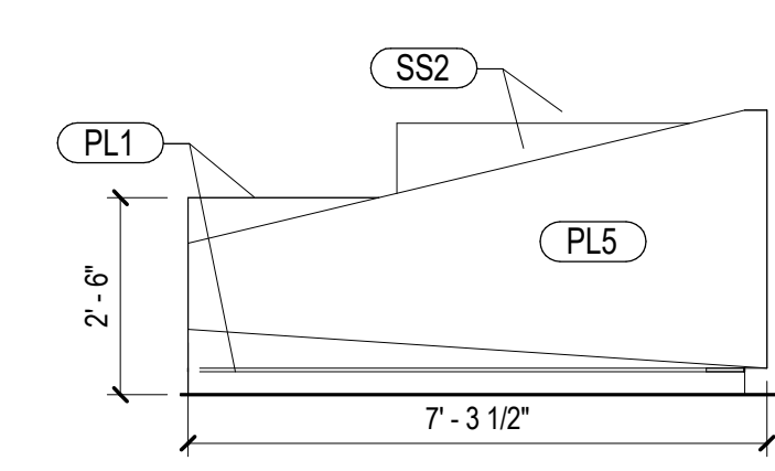
05 RECEPTION DESK - ELEVATION EAST SCALE: 3/8" = 1'-0"
