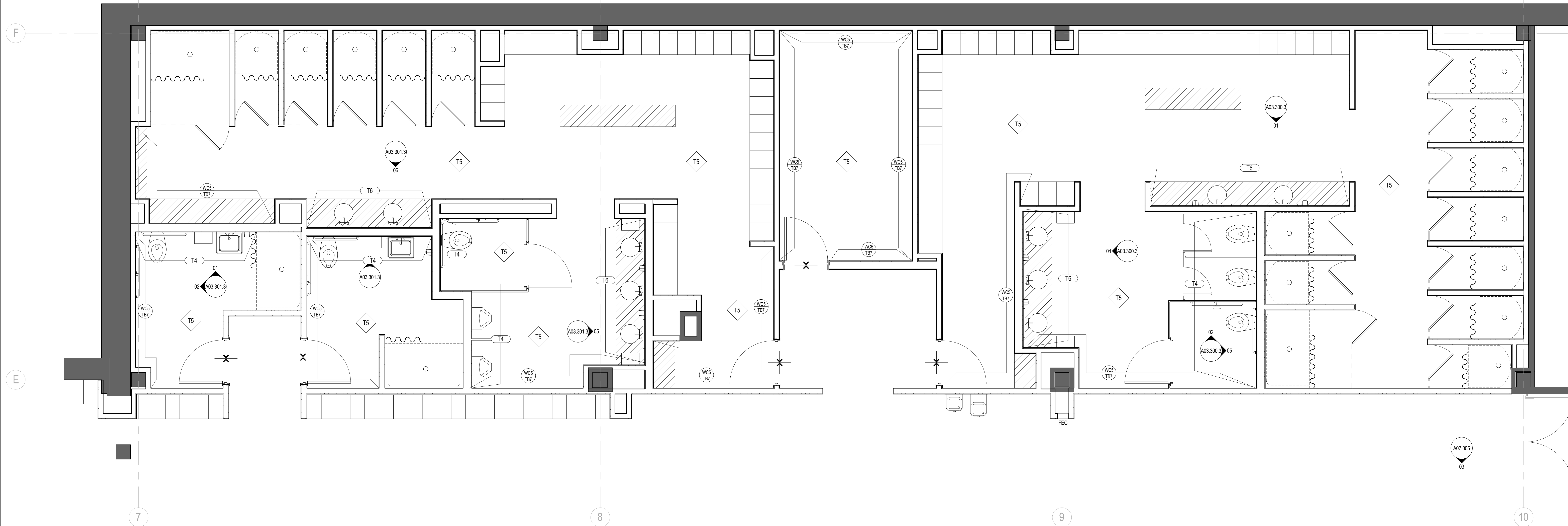
01 ENLARGED FITNESS LOCKER ROOM PLAN SCALE: 3/8" = 1'-0"
