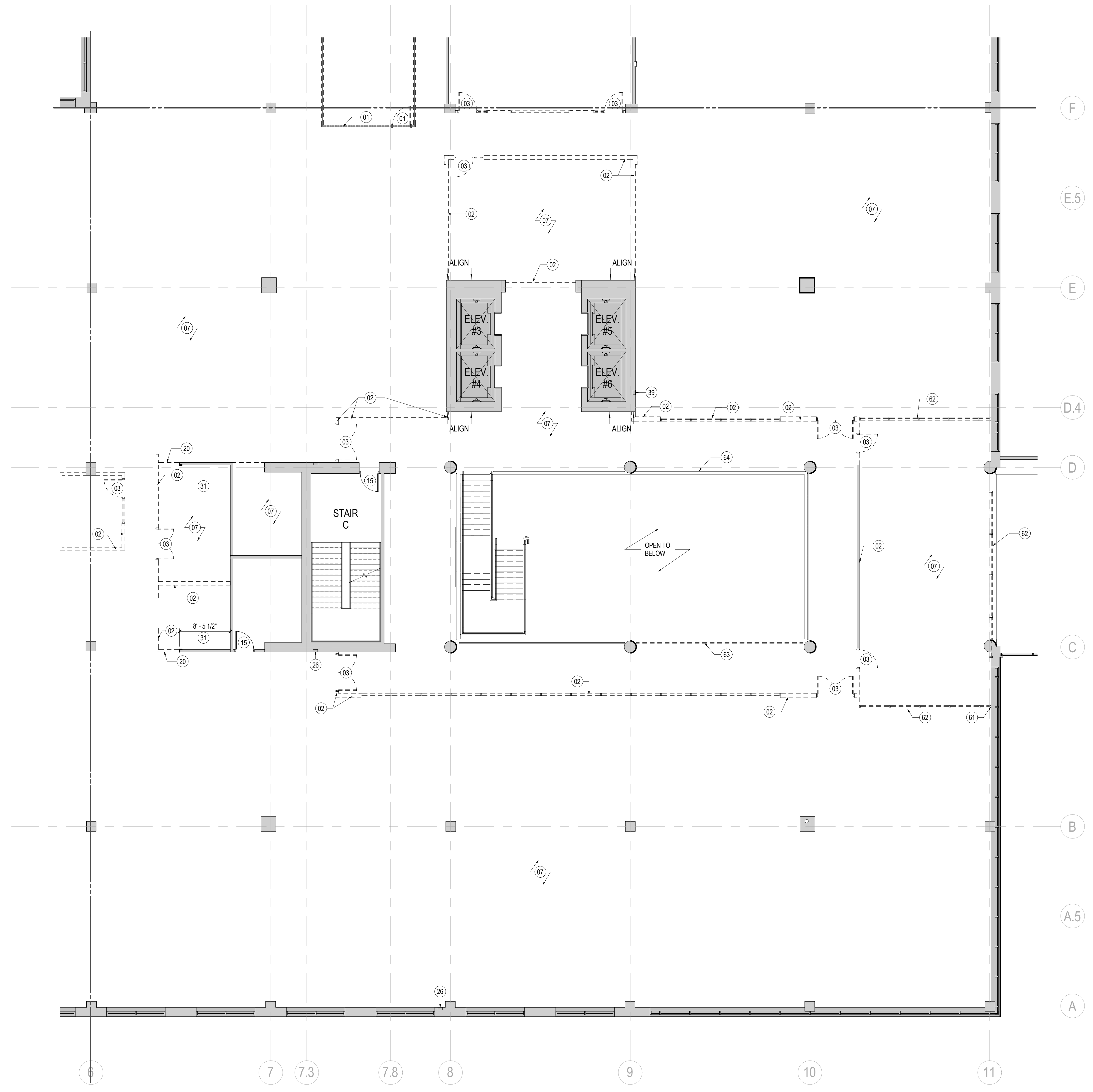
01 DEMOLITION PLAN - LEVEL 02 - AREA C SCALE: 1/8" = 1'-0"
