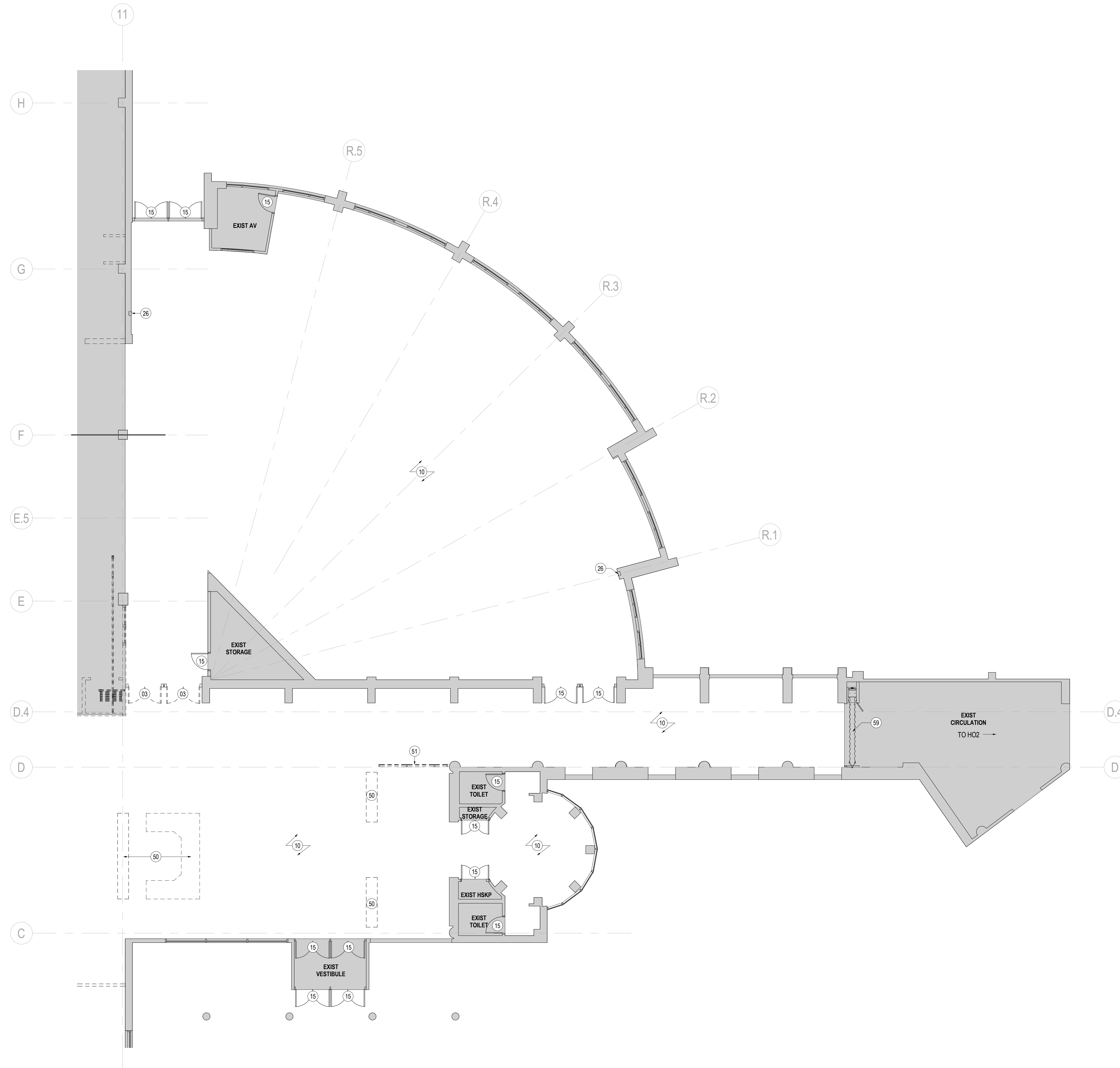
01 DEMOLITION PLAN - LEVEL 01 - AREA C1 SCALE: 1/8" = 1'-0"
