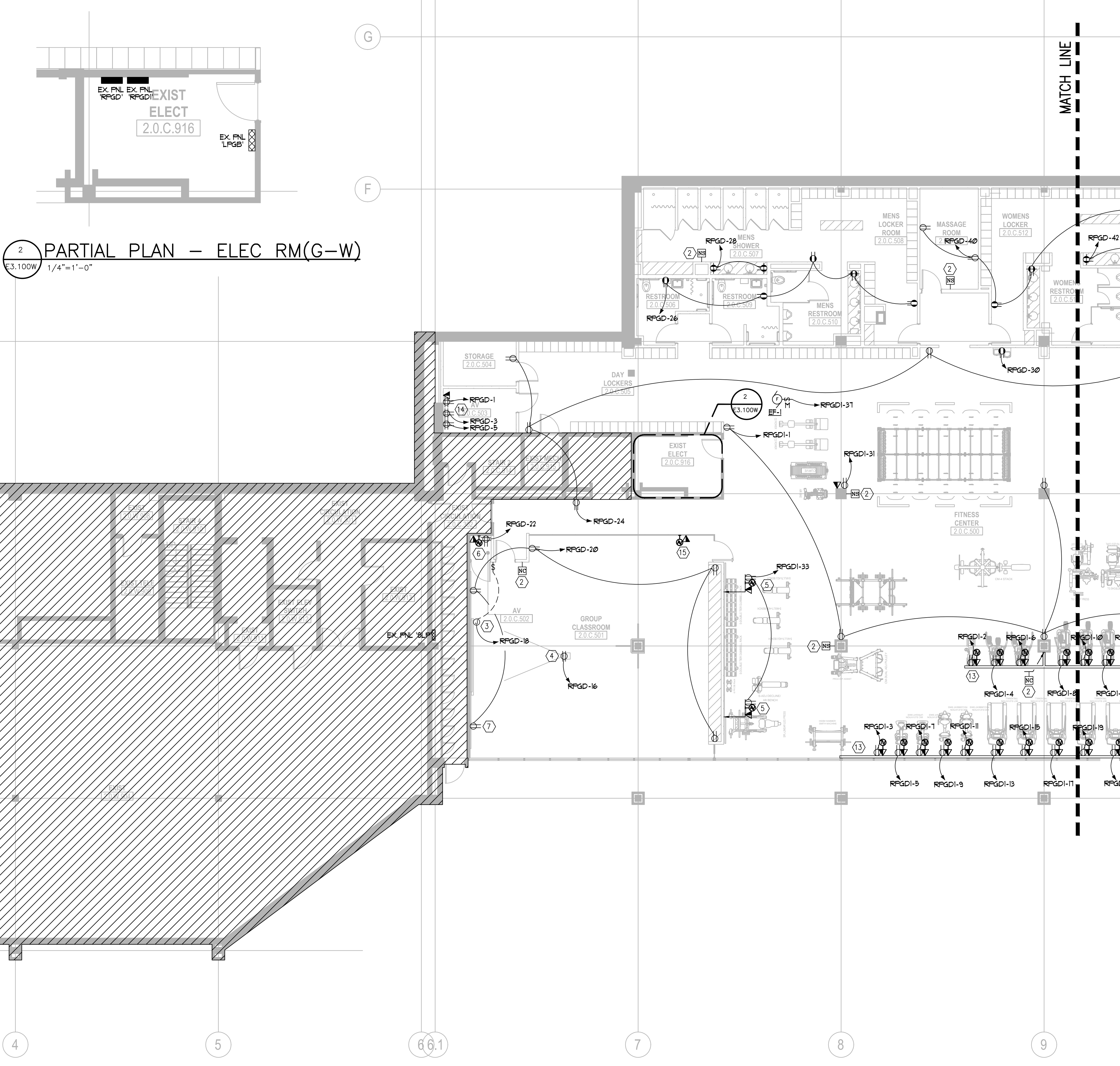
1 GROUND FLOOR PLAN (WEST) - ELECTRICAL 3.100W 1/8"=1'-0"
