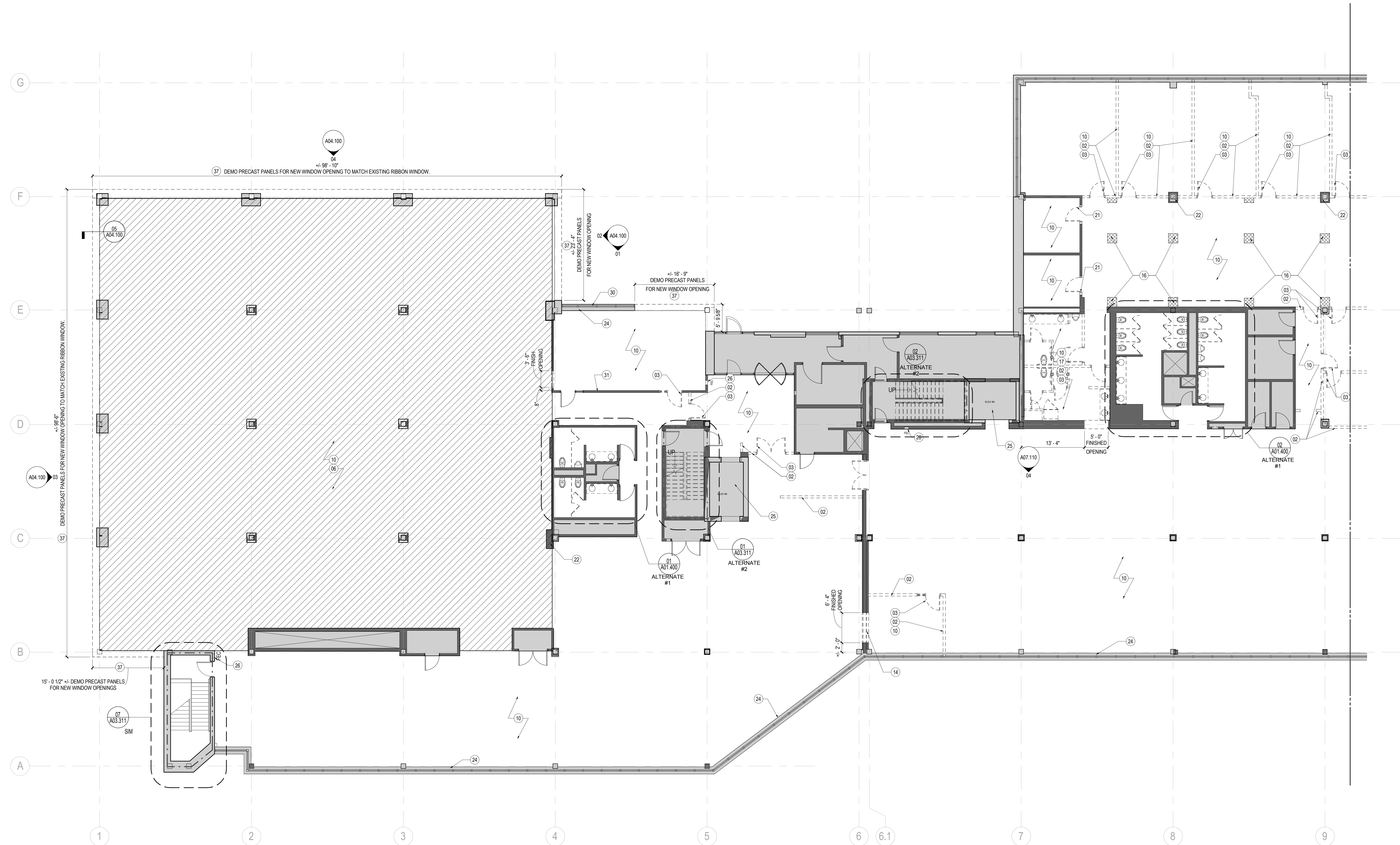
01 DEMOLITION PLAN - LEVEL 01 - WEST SCALE: 1/8" = 1'-0"
