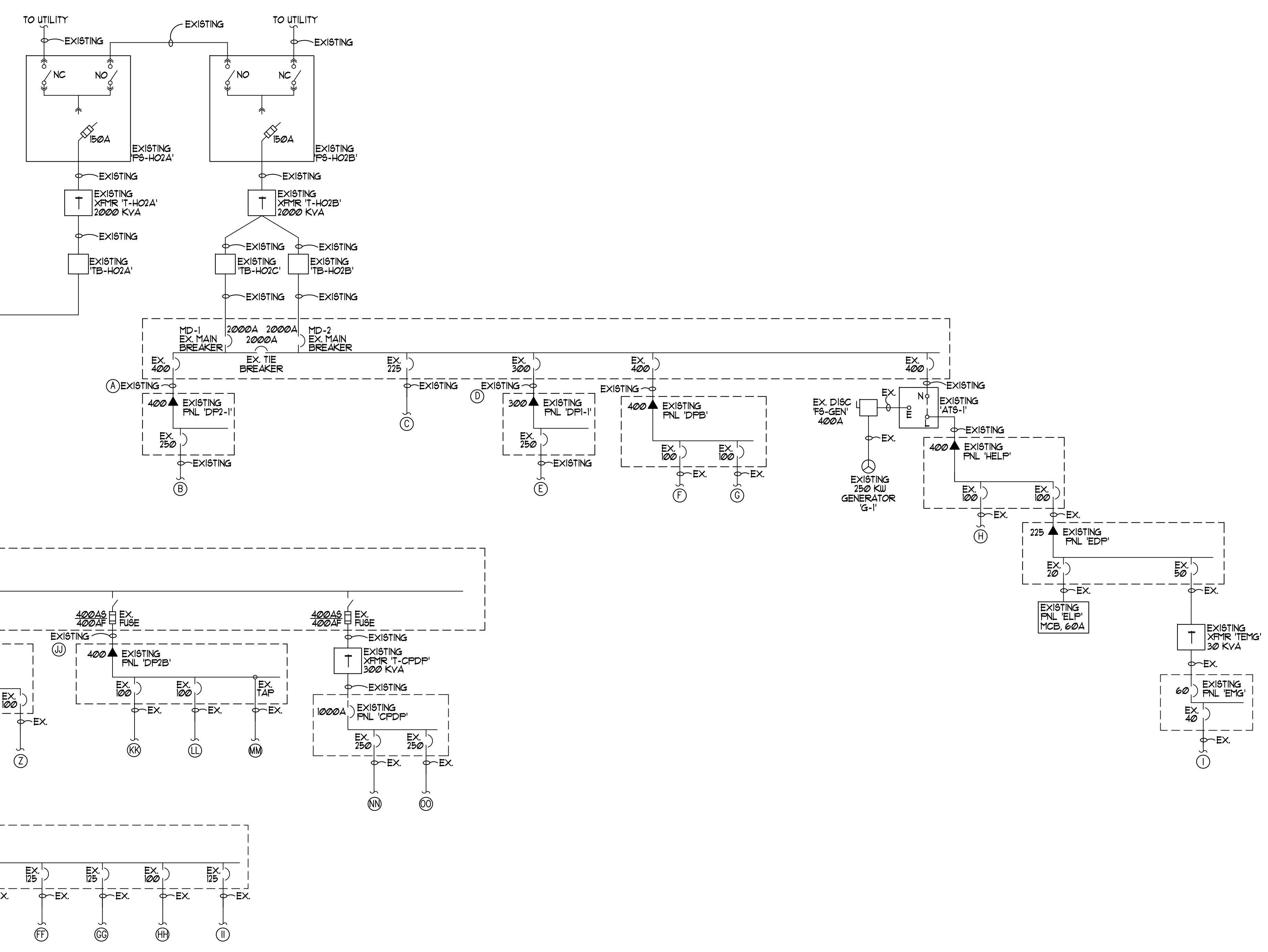
1 POWER RISER DIAGRAM E1.500 NOT TO SCALE
