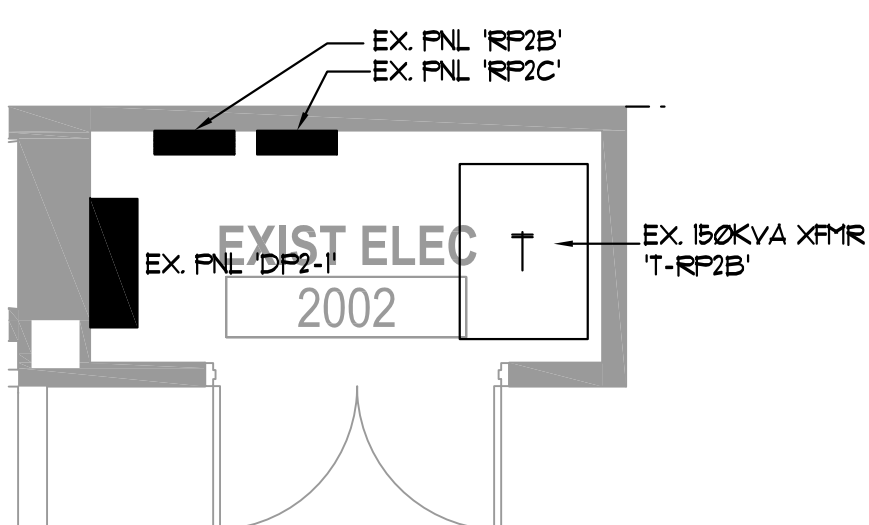
10 PARTIAL PLAN - ELEC RM(2-W) E1.400 1/4"=1'-0"
