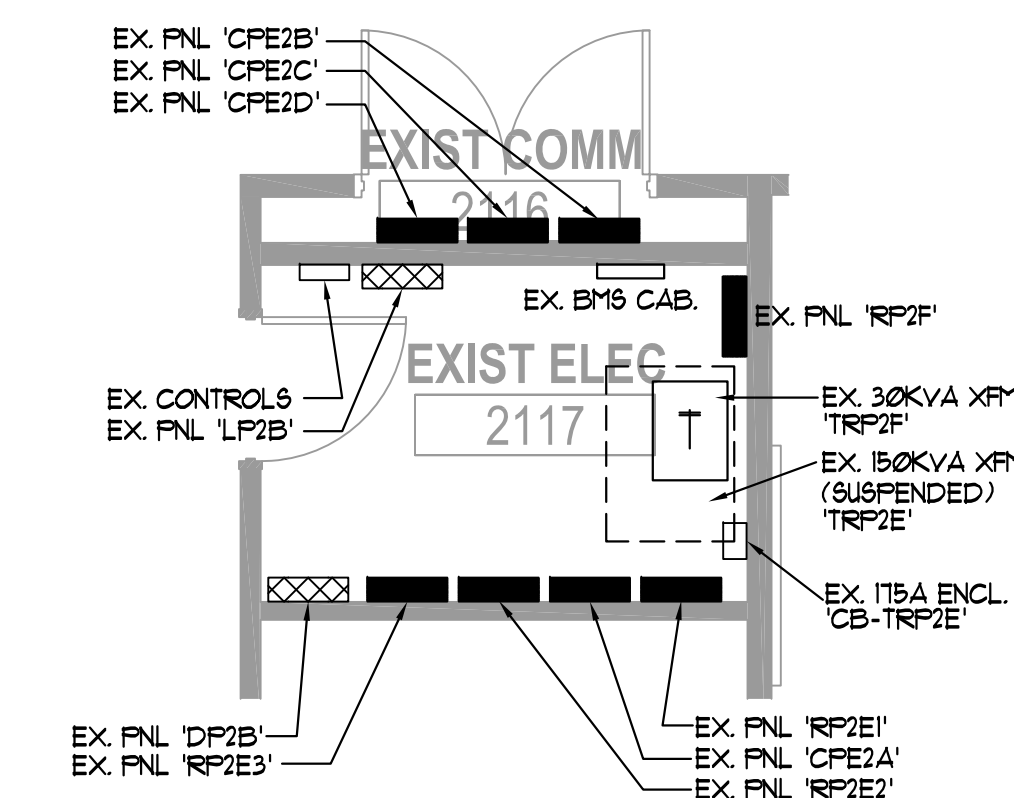
6 PARTIAL PLAN - ELEC RM(2-E) E1.400 1/4"=1'-0"
