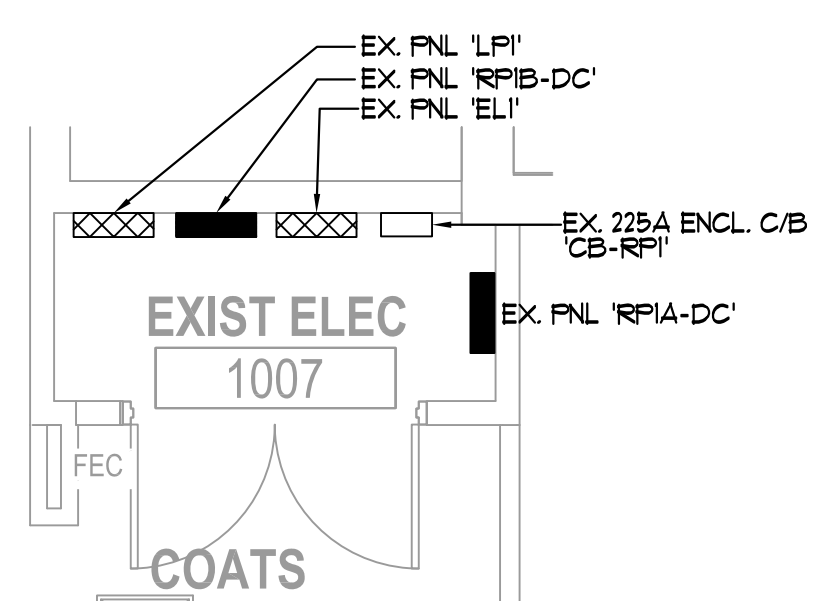
4 PARTIAL PLAN - ELEC RM(1-W) E1.400 1/4"=1'-0"
