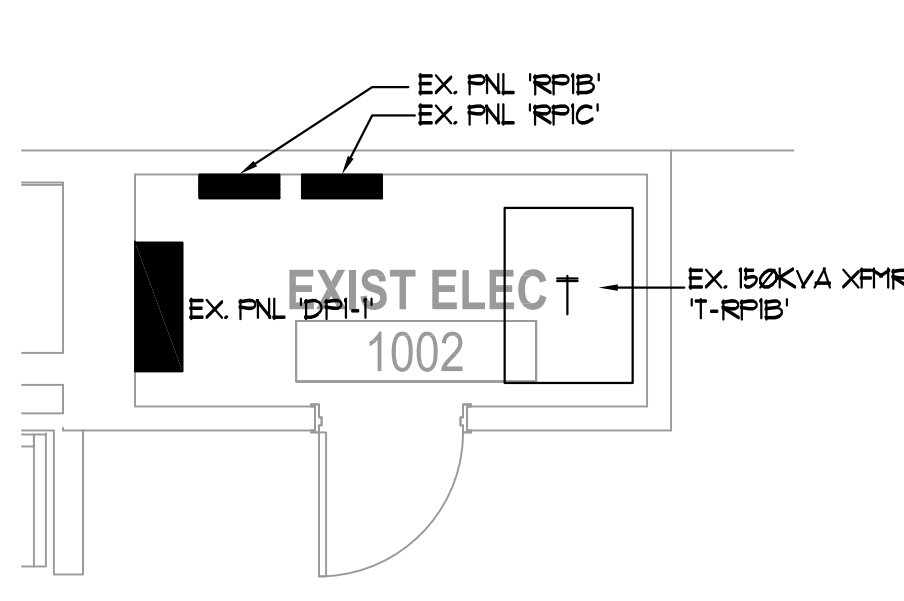
5 PARTIAL PLAN - ELEC RM(1-W) E1.400 1/4"=1'-0"
