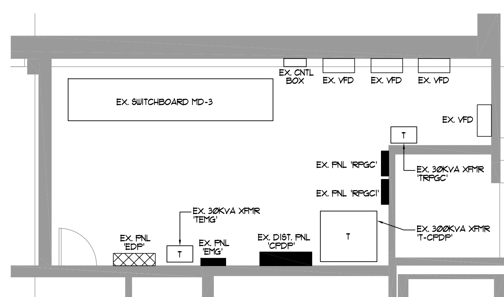
11 PARTIAL PLAN - ELEC RM(G-E) E1.400 1/4"=1'-0"
