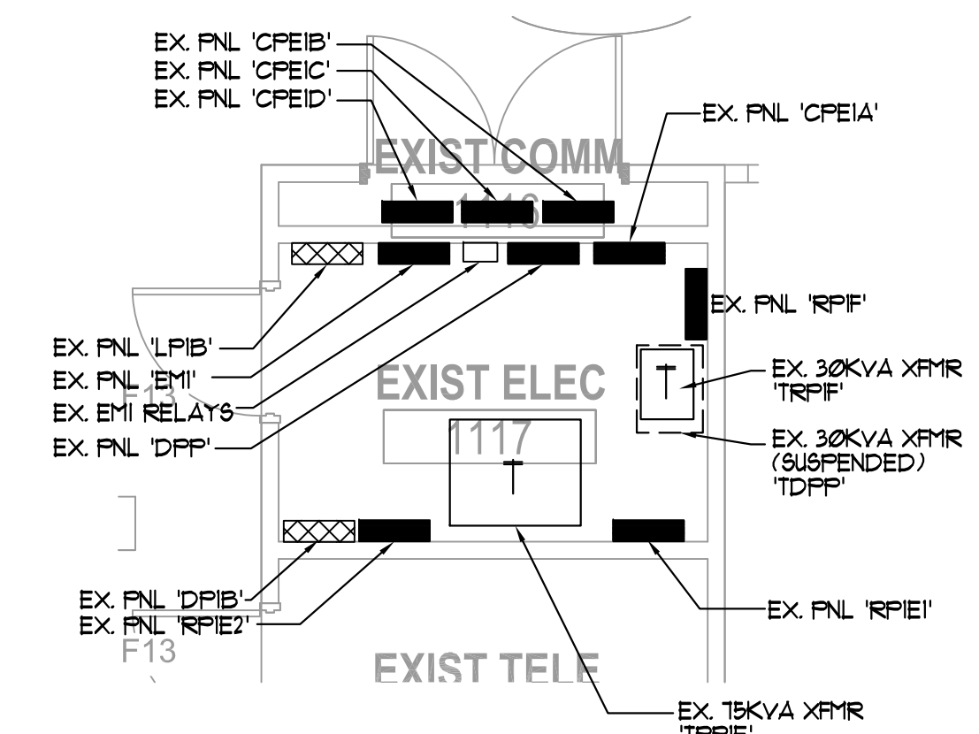
1 PARTIAL PLAN - ELEC RM(1-E) E1.400 1/4"=1'-0"
