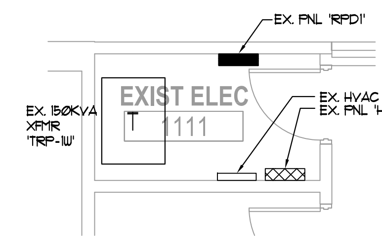
2 PARTIAL PLAN - ELEC RM(1-W) E1.400 1/4"=1'-0"
