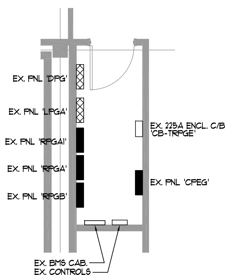
13 PARTIAL PLAN - ELEC RM(G-E) E1.400 1/4"=1'-0"
