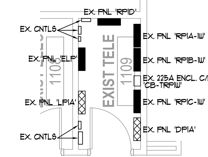
3 PARTIAL PLAN - ELEC RM(1-W) E1.400 1/4"=1'-0"
