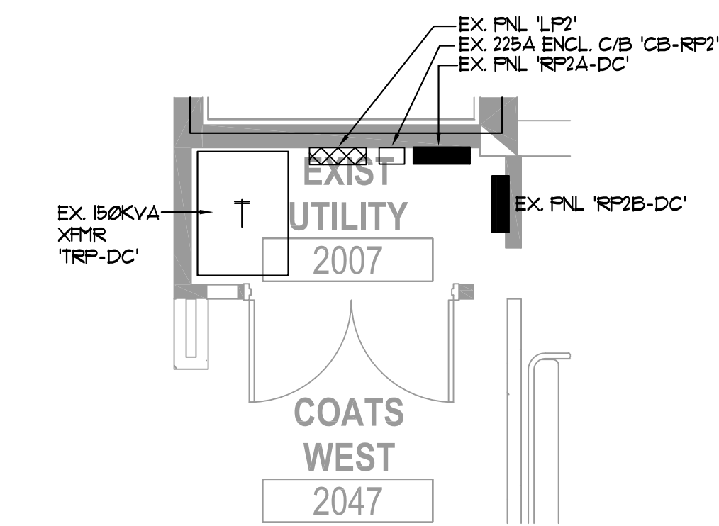
9 PARTIAL PLAN - ELEC RM(2-W) E1.400 1/4"=1'-0"
