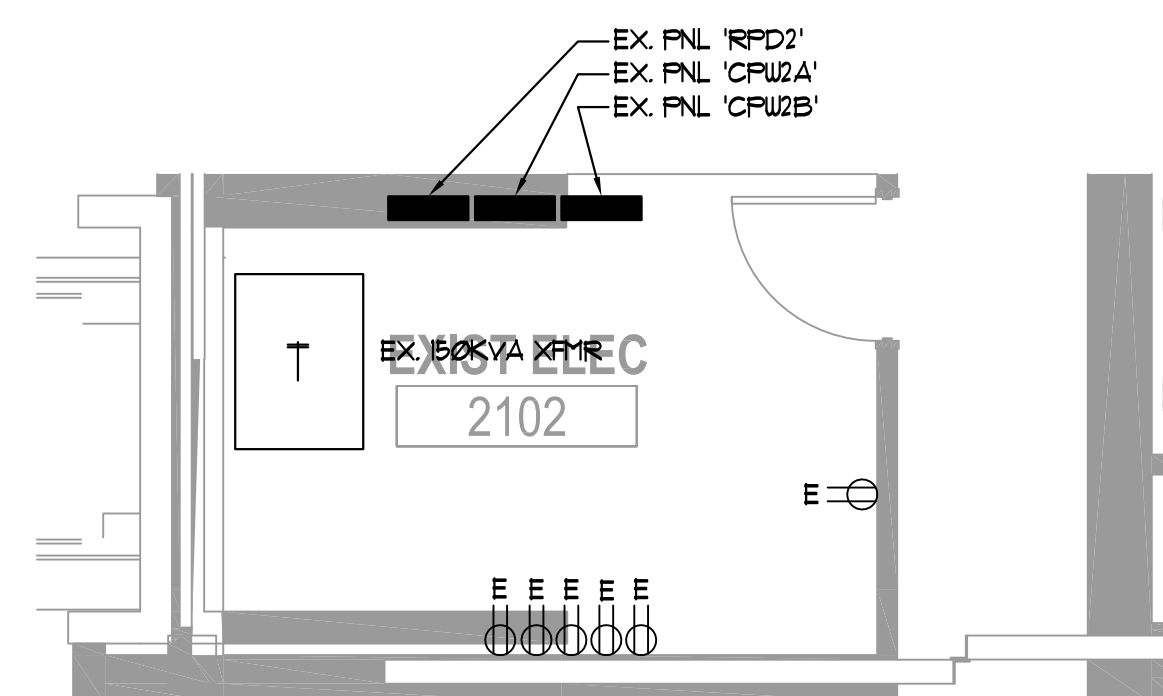
7 PARTIAL PLAN - ELEC RM(2-W) E1.400 1/4"=1'-0"
