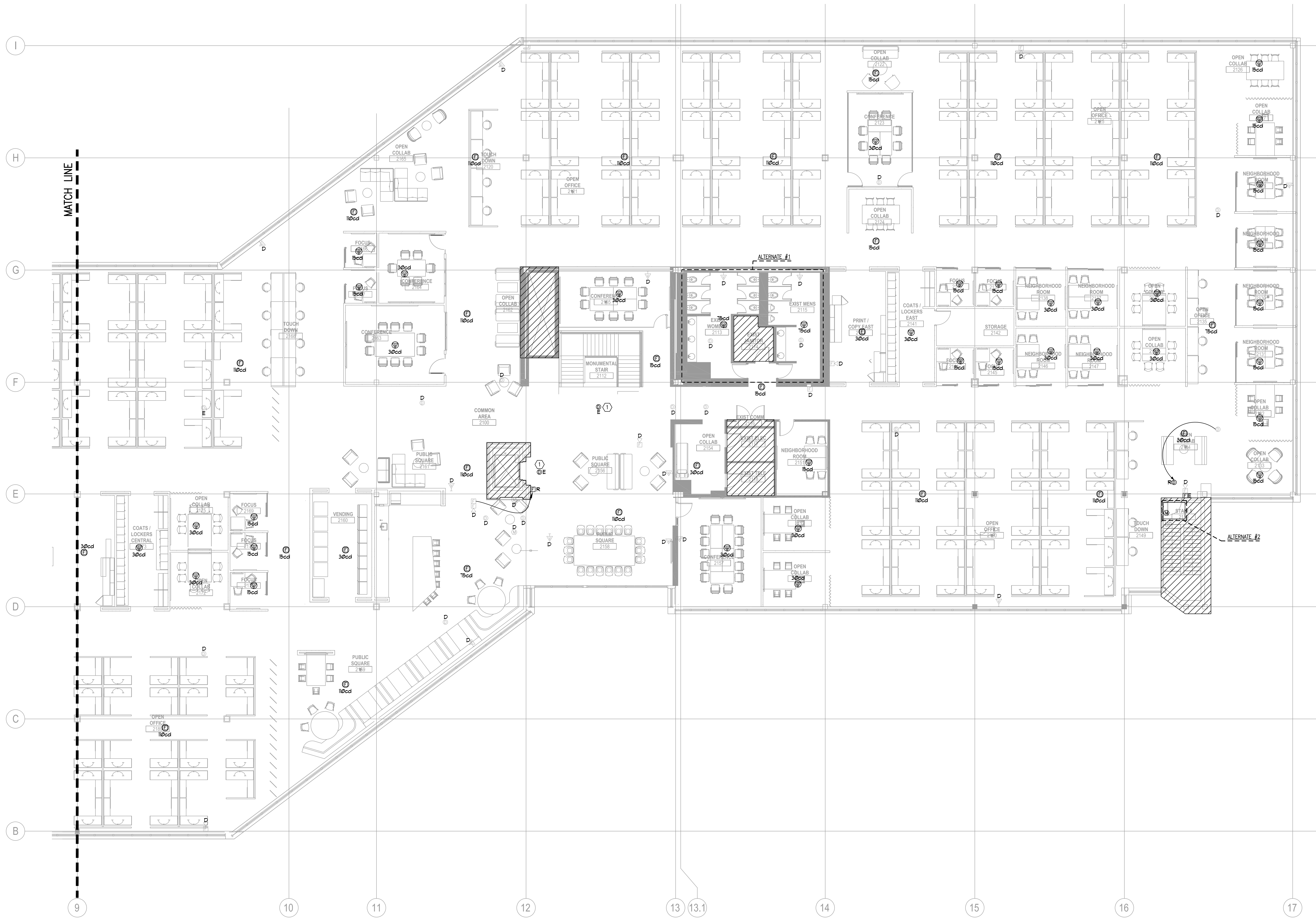
1 2ND FLOOR PLAN (EAST) - FIRE ALARM E1.302E 1/8"=1'-0"
