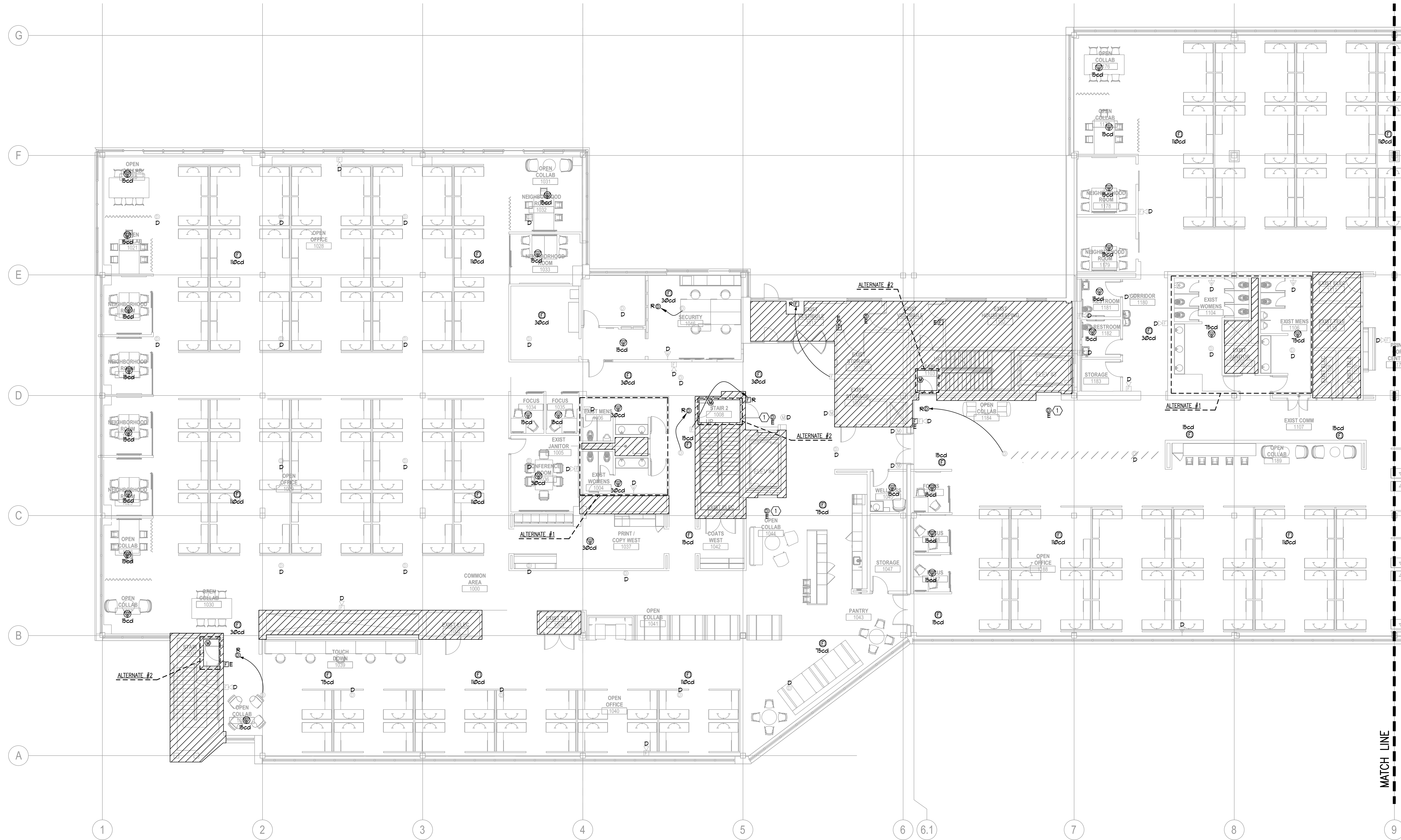
1 1ST FLOOR PLAN (WEST) - FIRE ALARM E1.301W 1/8"=1'-0"
