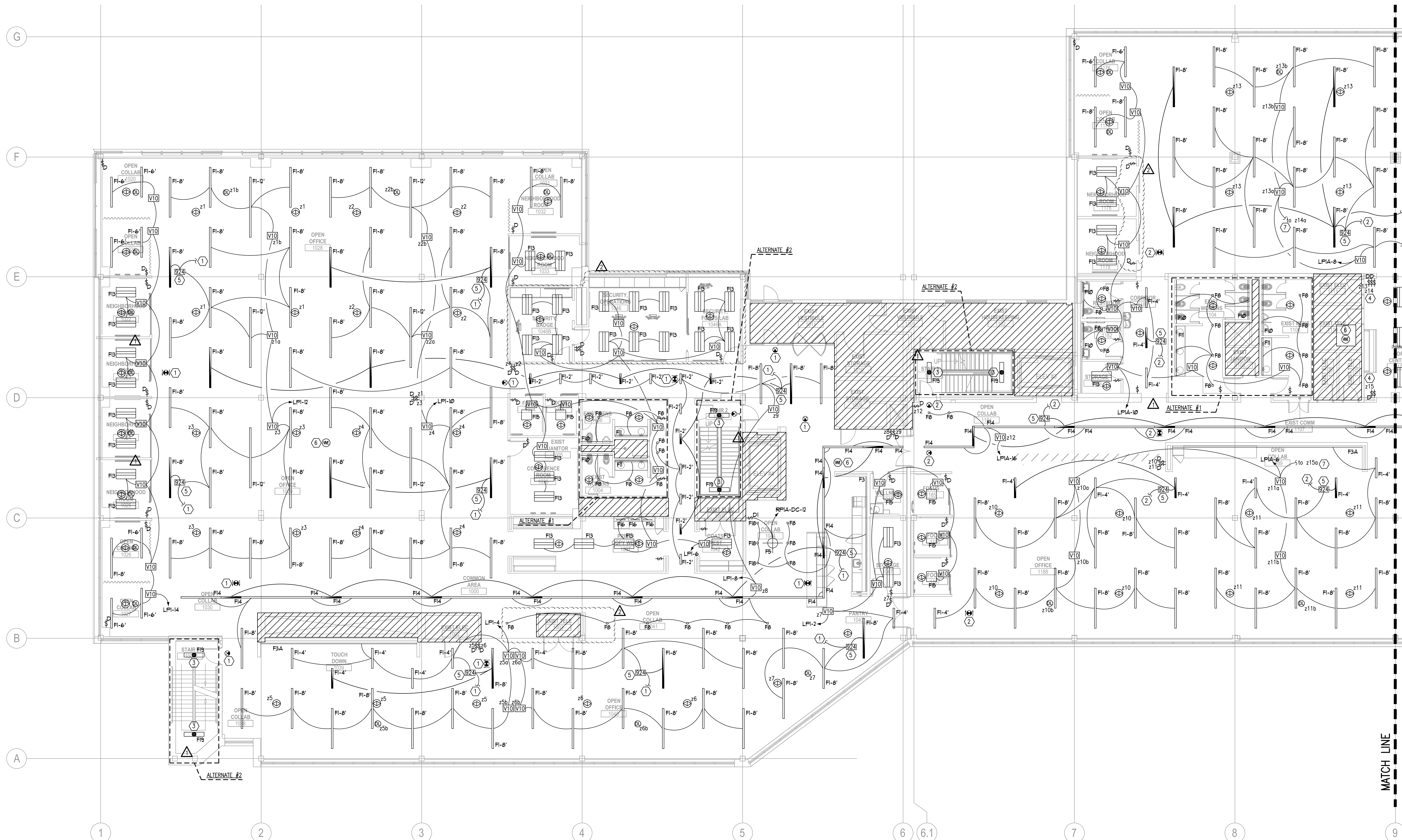
1ST FLOOR PLAN (WEST) - LIGHTING E1.201W 1/8"=1'-0"
