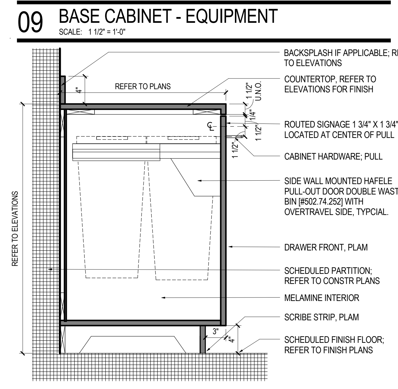
10 BASE CABINET - PULL-OUT TRASH CABINET SCALE: 1 1/2" = 1'-0"
