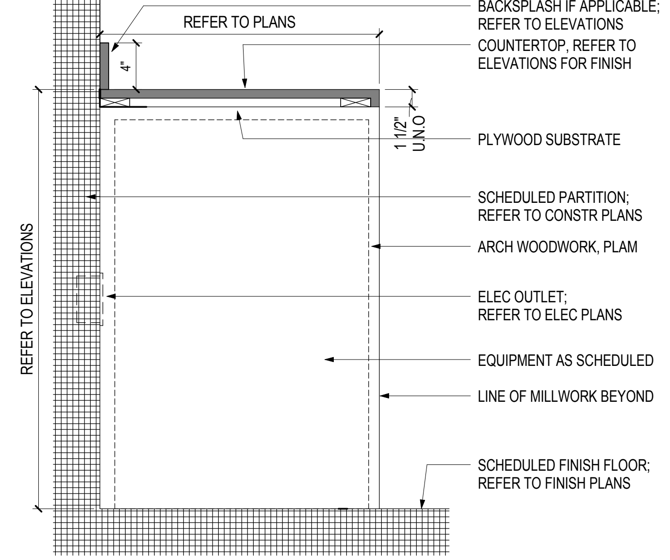
09 BASE CABINET - EQUIPMENT SCALE: 1 1/2" = 1'-0"
