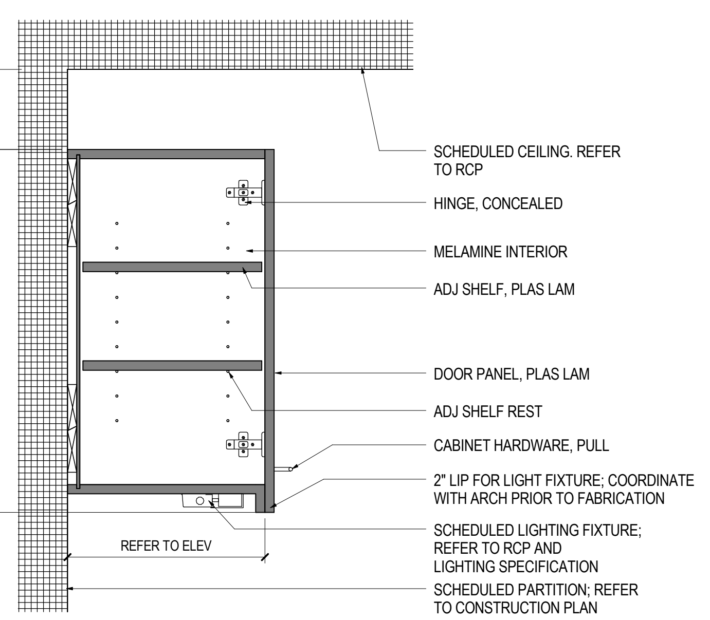
08 DETAIL UPPER CABINET TOP FREE SCALE: 1 1/2" = 1'-0"
