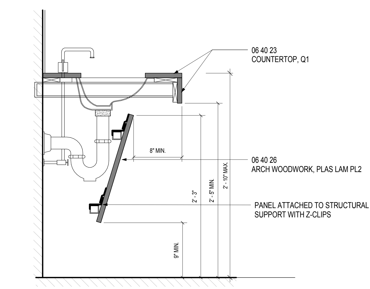
13 LAVATORY COUNTER SCALE: 1 1/2" = 1'-0"
