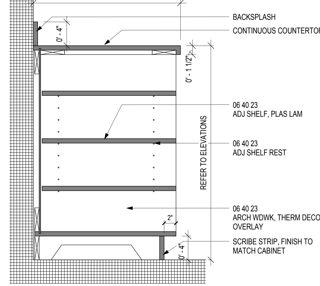
06 BASE CABINET OPEN SHELVING SCALE: 1 1/2" = 1'-0"
