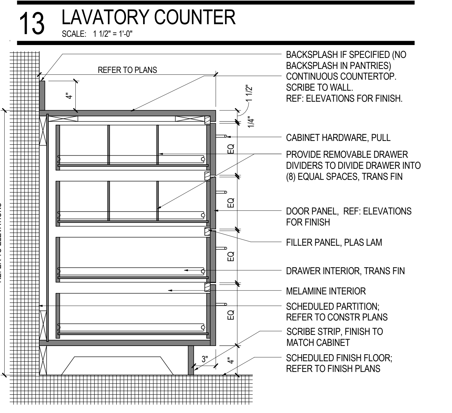
14 DETAIL BASE CABINET WITH DRAWERS (4) SCALE: 1 1/2" = 1'-0"
