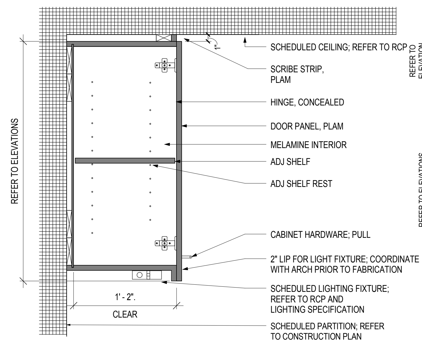
12 UPPER CABINET W/ UNDER LIGHT TO CEILING SCALE: 1 1/2" = 1'-0"
