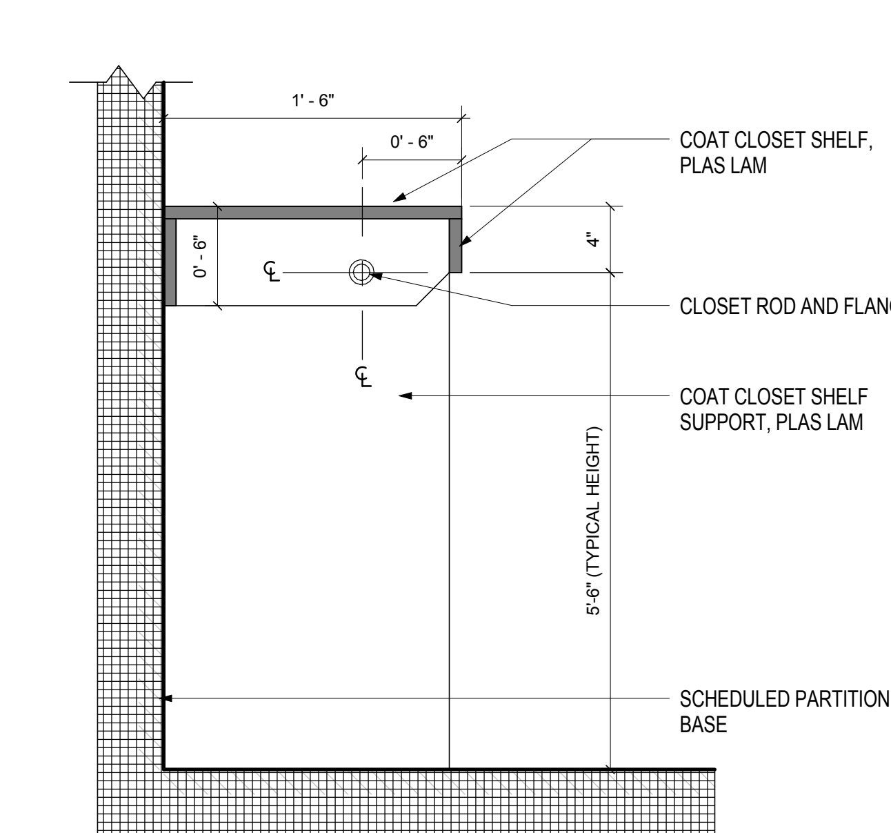
03 CLOSET SHELF AND ROD SCALE: 1 1/2" = 1'-0"
