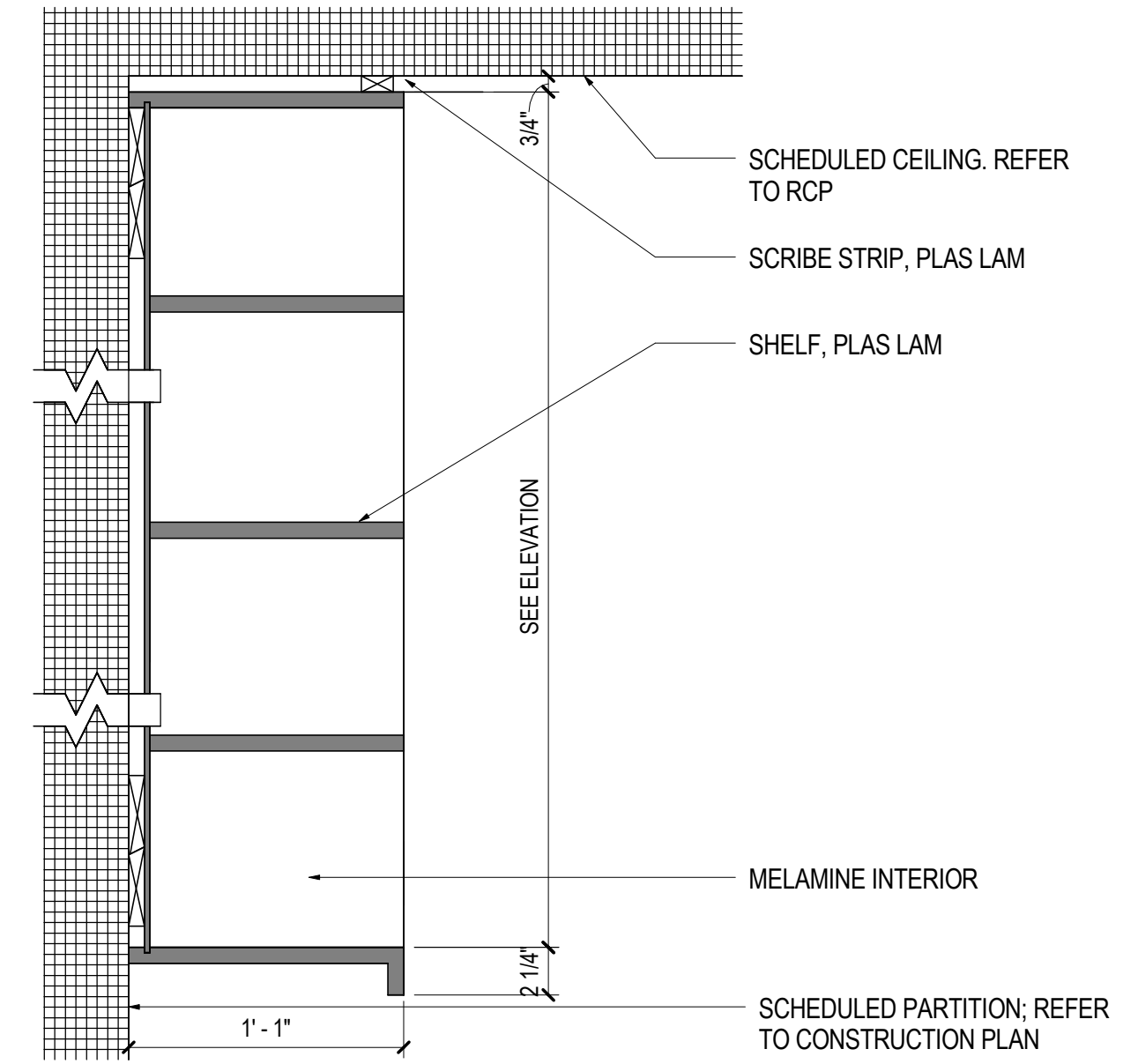
05 DETAIL OPEN SHELVES SCALE: 1 1/2" = 1'-0"
