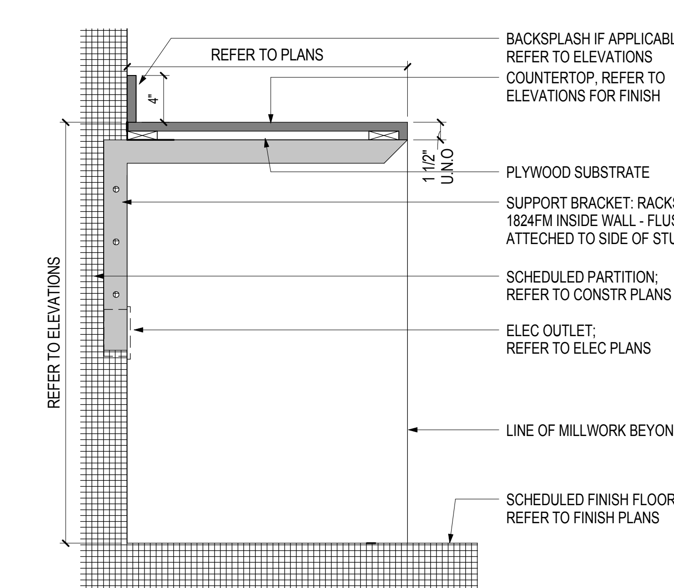
01 BASE COUNTER - OPEN SCALE: 1 1/2" = 1'-0"
