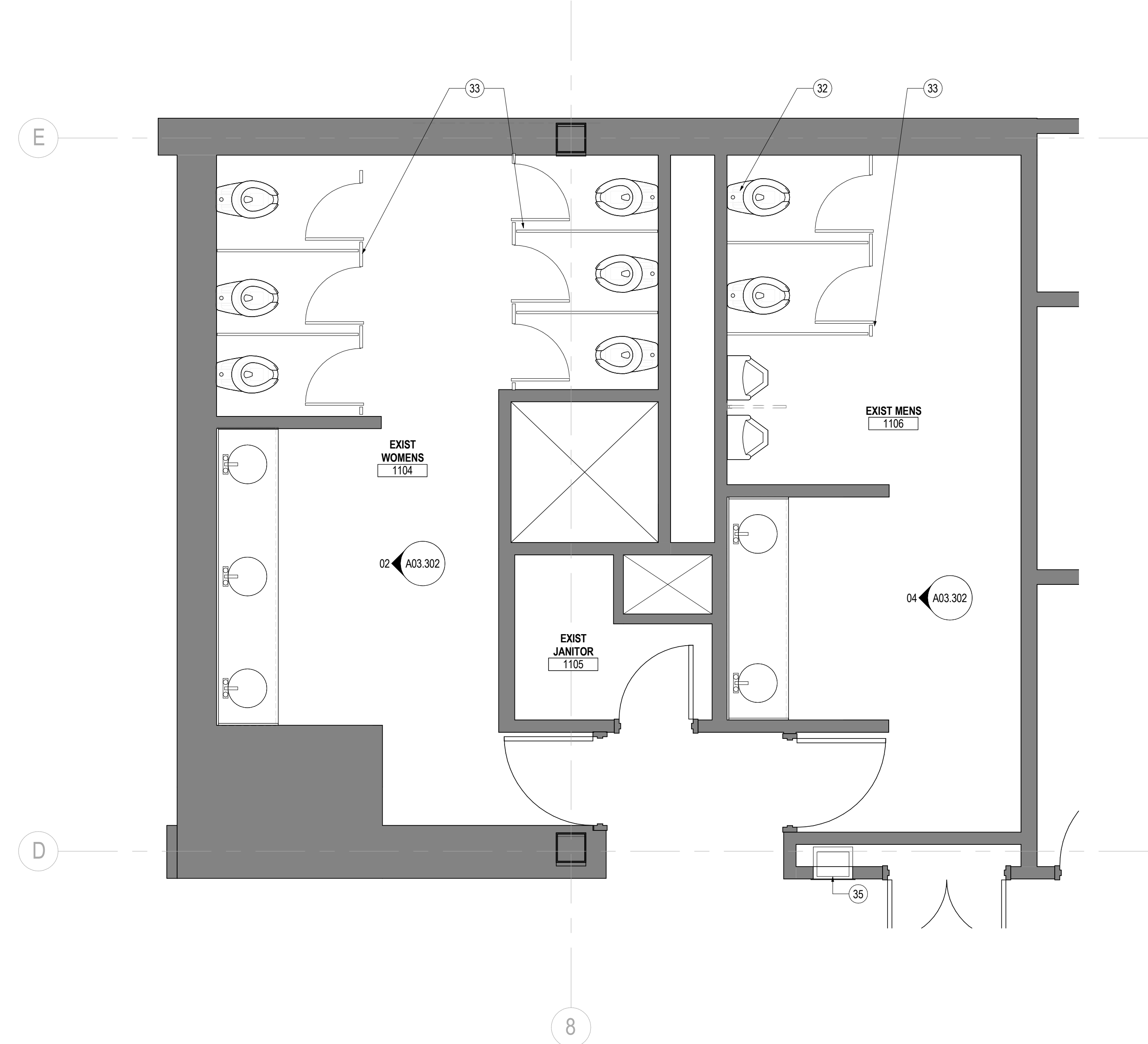
03 ENLARGED PLAN - CENTRAL EXISTING RESTROOM 1104 & 1106 SCALE: 3/8" = 1'-0"
