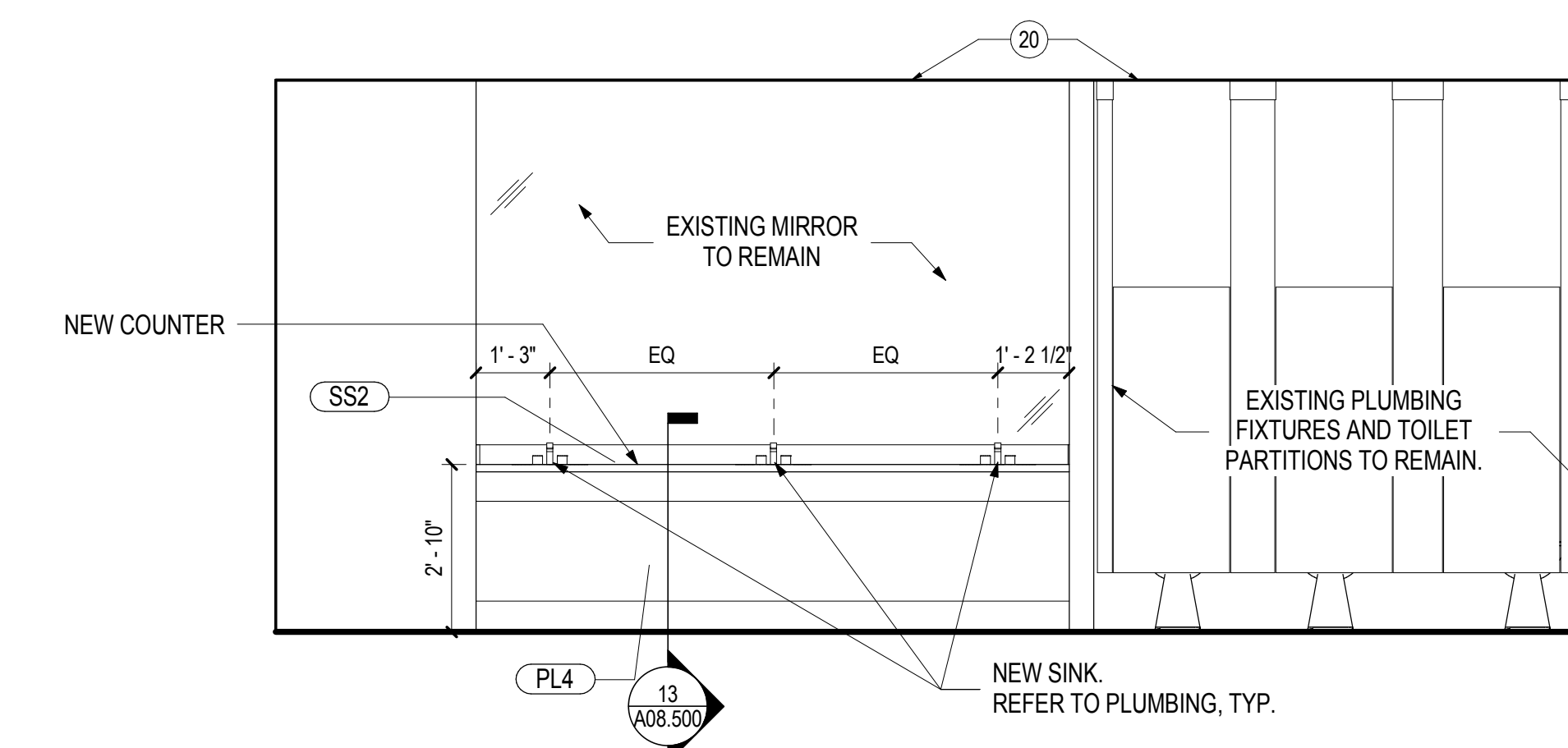
02 1104 & 2104 EXISTING WOMENS - EAST ELEVATION SCALE: 3/8" = 1'-0"
