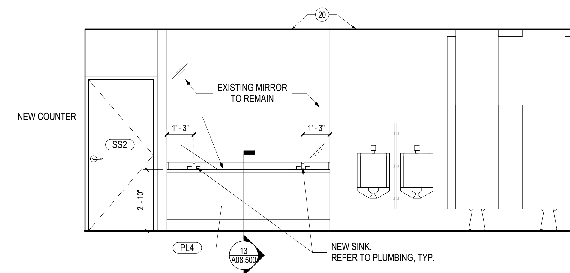
04 1106 & 2106 EXISTING MENS - EAST ELEVATION SCALE: 3/8" = 1'-0"
