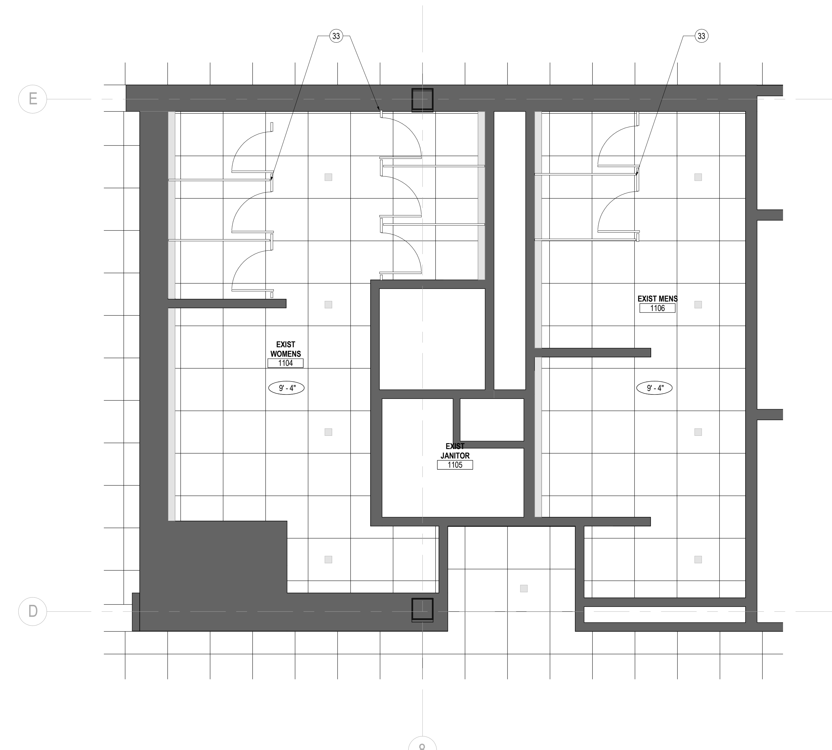
01 ENLARGED RCP - CENTRAL EXISTING RESTROOM 1104 & 1106 SCALE: 3/8" = 1'-0"
