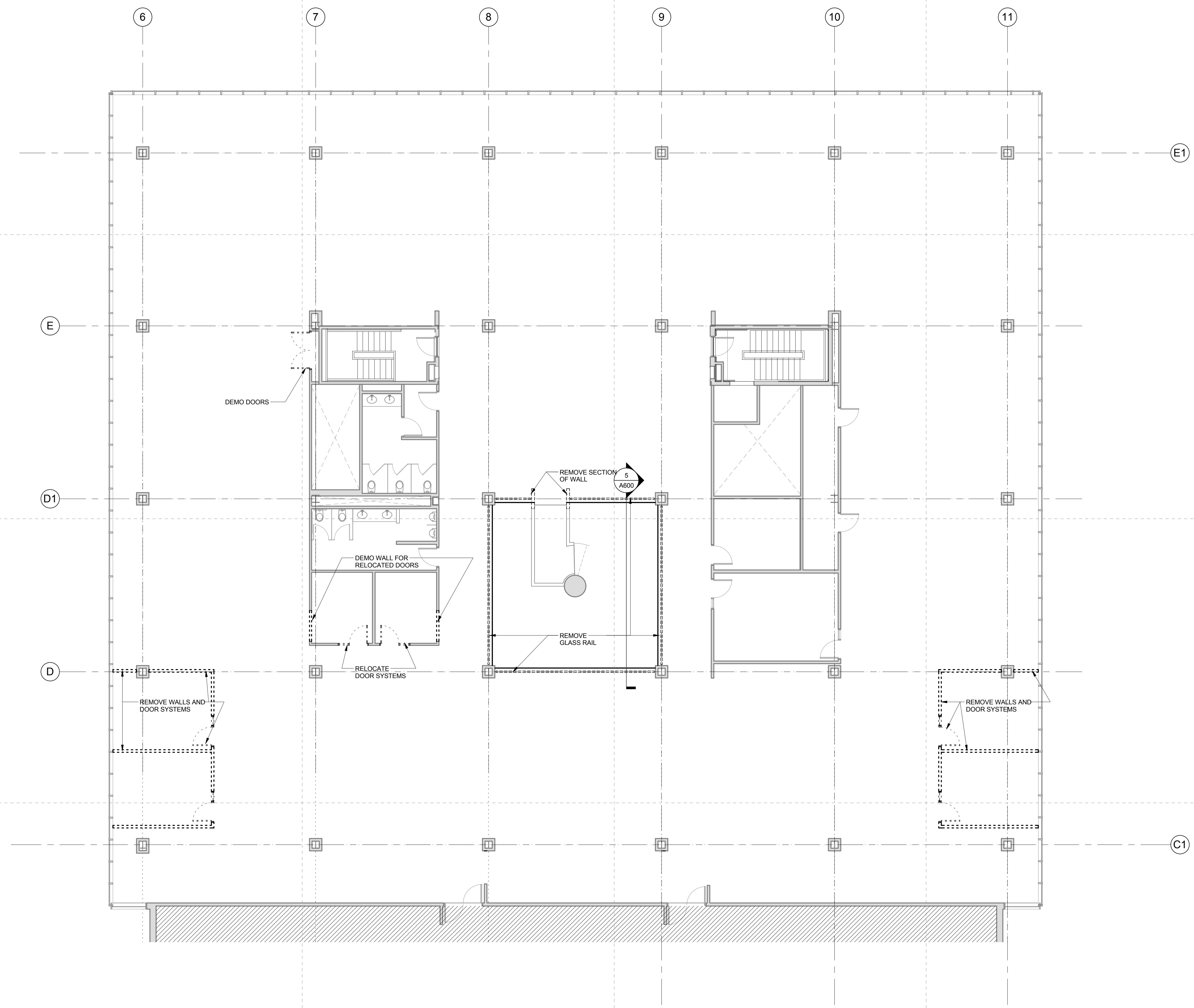
1 THIRD FL. - NORTH WING DEMO PLAN 1/8" = 1'-0"
