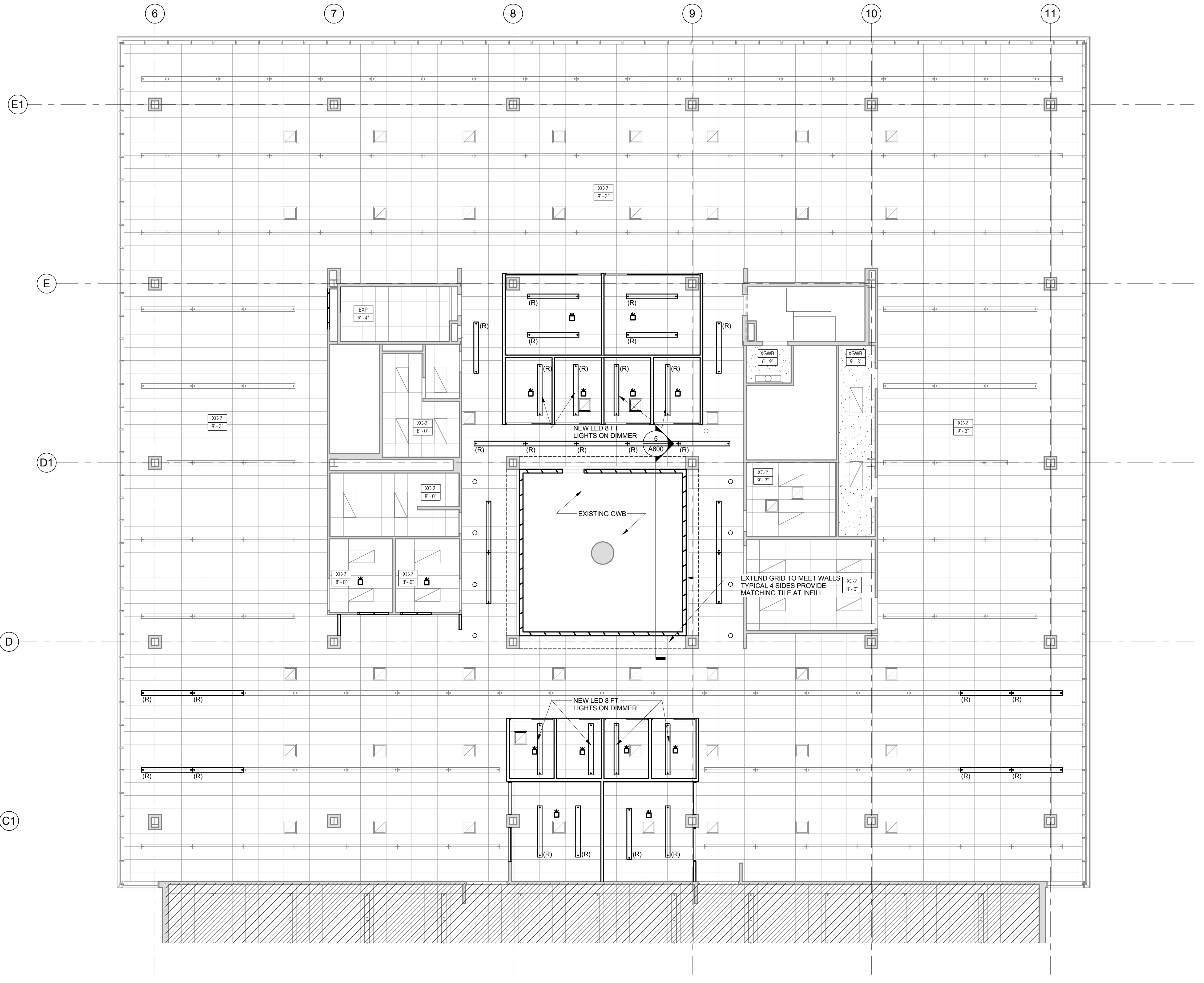
1 THIRD FL. - REFLECTED CEILING PLAN 1/8" = 1'-0"
