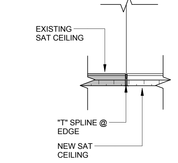
B2 CEILING DETAIL - SAT TO SAT ALIGNED (TYP) 1/2" = 1'-0"
