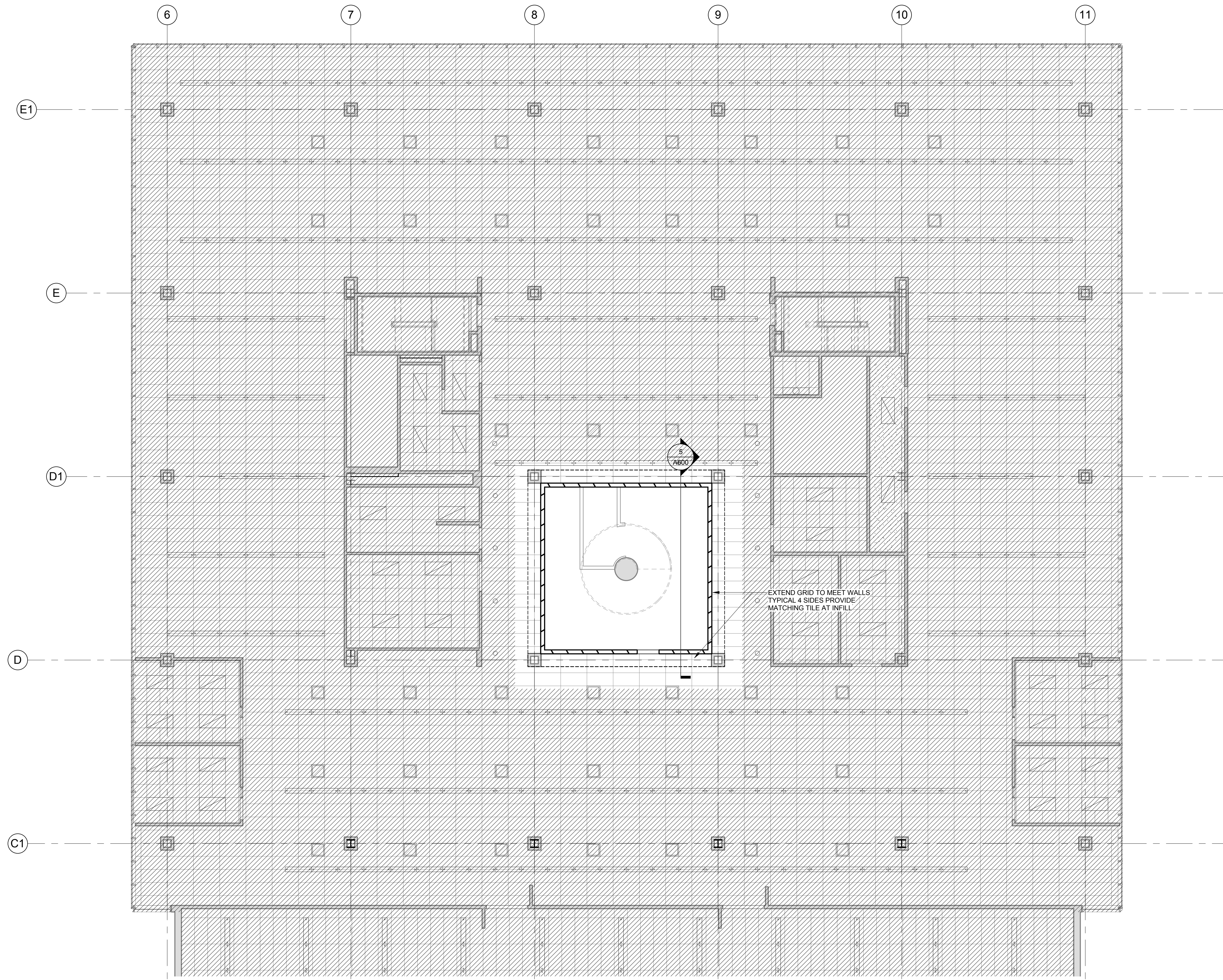
1 SECOND FL. - REFLECTED CEILING PLAN 1/8" = 1'-0"
