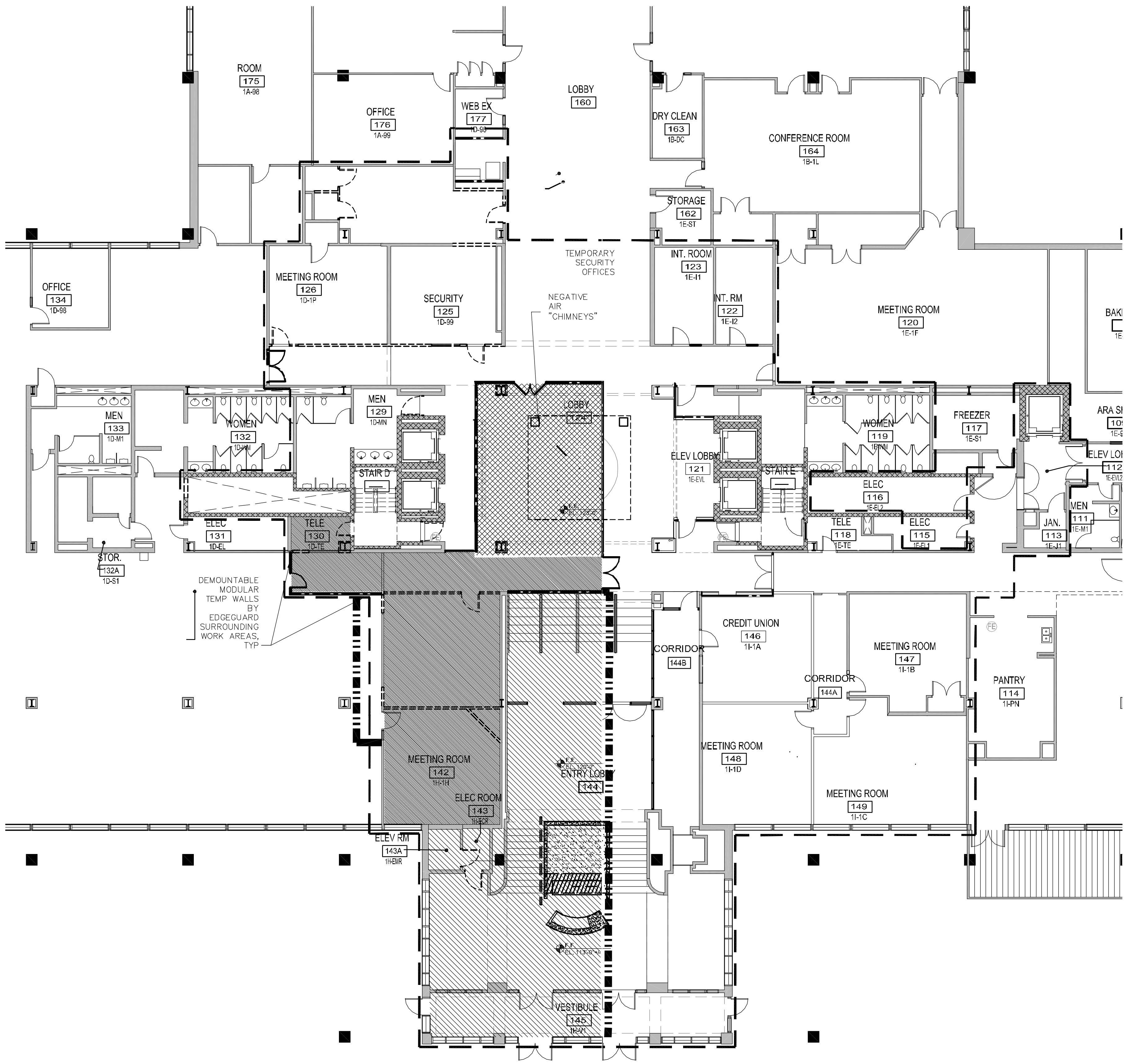
A1 1ST FLOOR CONSTRUCTION PLAN PHASE C 3/32" = 1'-0"
