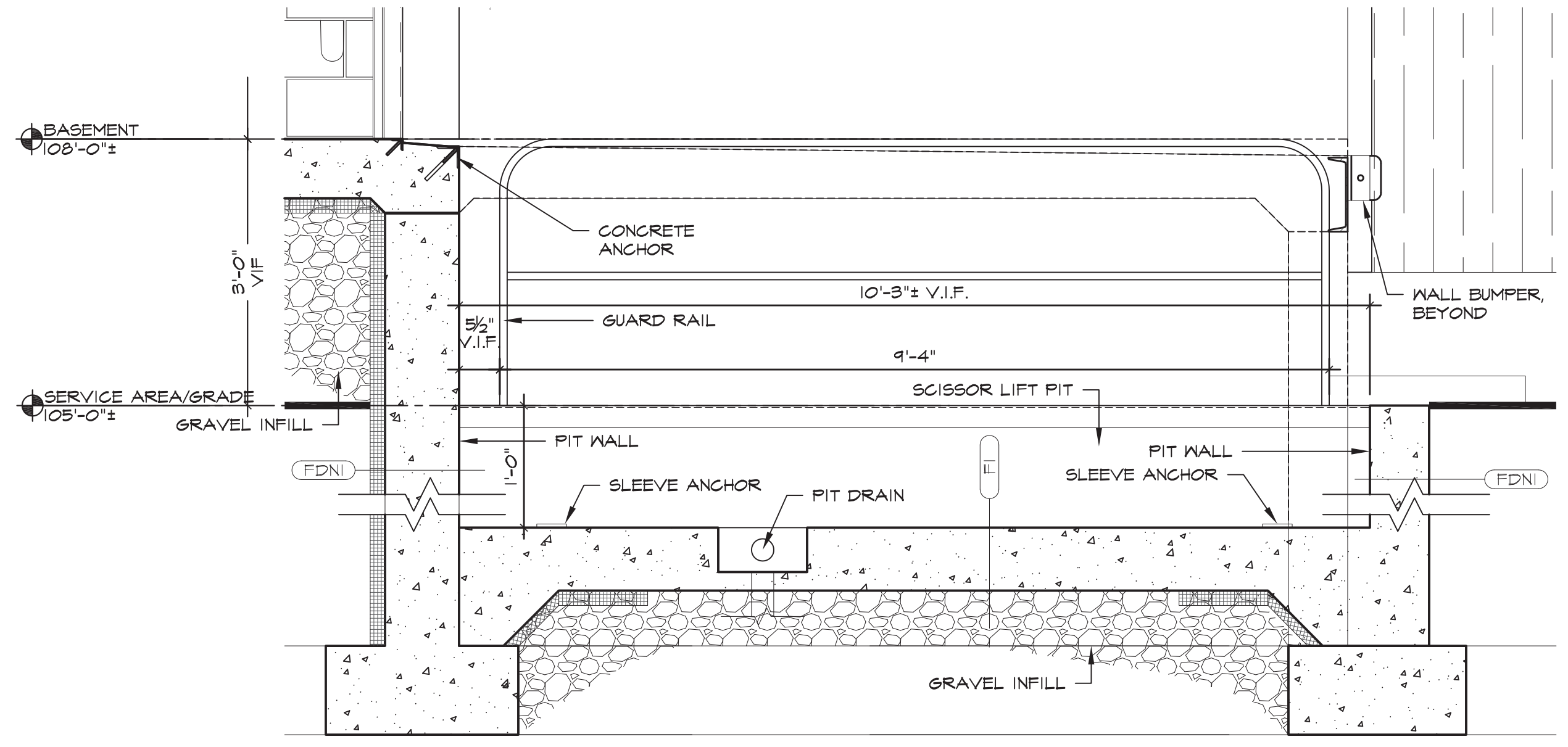
3 TYPICAL DETAIL @ SCISSOR LIFT 3/4" x 1'-0"
