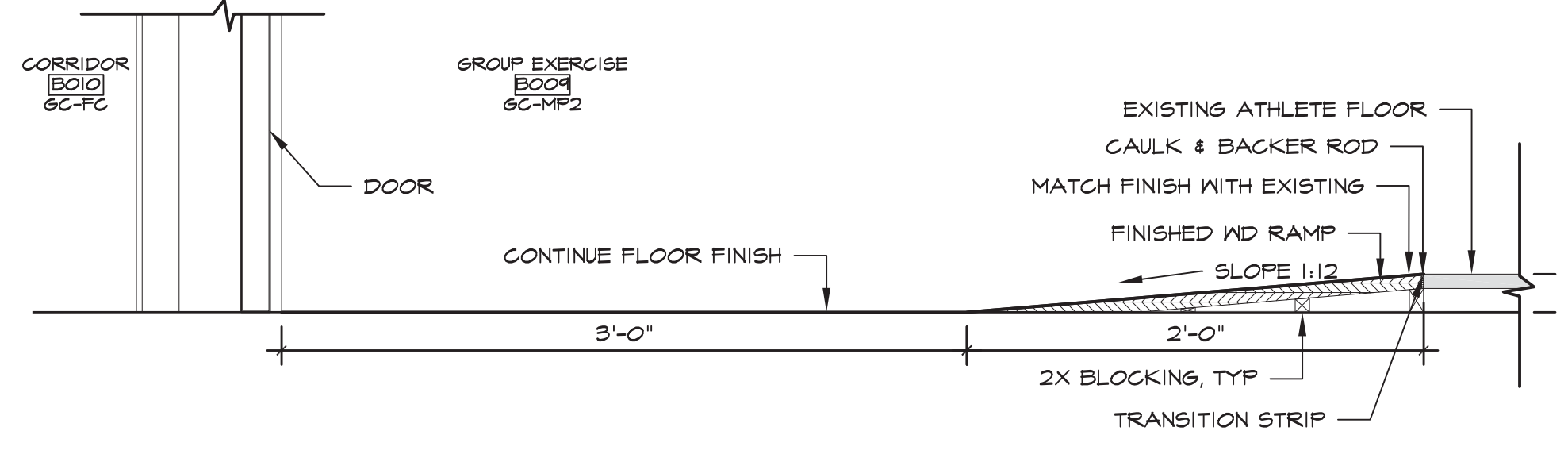
7 RAMP DETAIL 1/2" x 1'-0"
