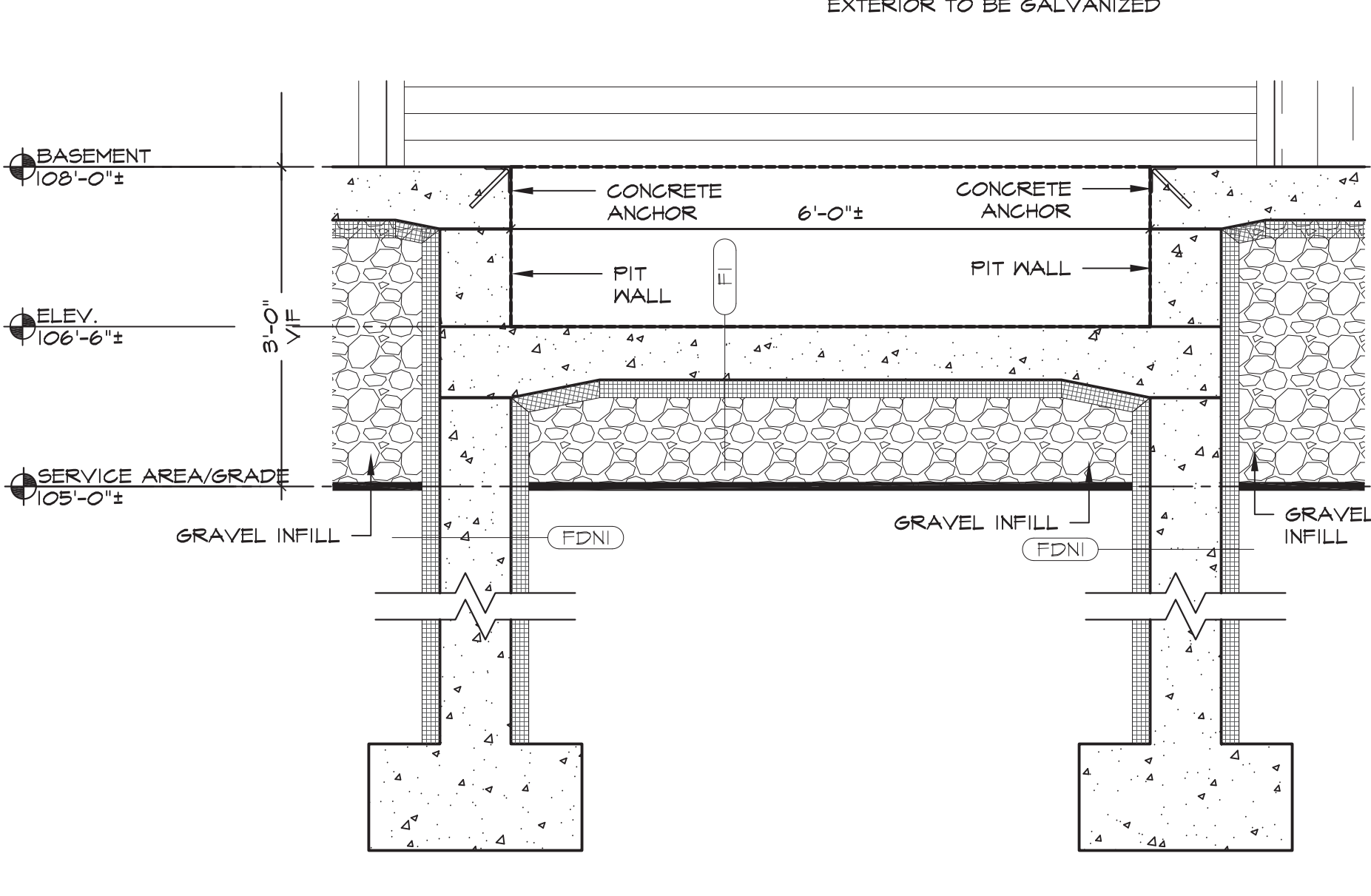
2 TYPICAL DETAIL @ DOCK LEVELER 3/4" x 1'-0"
