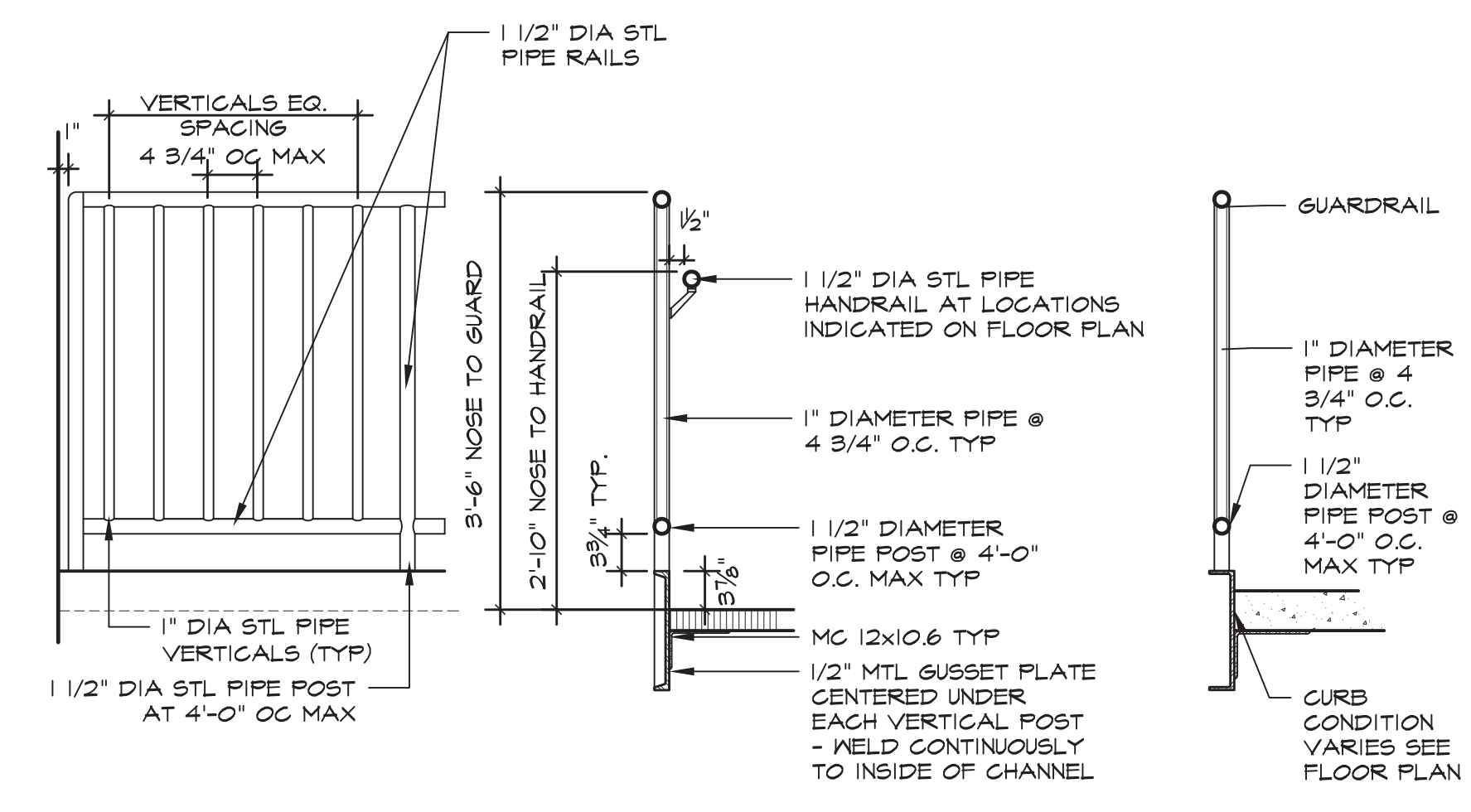
6 GUARDRAIL AND HANDRAIL DETAILS 3/4" x 1'-0" NOTE: EXTERIOR TO BE GALVANIZED
