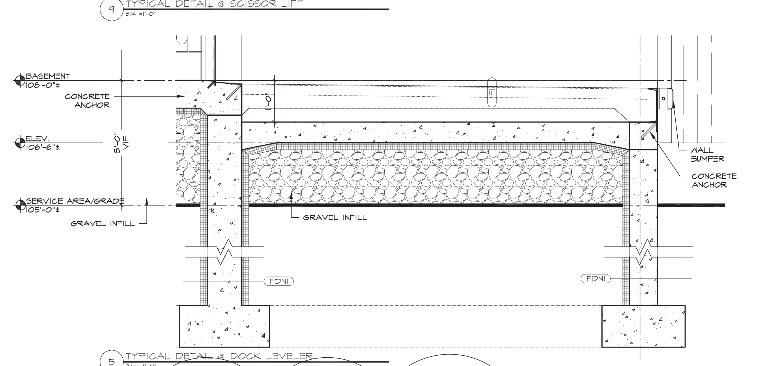
5 TYPICAL DETAIL @ DOCK LEVELER 3/4" x 1'-0"
