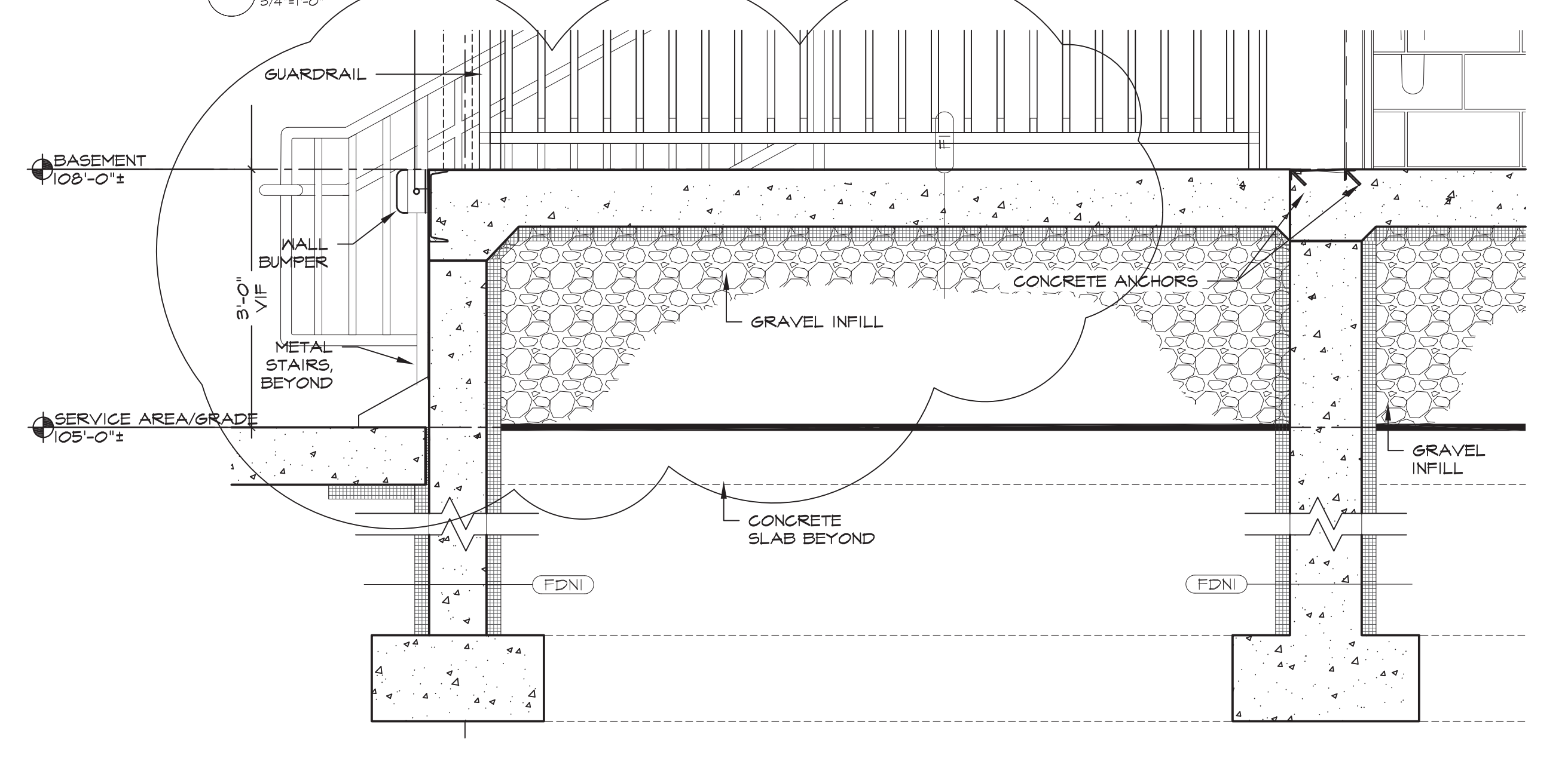
1 TYPICAL DETAIL @ DOCK LEVELER 3/4" x 1'-0"
