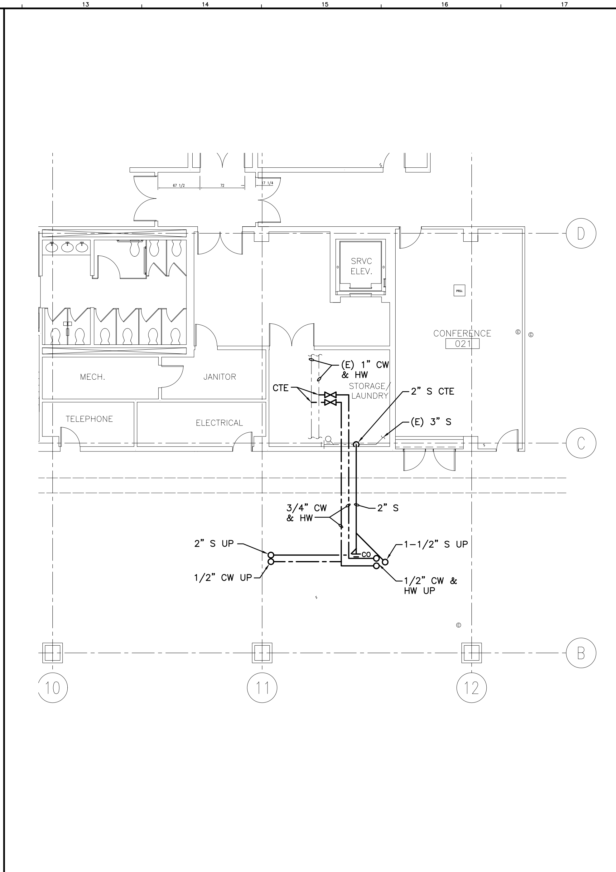
H13 GROUND LEVEL SUPPLY PIPING PLAN 1/8"=1'-0"
