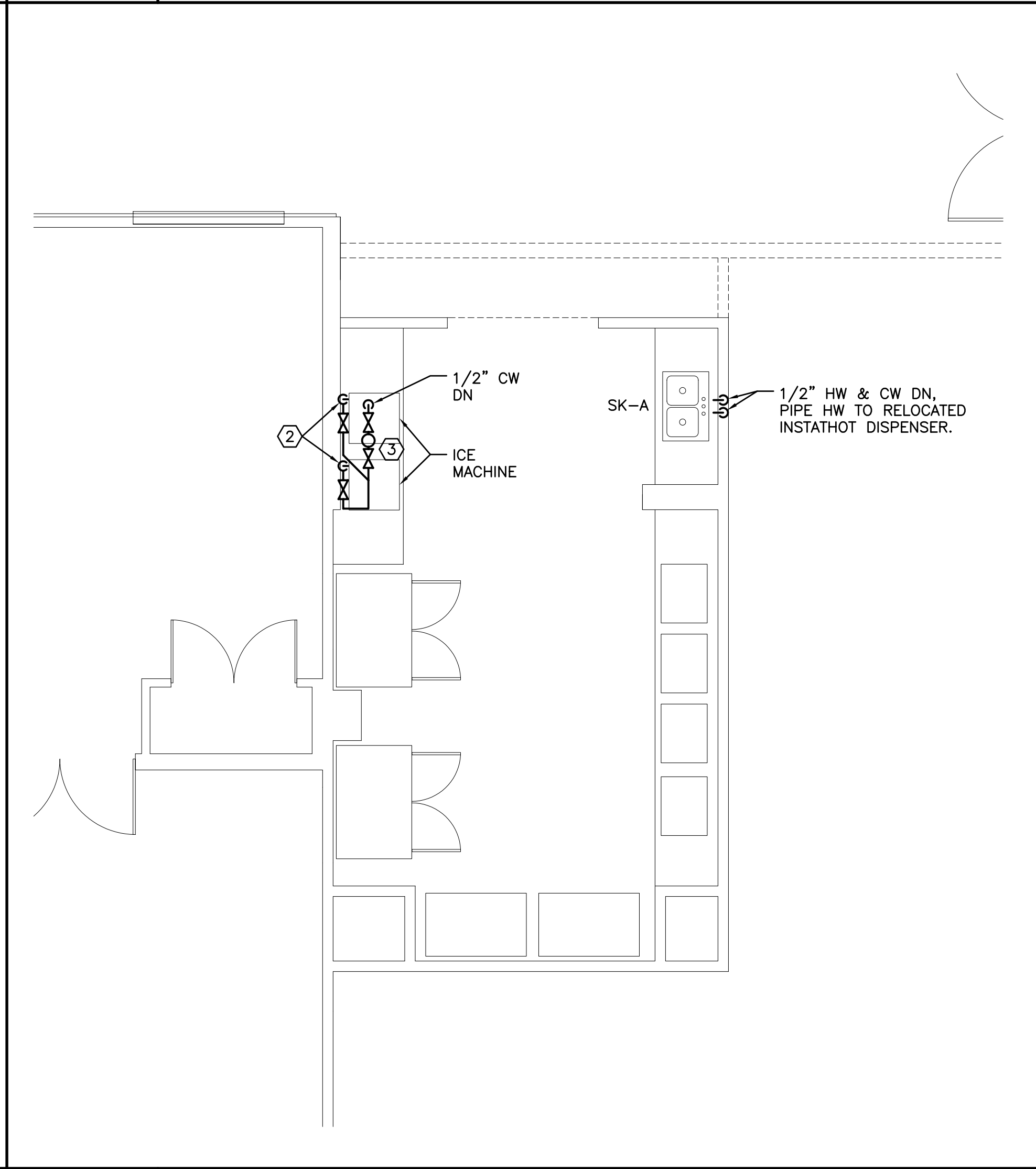
A13 SUPPLY PIPING PLAN 1/4"=1'-0"
