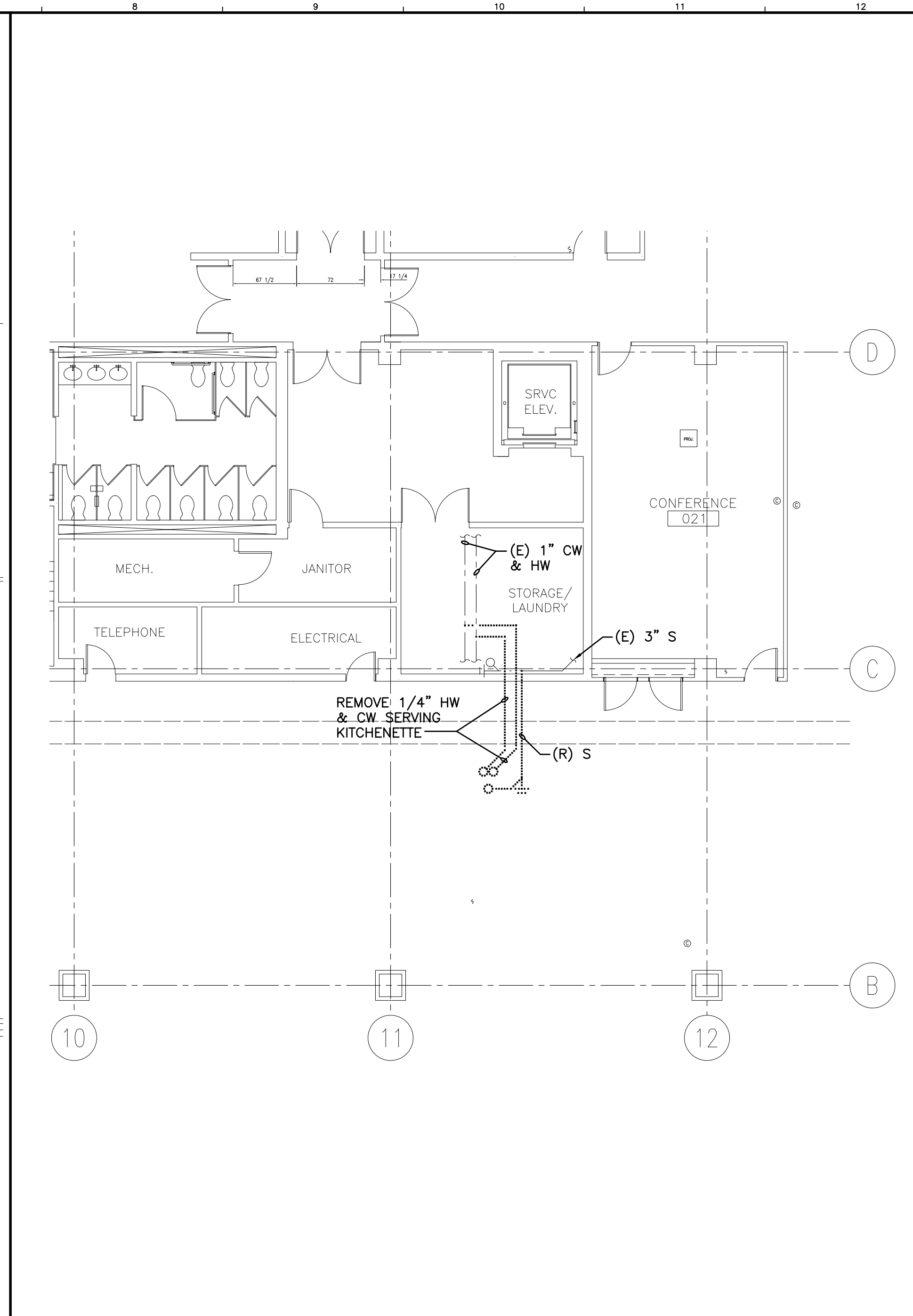
H7 GROUND LEVEL DEMOLITION PLAN 1/8"=1'-0"
