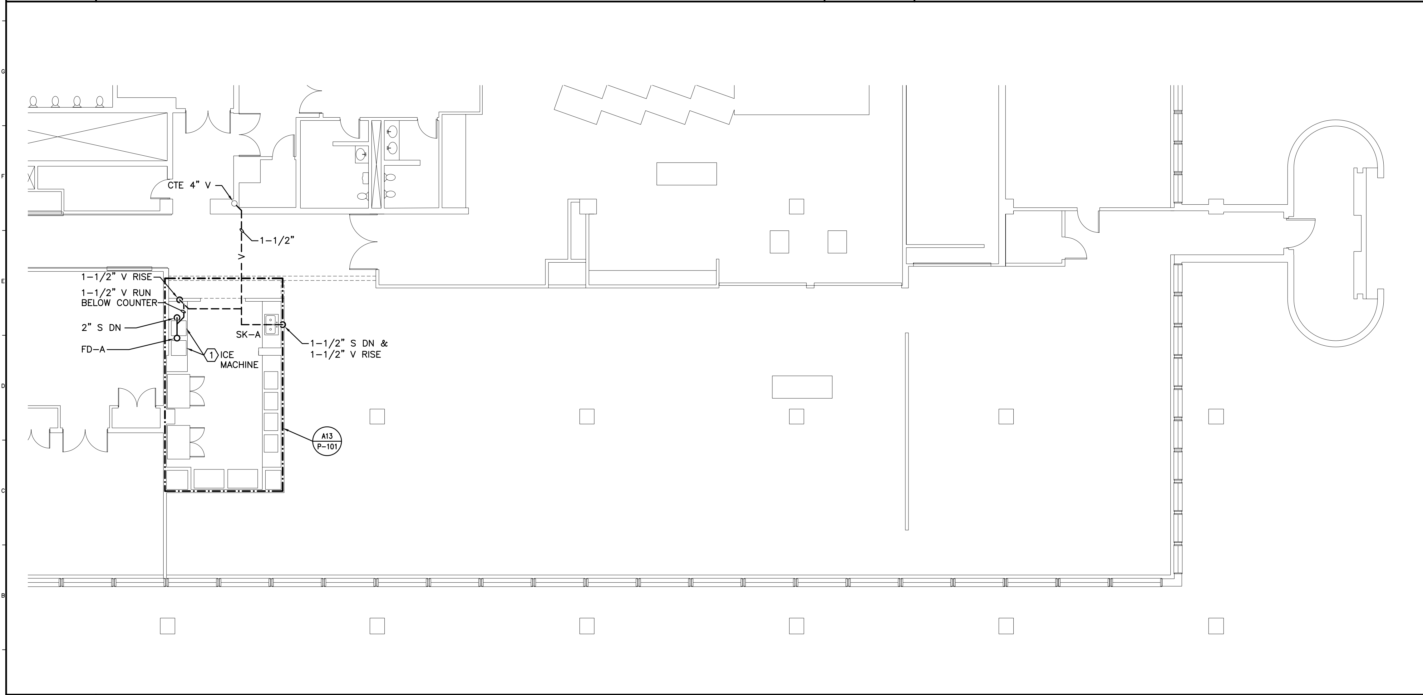
A1 DWV PIPING PLAN 1/8"=1'-0"
