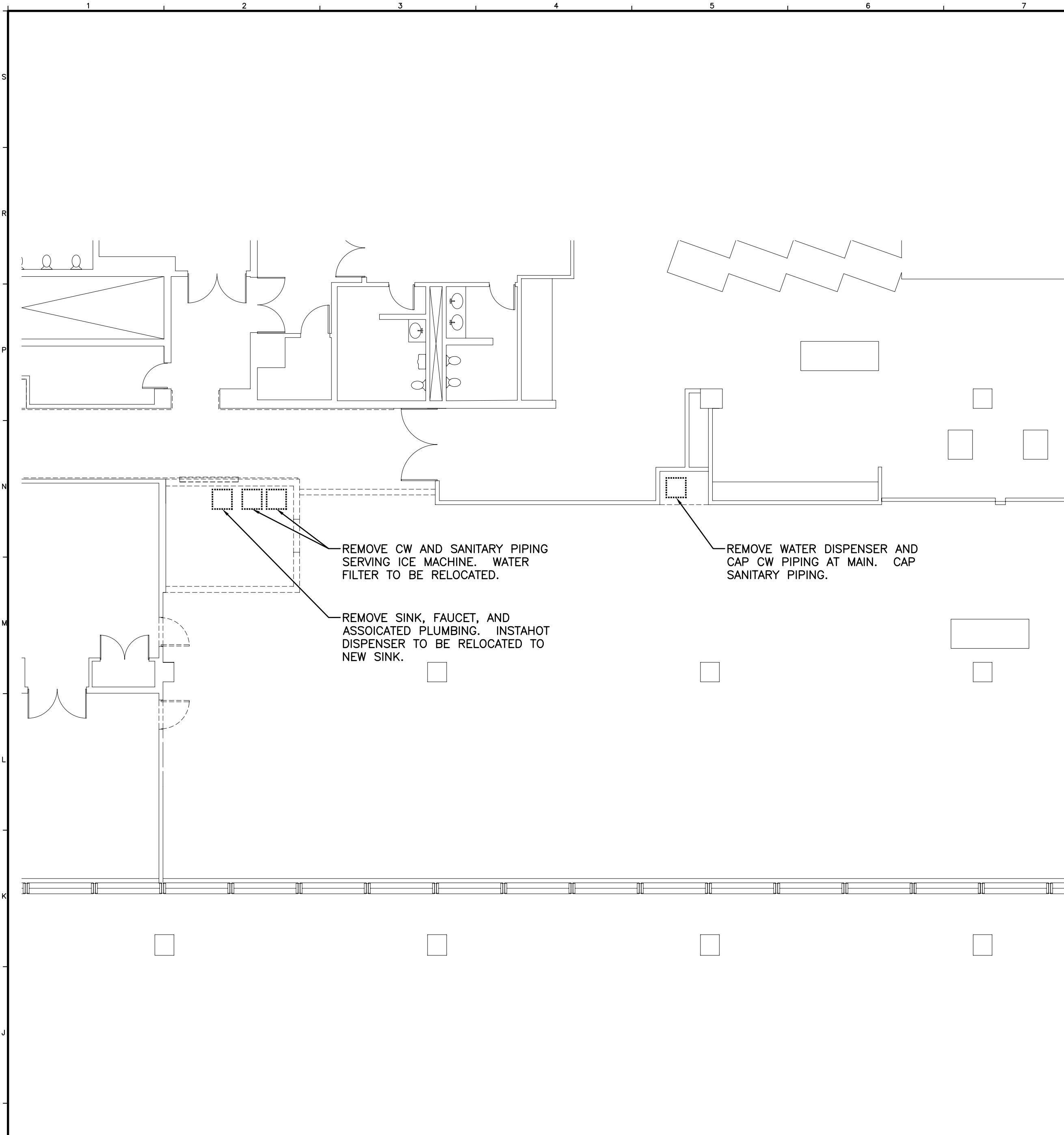
H1 DEMOLITION PLAN 1/8"=1'-0"
