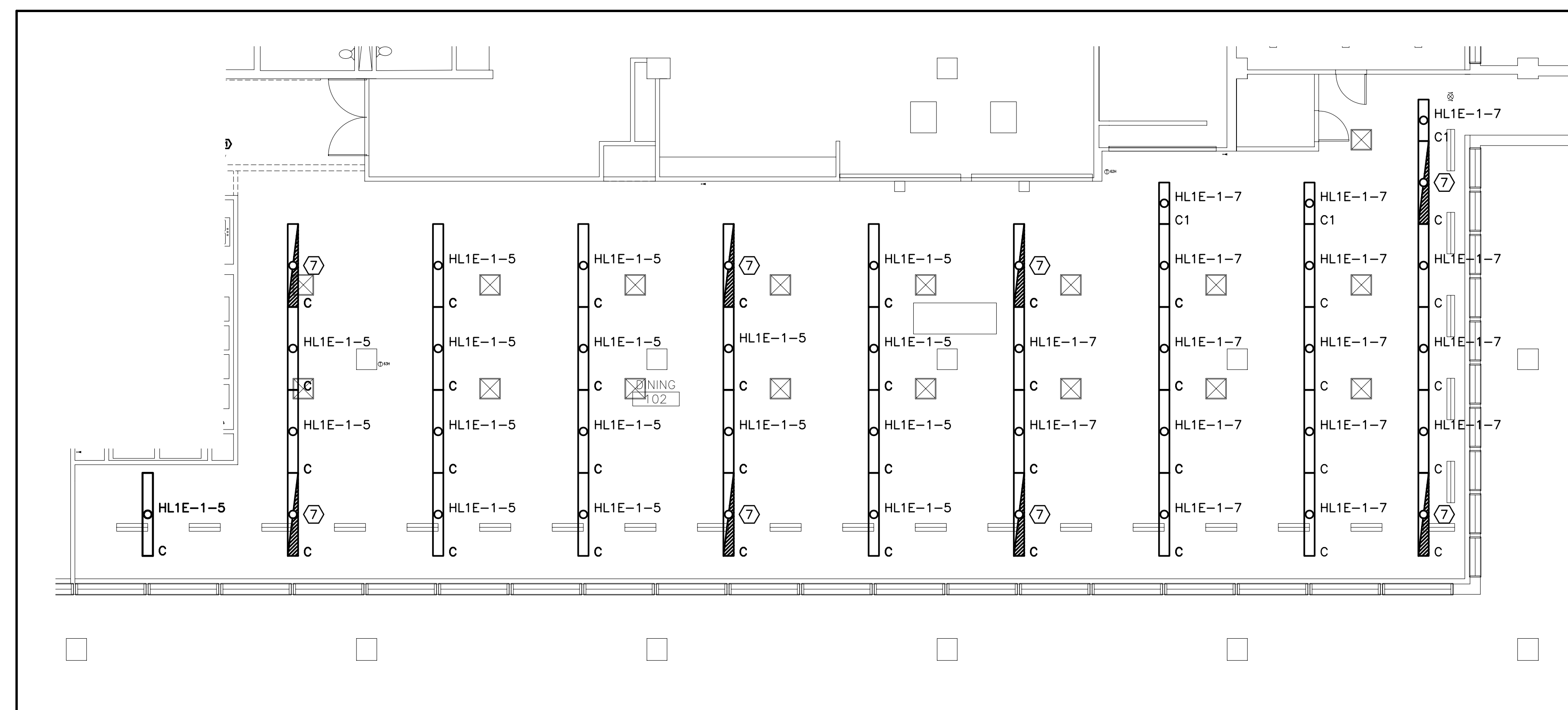
J1 DINING 102 LIGHTING PLAN 1/8"=1'-0"
