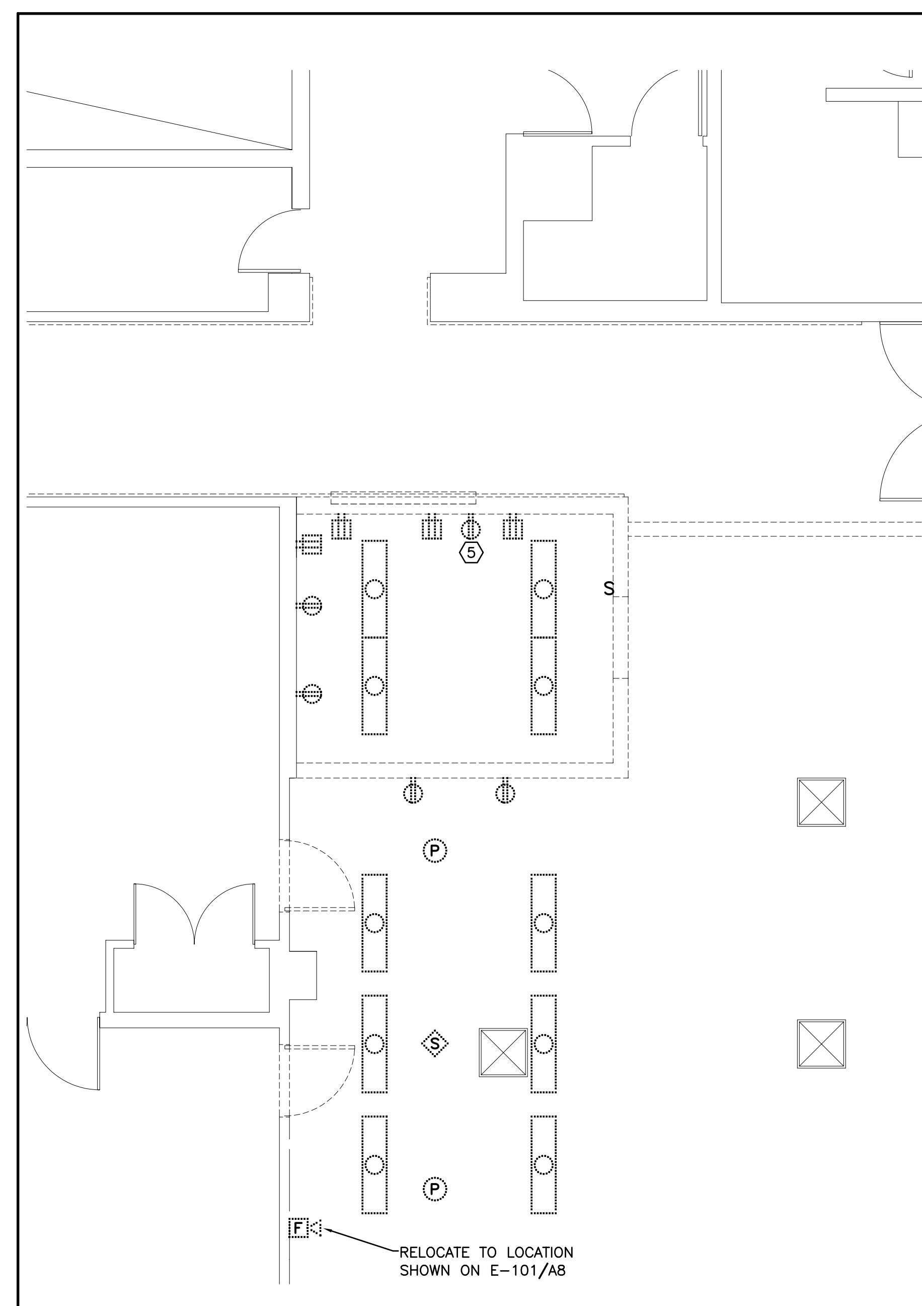
A1 DEMOLITION PLAN 1/4"=1'-0"
