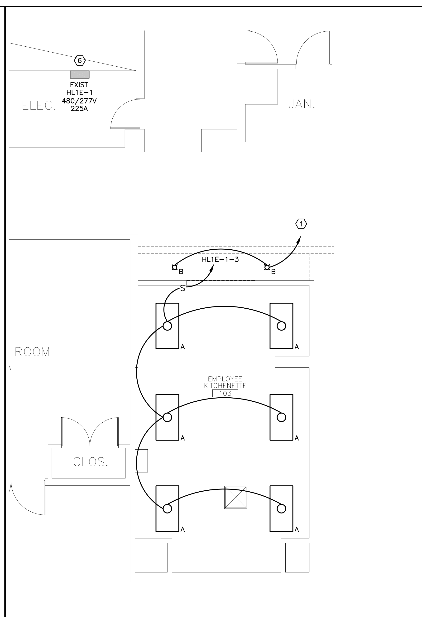
A13 EMPLOYEE KITCHENETTE 103 LIGHTING PLAN 1/4"=1'-0"
