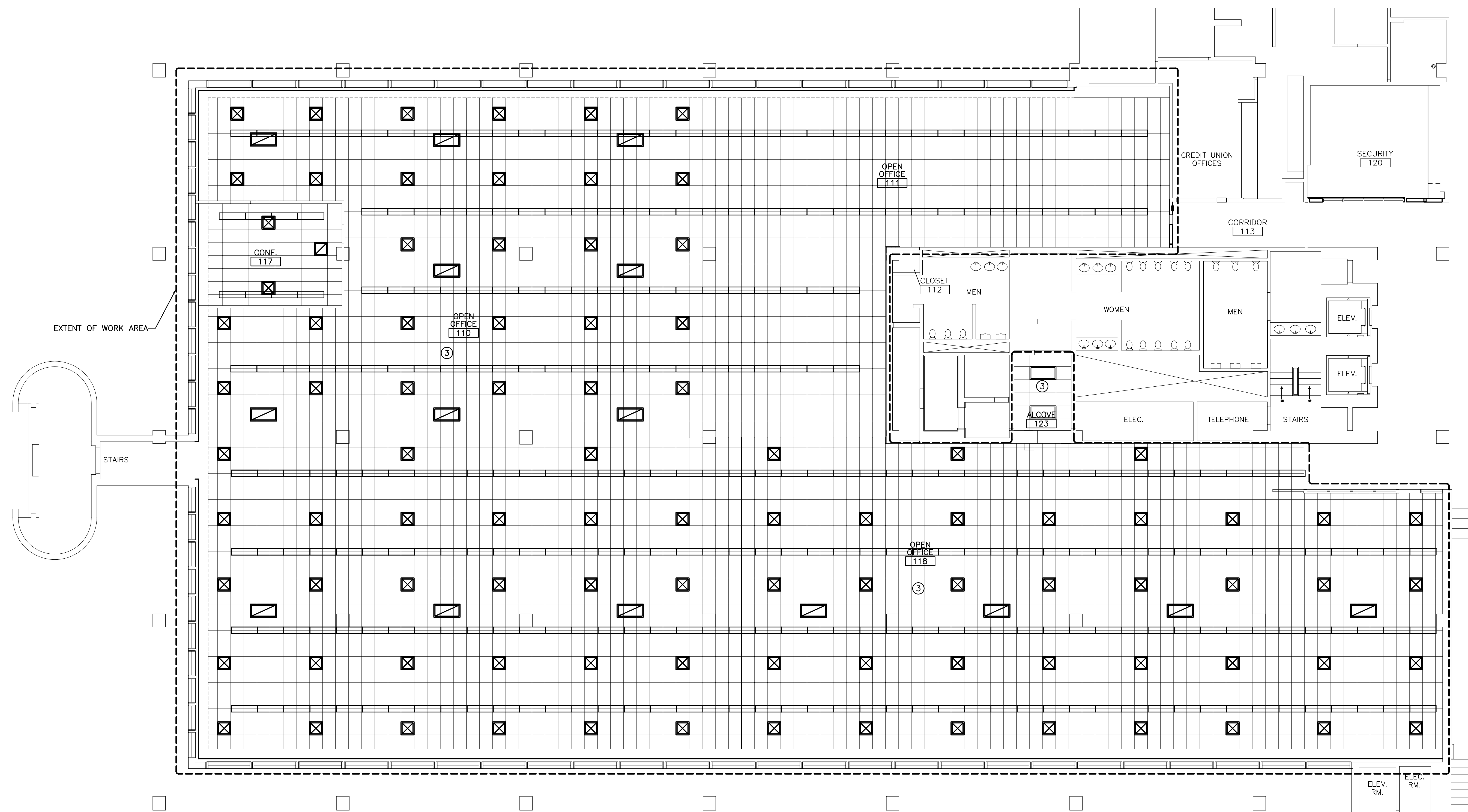
A1 ALTERNATE REFLECTED CEILING PLAN 1/8"=1'-0"
