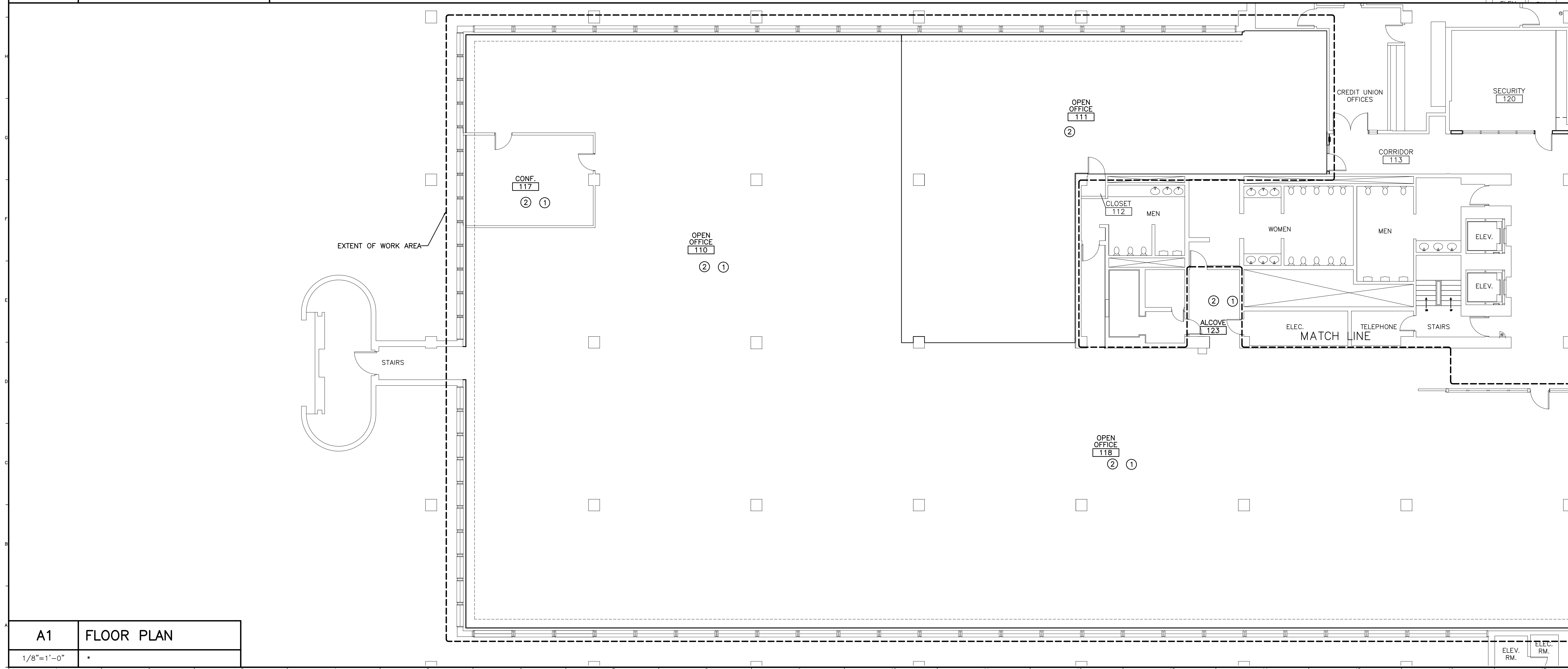
A9 REFLECTED CEILING PLAN 1/8"=1'-0"
