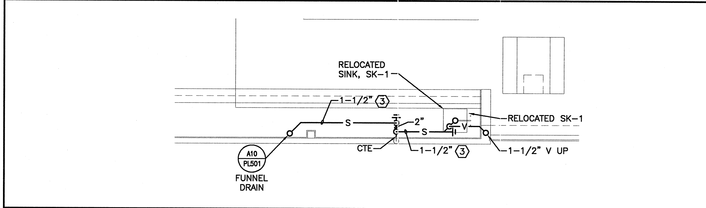
C7 BEVERAGE AREA DWV PIPING PART PLAN 1/4"=1'-0"
