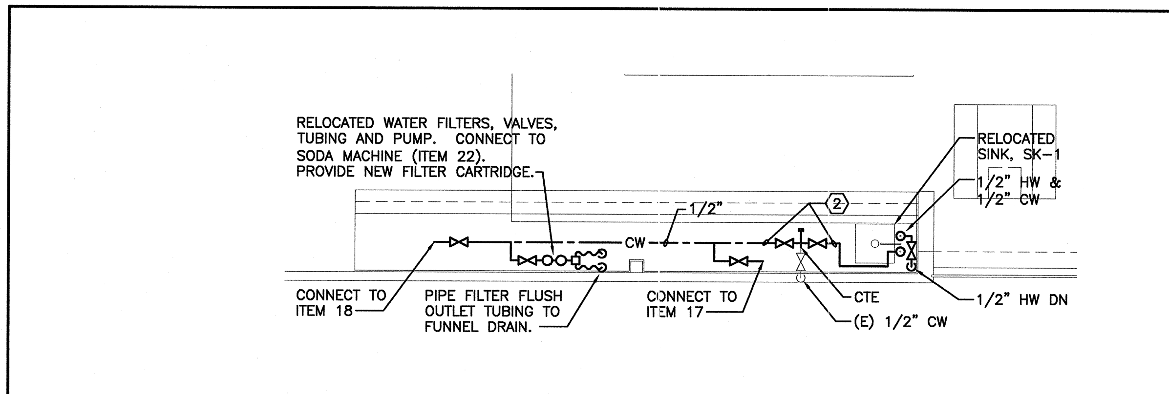
F7 BEVERAGE AREA SUPPLY PIPING PART PLAN 1/4"=1'-0"
