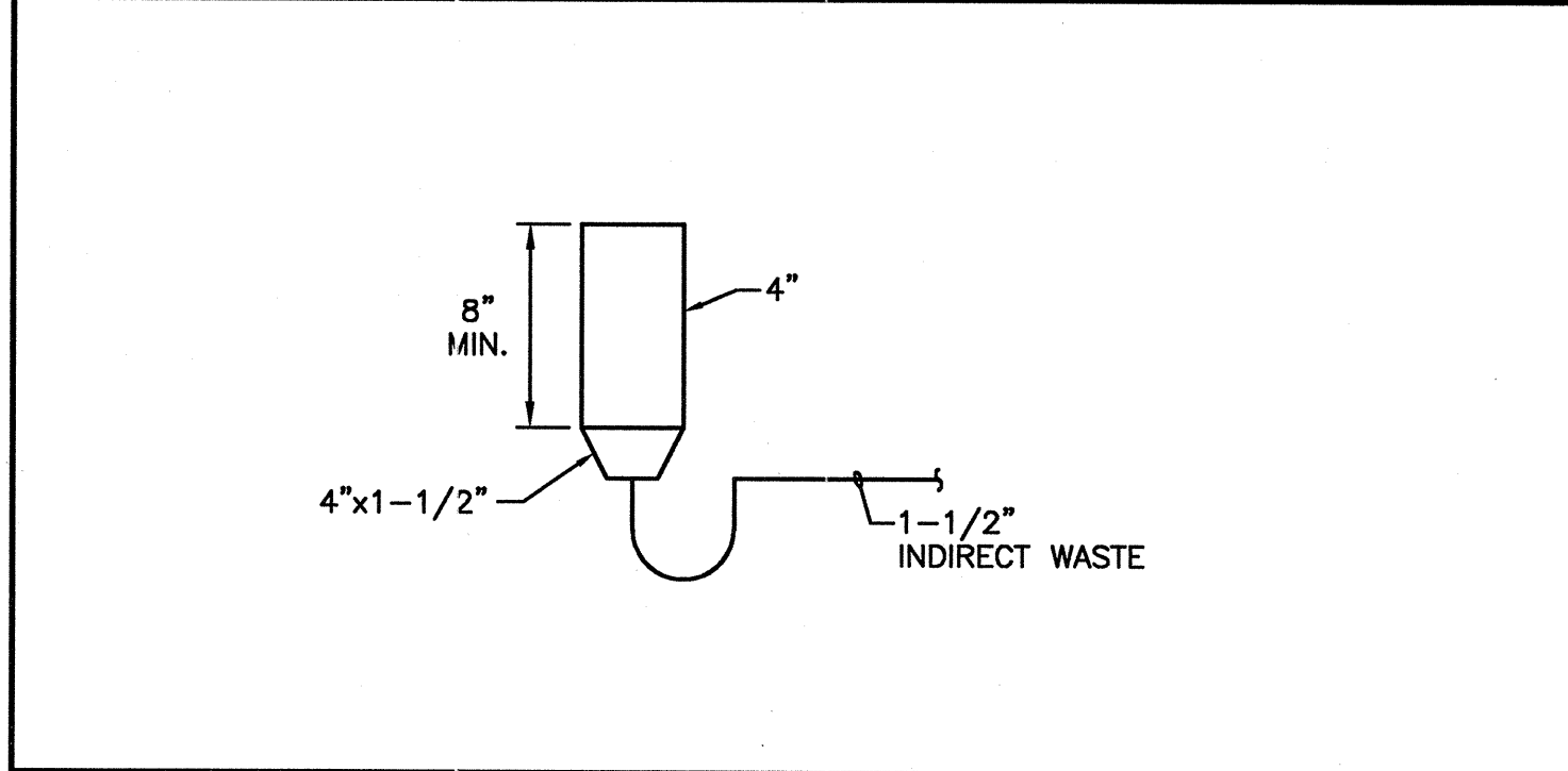
A10 FUNNEL DRAIN DETAIL NOT TO SCALE
