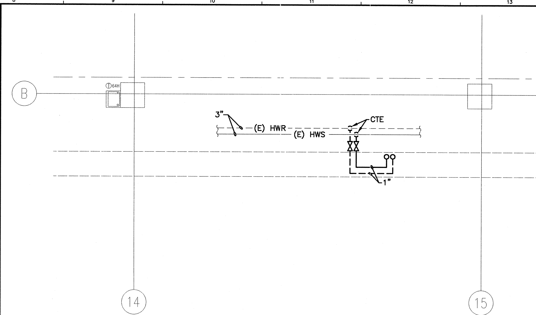
J8 GROUND LEVEL PART PLAN 1/4"=1'-0" M-401
