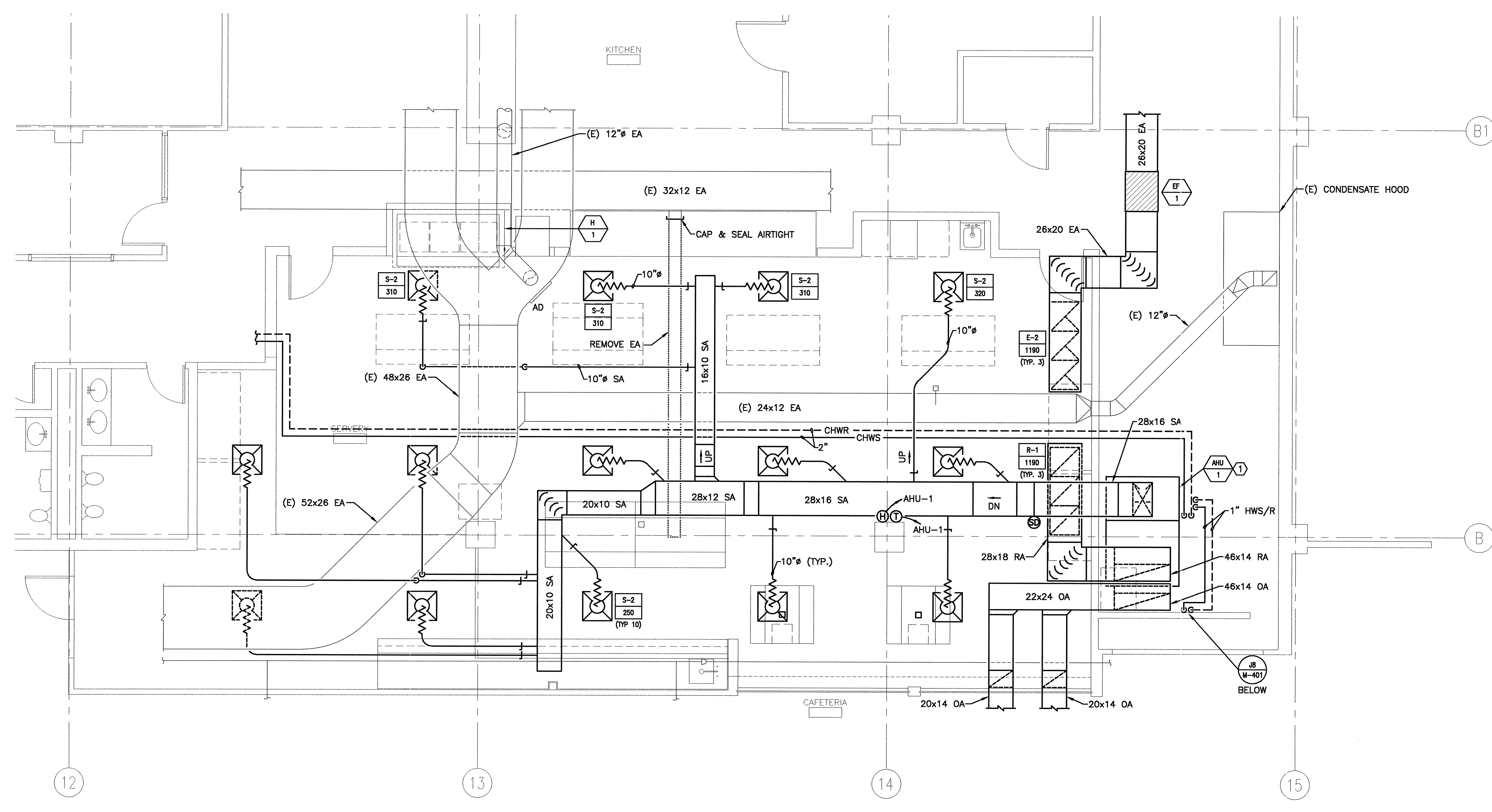
A1 SERVERY AREA HVAC PART PLAN 1/4"=1'-0" M-101
