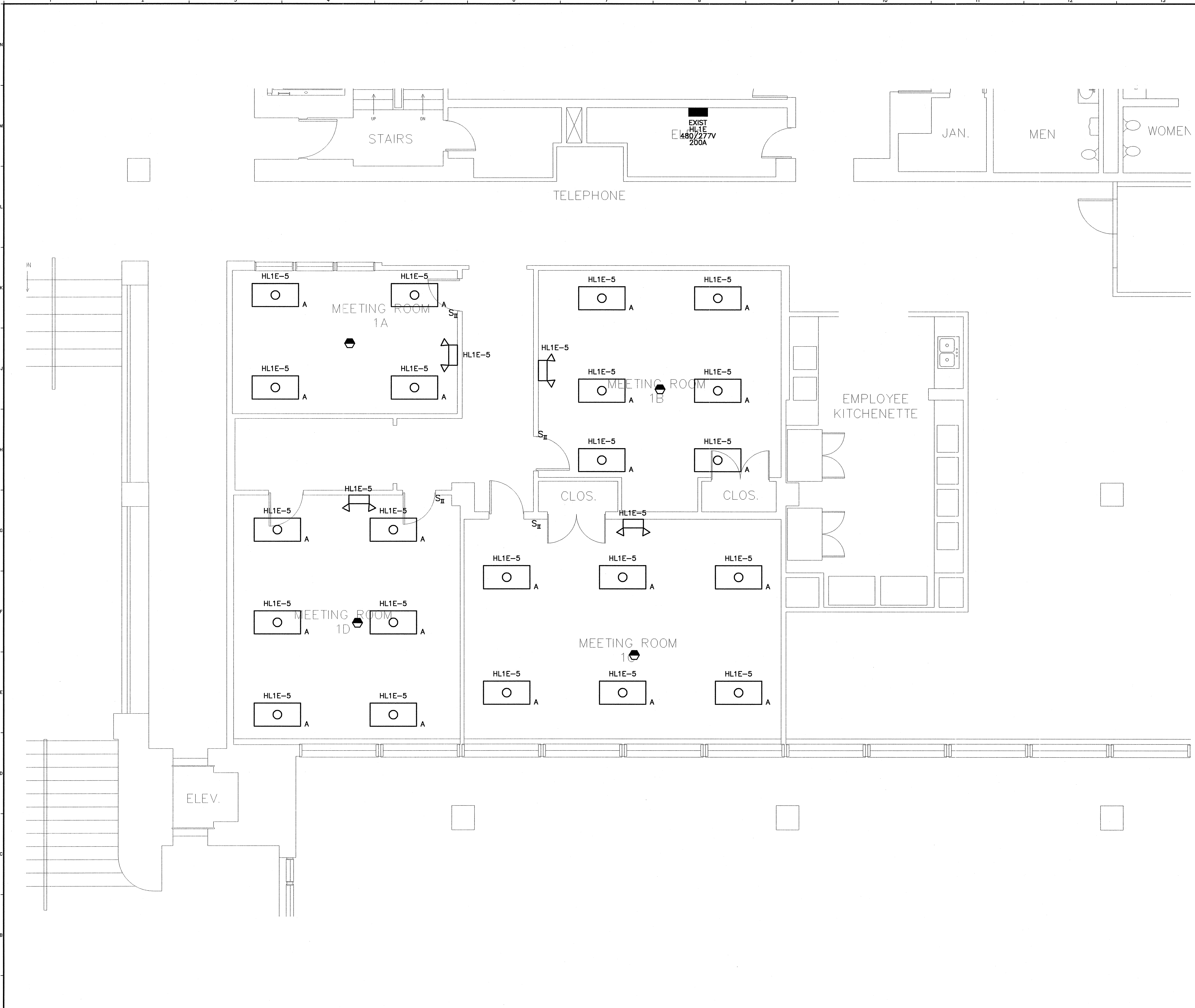
A1 I-ROOMS LIGHTING PLAN 1/4"=1'-0" *
