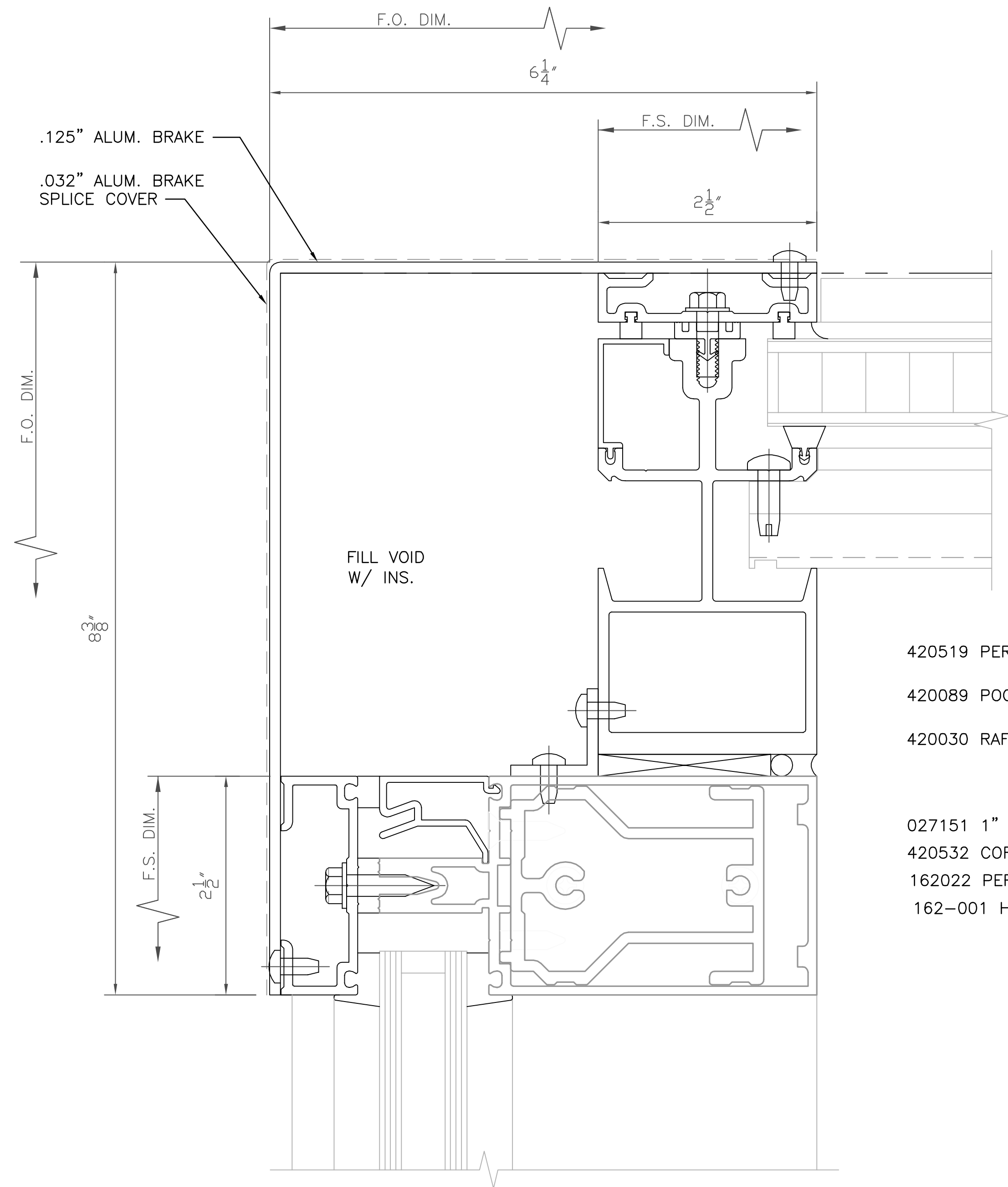
15 RAKE RAFTER DTL. FULL SCALE
