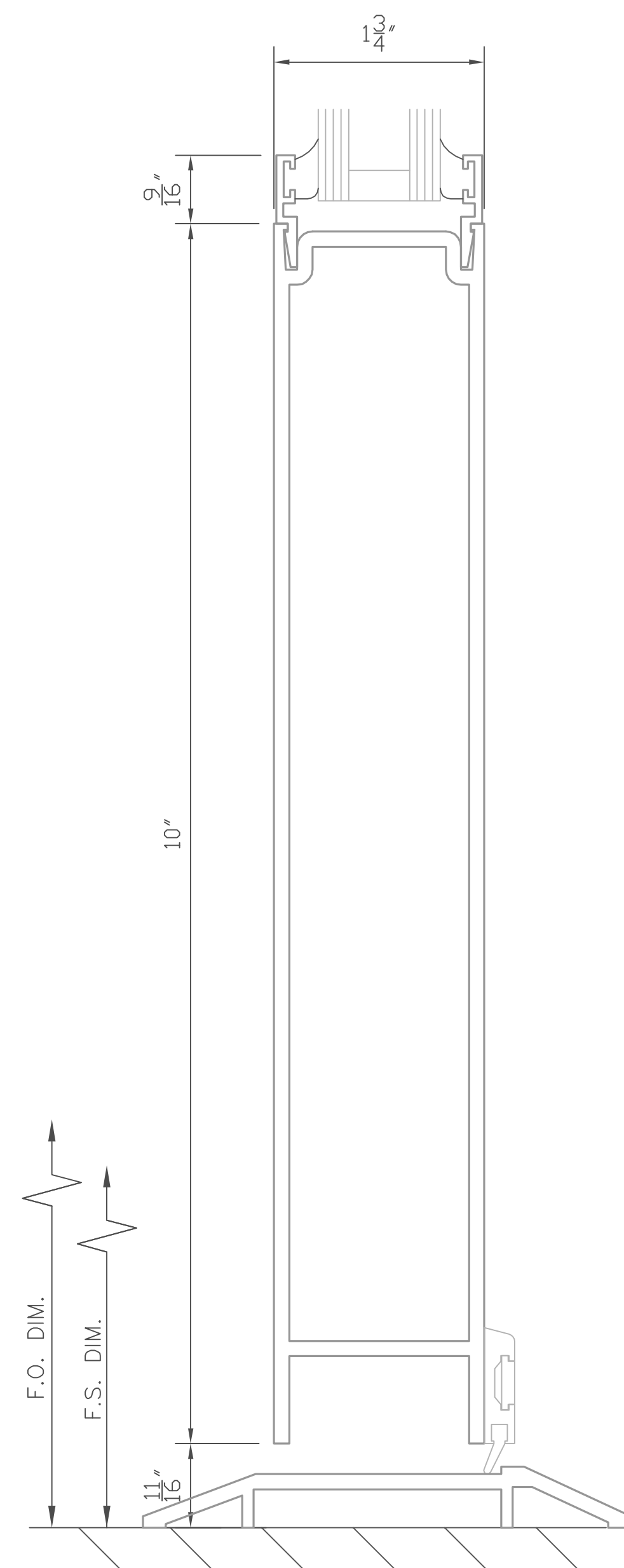
8 BOTTOM RAIL DTL. FULL SCALE
