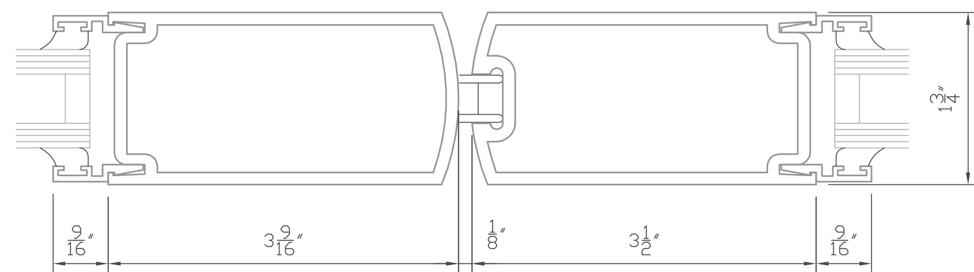
7 MEETING STILE DTL. FULL SCALE
