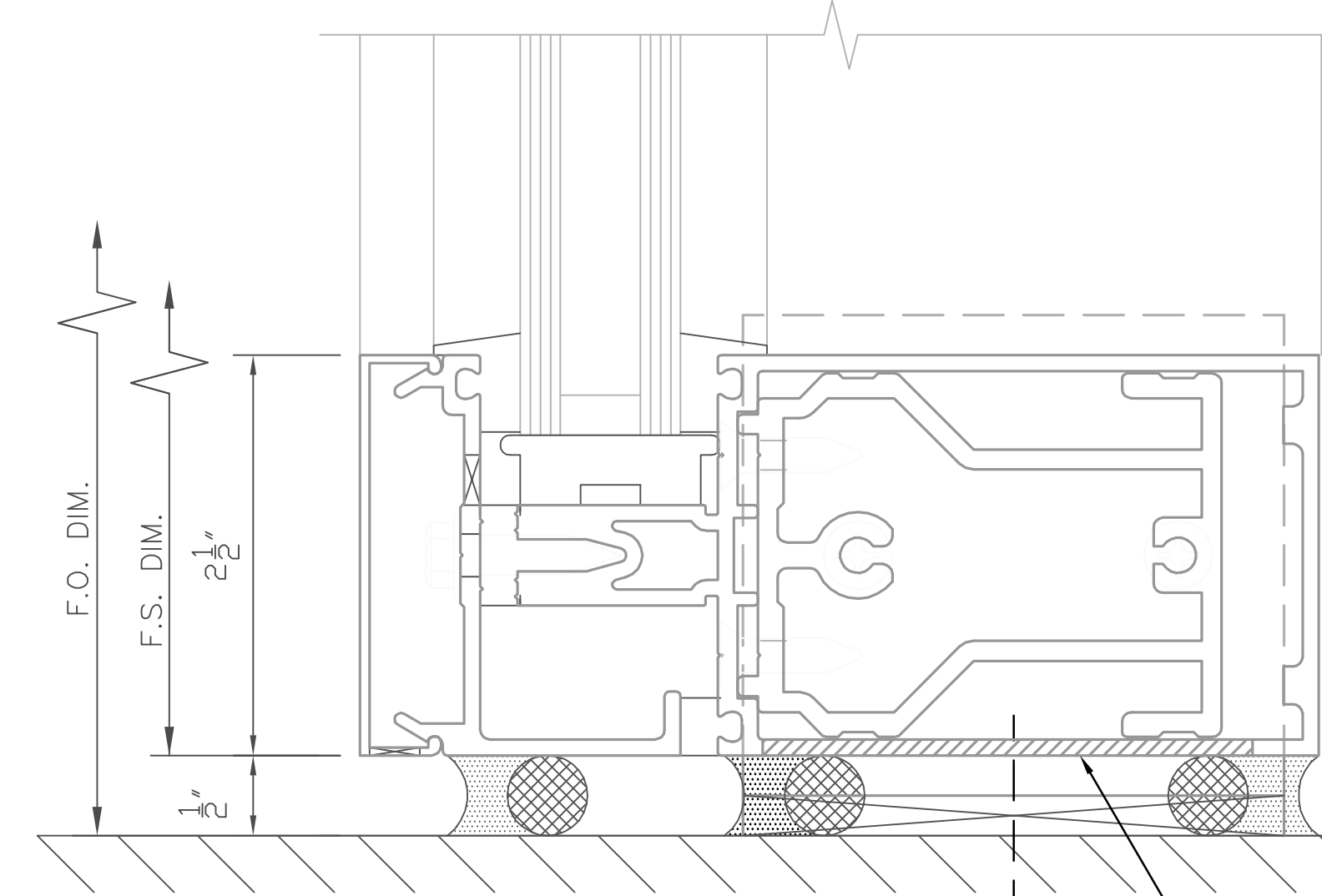
10 SILL DETAIL FULL SCALE
