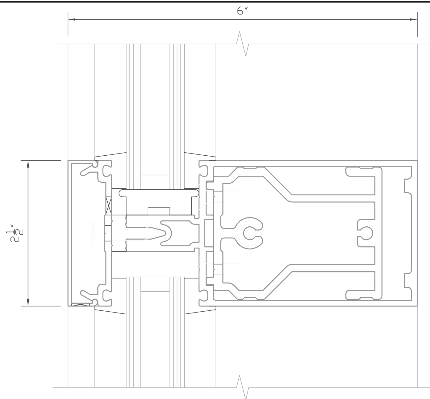
2 HORIZ. MULL. DTL. FULL SCALE
