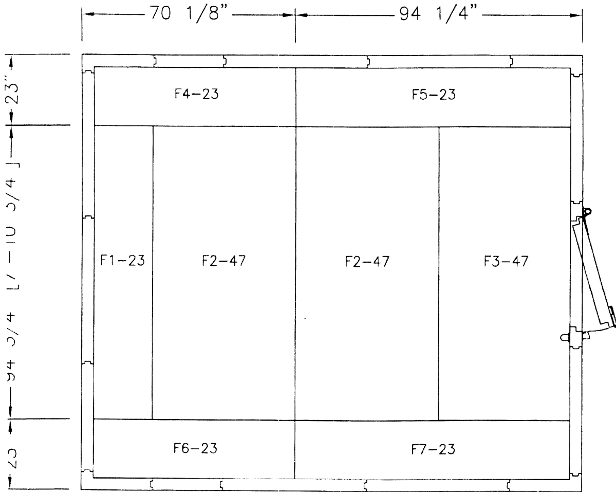
FLOOR LAYOUT
