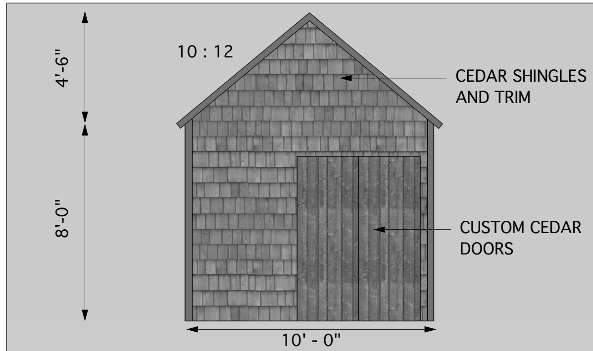
PROPOSED SHED: FRONT ELEVATION
