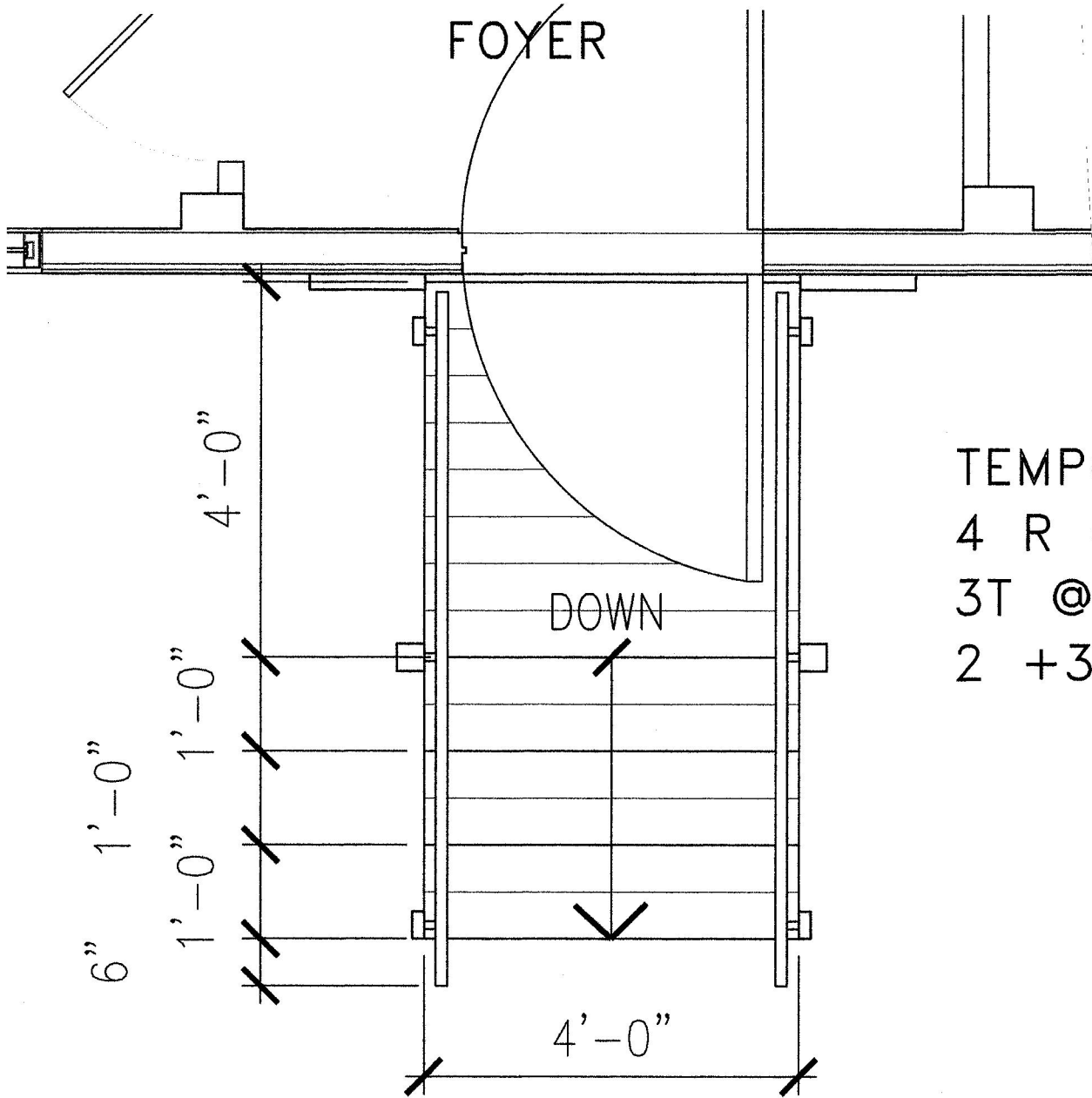
Temporary Stair Plan 1/2" = 1'-0" 8.5x11 output
