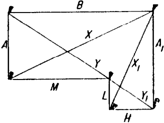
1C — TRUE "L" STAKEOUT
