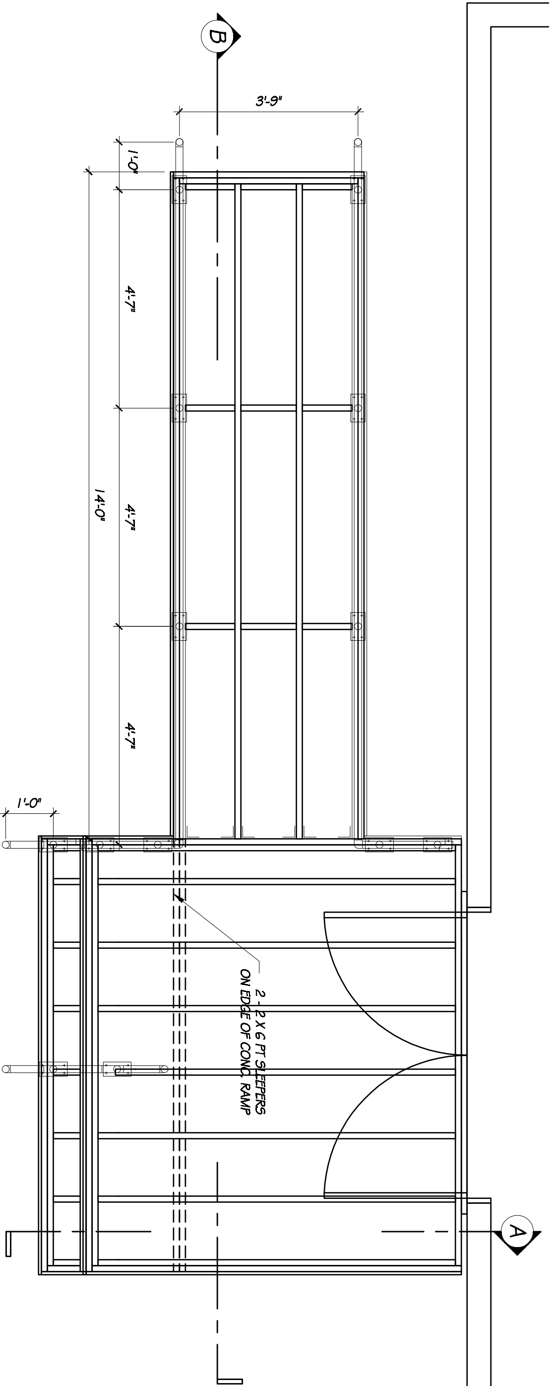
HANDRAIL LAYOUT PLAN \frac{1}{2}'' = 1'-0''
