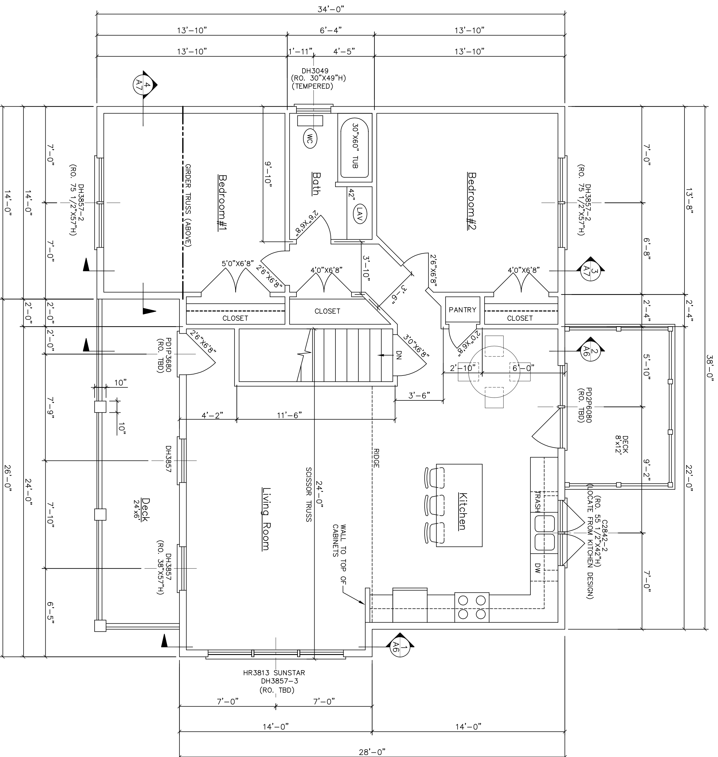
FLOOR PLAN—SECOND FLOOR
