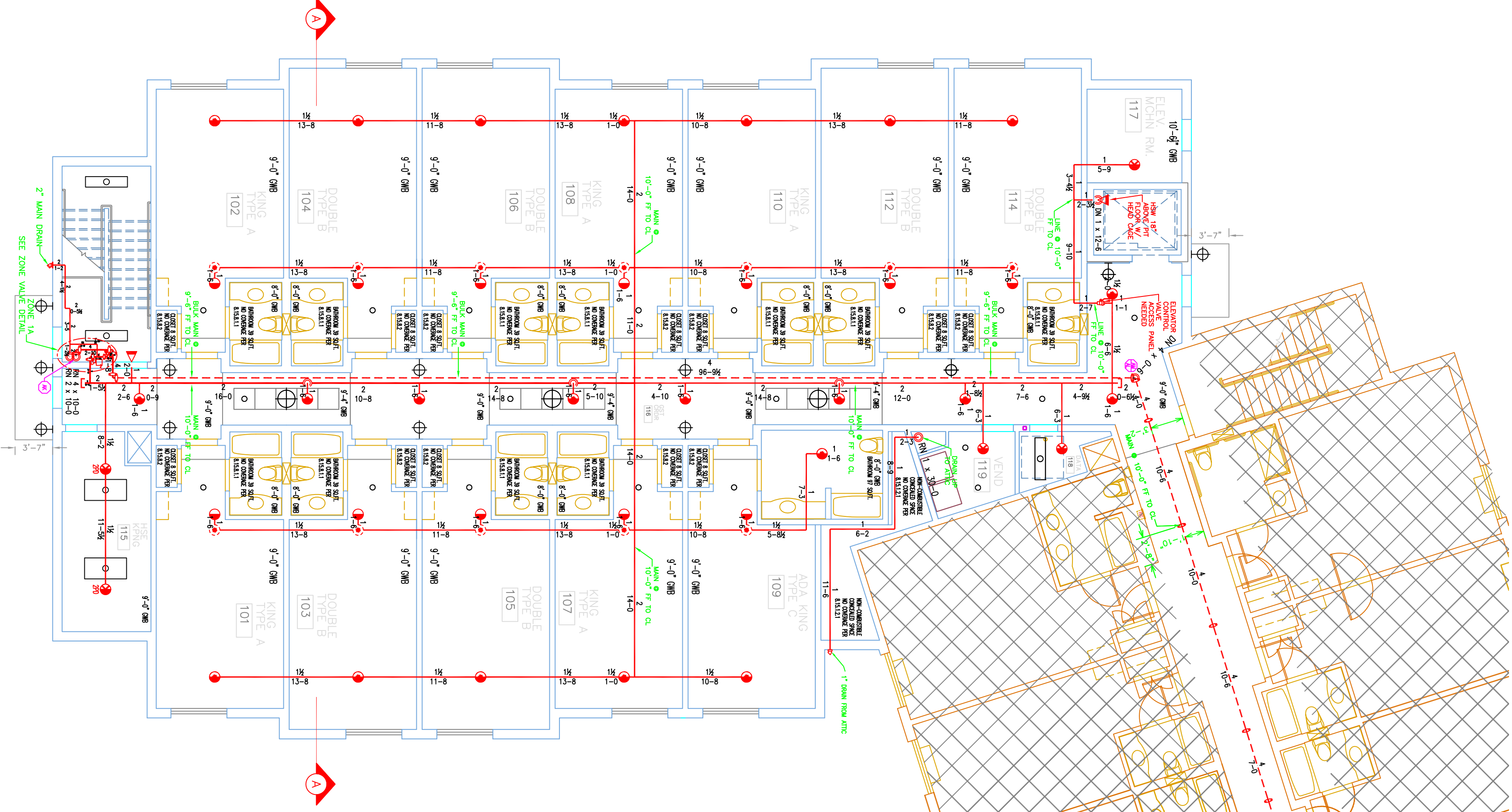
1 GROUND FLOOR (WET) SCALE 1/8" = 1'-0" TOTAL PROTECTED AREA 5,700 SQ.FT.
